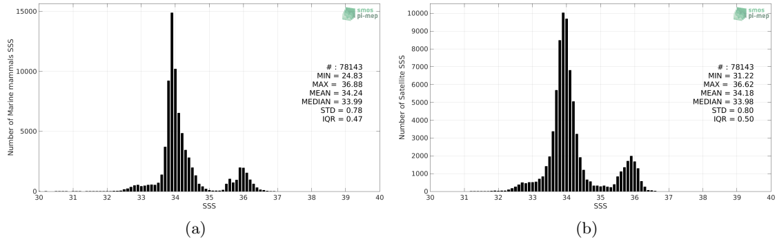
Figure 2: Histograms of SSS from Marine mammals (a) and SMOS and SMAP SSS L4 OI v1 - 7 Days (LOPS) (b) considering all match-up pairs per bins of 0.1 over the Global Ocean Pi-MEP region and for the full satellite product period.
