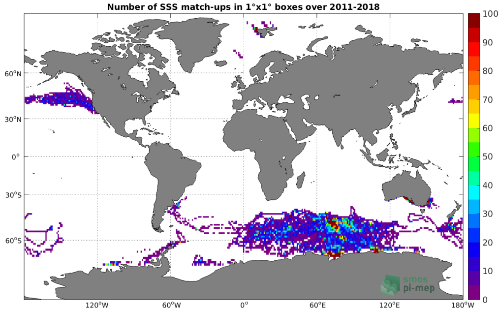
Figure 4: Number of SSS match-ups between Marine mammals SSS and the SMOS and SMAP SSS L4 OI v1 - 7 Days (LOPS) SSS product for the Global Ocean Pi-MEP region over 1°x1° boxes and for the full satellite product period.
