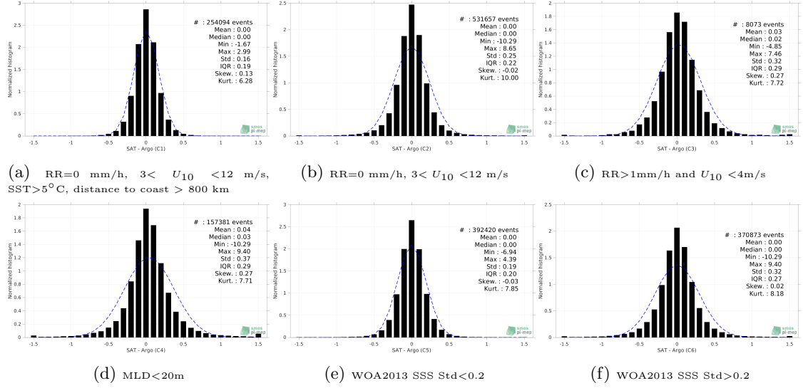
Figure 13: Normalized histogram of \Delta SSS (SMOS and SMAP SSS L4 OI v1 - 7 Days (LOPS) - Argo) for 6 different subdatasets corresponding to: RR=0 mm/h, 3 < U_{10} < 12 m/s, SST > 5°C, distance to coast > 800 km (a), RR=0 mm/h, 3 < U_{10} < 12 m/s (b), RR > 1mm/h and U_{10} < 4 m/s (c), MLD < 20m (d), WOA2013 SSS Std < 0.2 (e), WOA2013 SSS Std > 0.2 (f).
