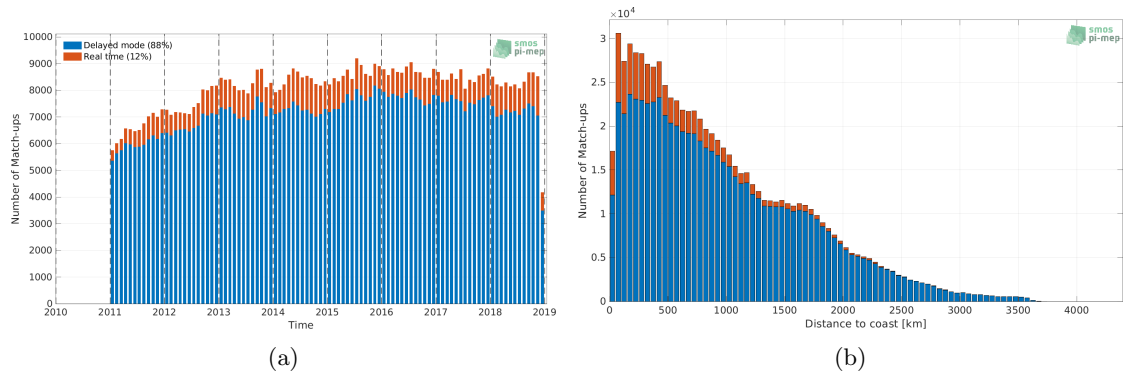
Figure 1: Number of match-ups between Argo and SMOS and SMAP SSS L4 OI v1 - 7 Days (LOPS) SSS as a function of time (a) and as function of the distance to coast (b) over the Global Ocean Pi-MEP region and for the full satellite product period.
