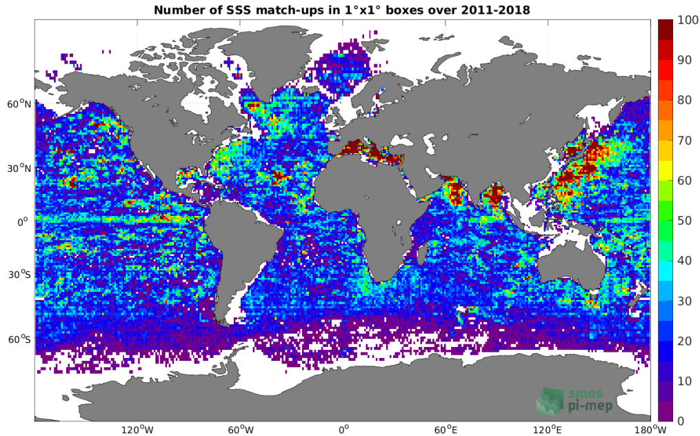
Figure 4: Number of SSS match-ups between Argo SSS and the SMOS and SMAP SSS L4 OI v1 - 7 Days (LOPS) SSS product for the Global Ocean Pi-MEP region over 1^\circ \times 1^\circ boxes and for the full satellite product period.
