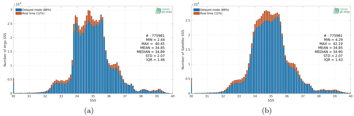
Figure 2: Histograms of SSS from Argo (a) and SMOS and SMAP SSS L4 OI v1 - 7 Days (LOPS) (b) considering all match-up pairs per bins of 0.1 over the Global Ocean Pi-MEP region and for the full satellite product period.
