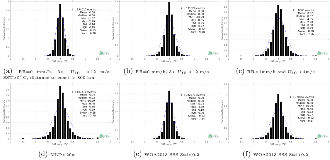
Figure 13: Normalized histogram of \Delta\text{SSS} (SMOS and SMAP SSS L4 OI v1 - 7 Days (LOPS) - Argo) for 6 different subdatasets corresponding to: RR=0 mm/h, 3 < U_{10} < 12 m/s, SST>5°C, distance to coast > 800 km (a), RR=0 mm/h, 3 < U_{10} < 12 m/s (b), RR>1mm/h and U_{10} < 4 m/s (c), MLD<20m (d), WOA2013 SSS Std<0.2 (e), WOA2013 SSS Std>0.2 (f).
