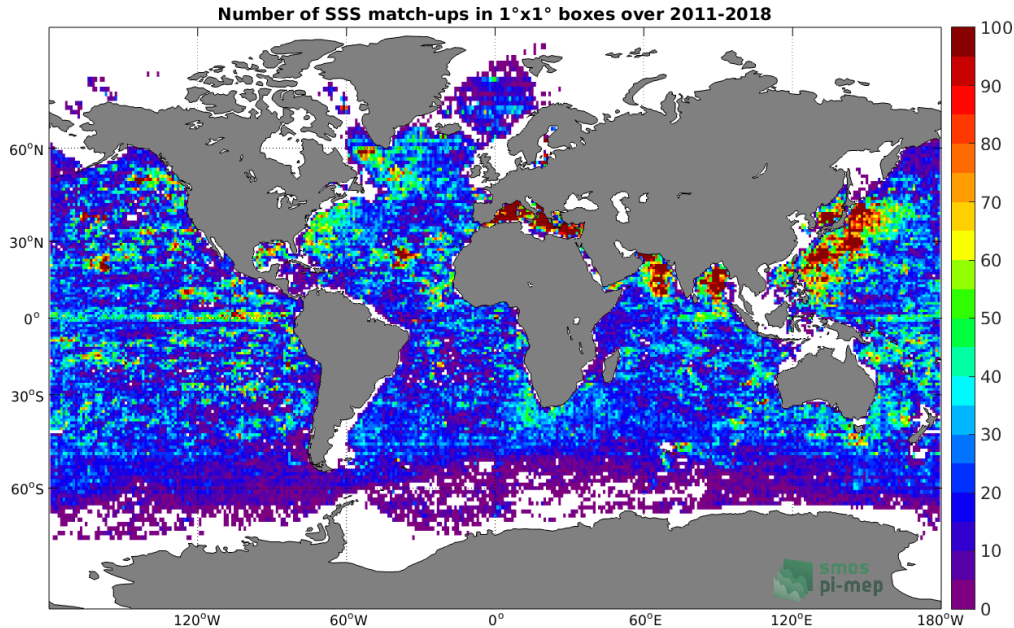
Figure 4: Number of SSS match-ups between Argo SSS and the SMOS and SMAP SSS L4 OI v1 - 7 Days (LOPS) SSS product for the Global Ocean Pi-MEP region over 1^\circ \times 1^\circ boxes and for the full satellite product period.
