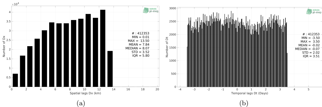
Figure 5: Histograms of the spatial (a) and temporal (b) lags between the location/time of the TSG (Polarstern) measurement and the date of the corresponding SMOS SSS L4 v1 - Weekly (CMEMS-CNR) SSS pixel.
