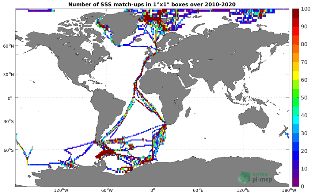
Figure 4: Number of SSS match-ups between TSG (Polarstern) SSS and the SMOS SSS L4 v1 - Weekly (CMEMS-CNR) SSS product for the Global Ocean Pi-MEP region over 1^\circ \times 1^\circ boxes and for the full satellite product period.
