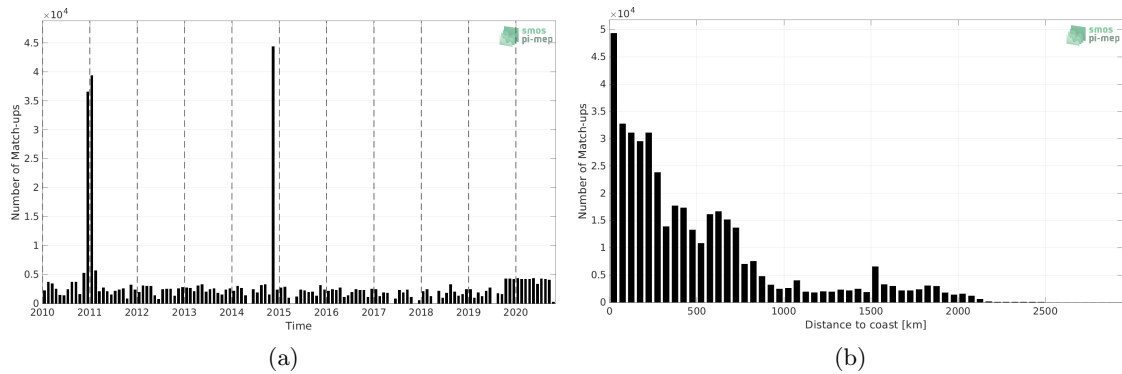
Figure 1: Number of match-ups between TSG (Polarstern) and SMOS SSS L4 v1 - Weekly (CMEMS-CNR) SSS as a function of time (a) and as function of the distance to coast (b) over the Global Ocean Pi-MEP region and for the full satellite product period.
