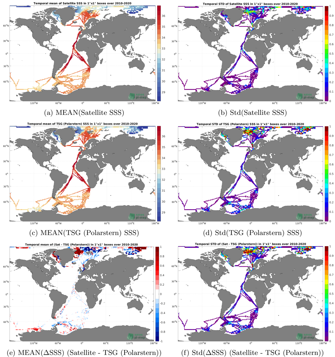
Figure 6: Temporal mean (left) and Std (right) of SSS from SMOS SSS L4 v1 - Weekly (CMEMS-CNR) (top), TSG (Polarstern) (middle), and of \Delta SSS (Satellite - TSG (Polarstern)). Only match-up pairs are used to generate these maps.
