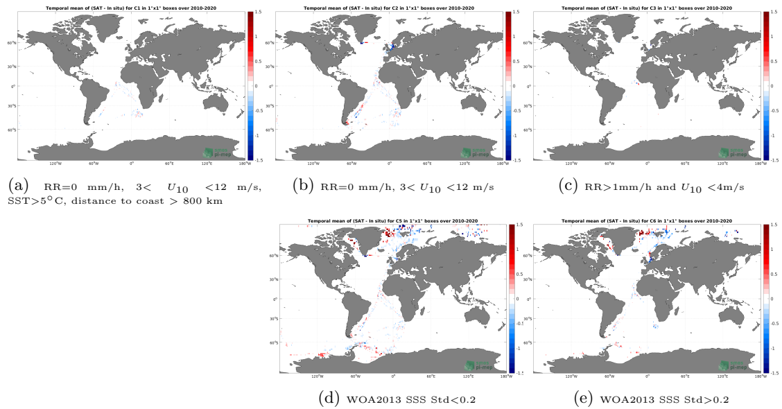
Figure 12: Temporal mean gridded over spatial boxes of size 1^\circ \times 1^\circ of \Delta SSS (SMOS SSS L4 v1 - Weekly (CMEMS-CNR) - TSG (Polarstern)) for 5 different subdatasets corresponding to:RR=0 mm/h, 3 < U_{10} < 12 m/s, SST > 5^\circ\text{C} , distance to coast > 800 km (a), RR=0 mm/h, 3 < U_{10} < 12 m/s (b), RR > 1 mm/h and U_{10} < 4 m/s (c), WOA2013 SSS Std < 0.2 (d), WOA2013 SSS Std > 0.2 (e).
