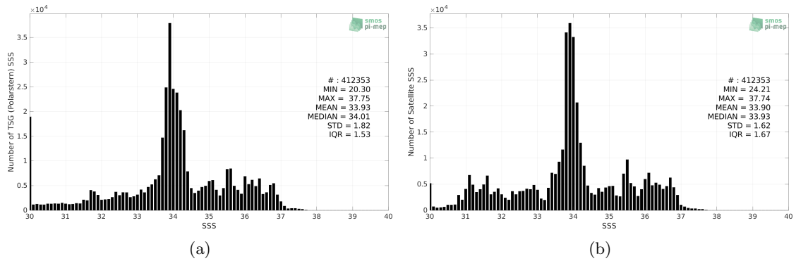
Figure 2: Histograms of SSS from TSG (Polarstern) (a) and SMOS SSS L4 v1 - Weekly (CMEMS-CNR) (b) considering all match-up pairs per bins of 0.1 over the Global Ocean Pi-MEP region and for the full satellite product period.
