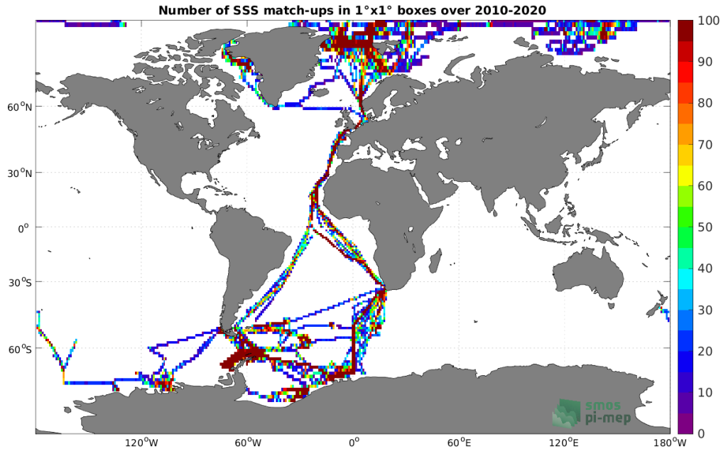
Figure 4: Number of SSS match-ups between TSG (Polarstern) SSS and the SMOS SSS L4 v1 - Weekly (CMEMS-CNR) SSS product for the Global Ocean Pi-MEP region over 1°x1° boxes and for the full satellite product period.
