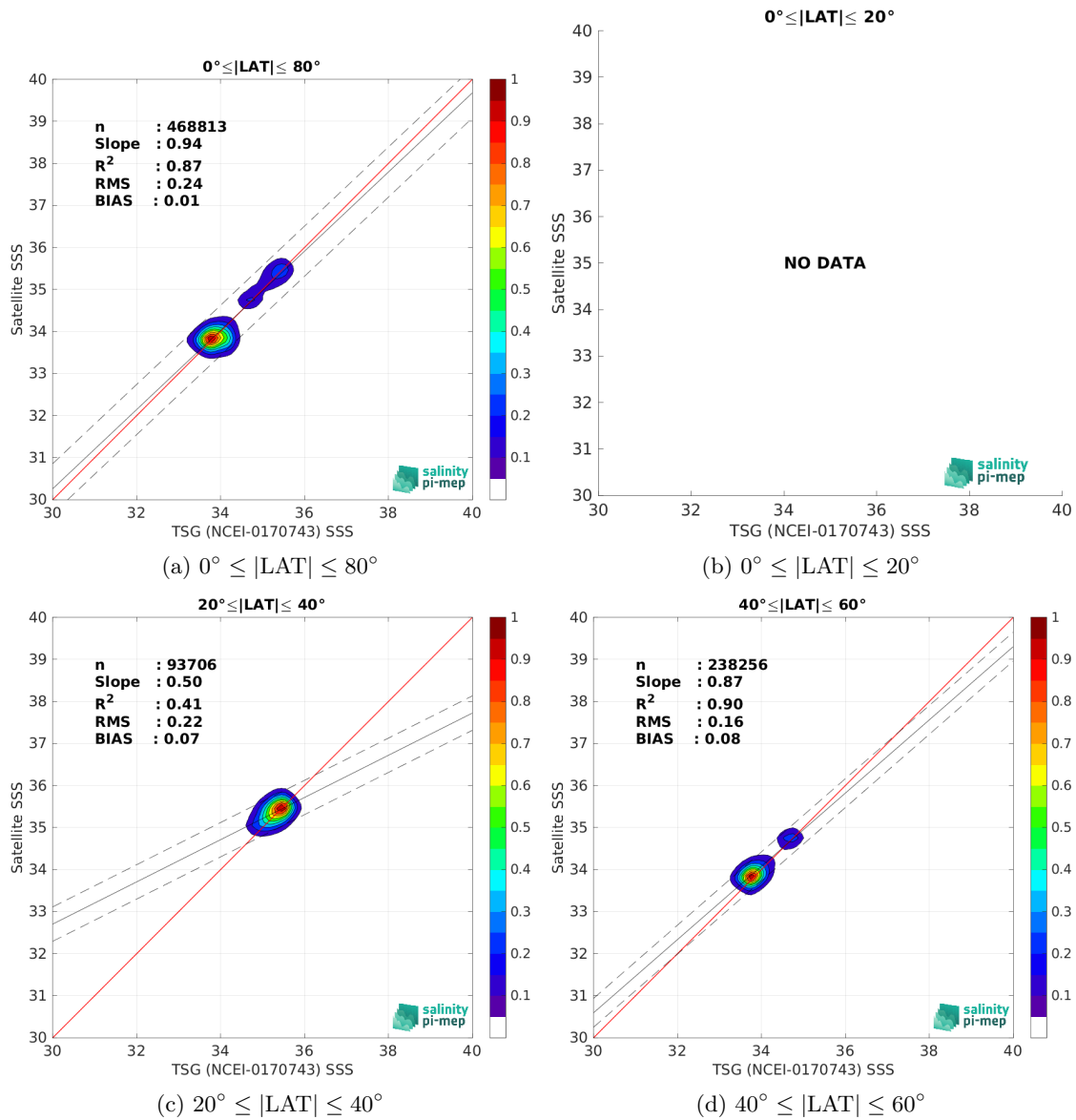
Figure 9: Contour maps of the concentration of SMOS SSS L4 v1 - Weekly (CMEMS-CNR) SSS (y-axis) versus TSG (NCEI-0170743) SSS (x-axis) at match-up pairs for different latitude bands. For each plot, the red line shows x=y . The black thin and dashed lines indicate a linear fit through the data cloud and the \pm 95\% confidence levels, respectively. The number match-up pairs n , the slope and R^2 coefficient of the linear fit, the root mean square (RMS) and the mean bias between satellite and in situ data are indicated for each latitude band in each plots.
