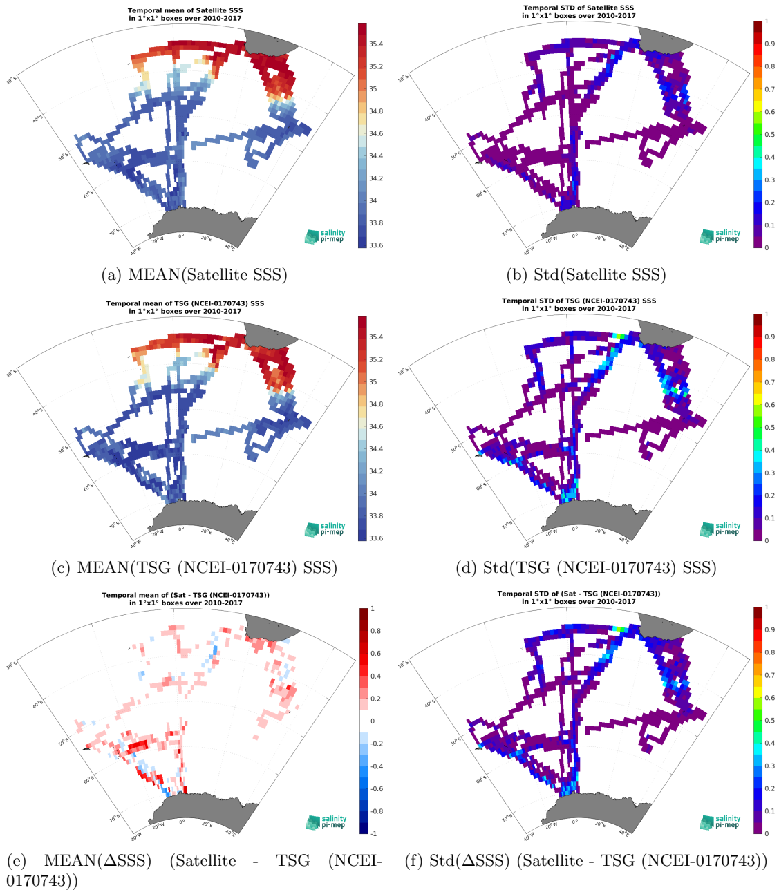
Figure 6: Temporal mean (left) and Std (right) of SSS from SMOS SSS L4 v1 - Weekly (CMEMS-CNR) (top), TSG (NCEI-0170743) (middle), and of \Delta SSS (Satellite - TSG (NCEI-0170743)). Only match-up pairs are used to generate these maps.
