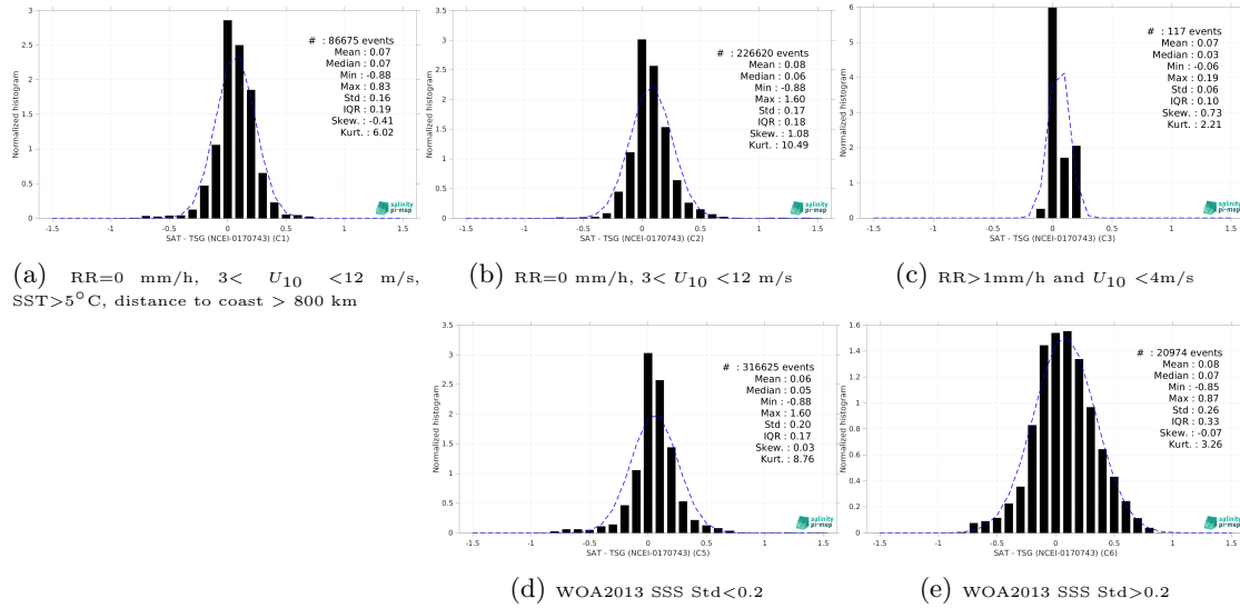
Figure 13: Normalized histogram of \Delta SSS (SMOS SSS L4 v1 - Weekly (CMEMS-CNR) - TSG (NCEI-0170743)) for 5 different subdatasets corresponding to: RR=0 mm/h, 3 < U_{10} < 12 m/s, SST>5°C, distance to coast > 800 km (a), RR=0 mm/h, 3 < U_{10} < 12 m/s (b), RR>1mm/h and U_{10} < 4 m/s (c), WOA2013 SSS Std<0.2 (d), WOA2013 SSS Std>0.2 (e).
