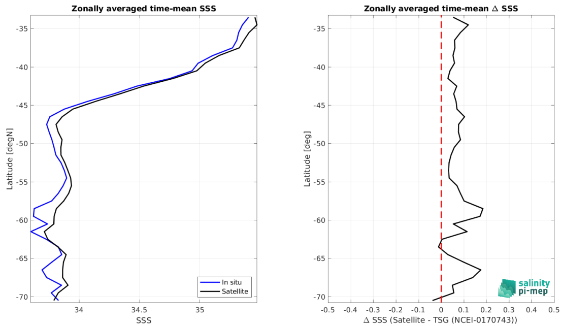
Figure 8: Left panel: Zonal mean SSS from SMOS SSS L4 v1 - Weekly (CMEMS-CNR) satellite product (black) and from TSG (NCEI-0170743) (blue). Right panel: Zonal mean of \Delta SSS (Satellite - TSG (NCEI-0170743)) for all the collected Pi-MEP match-up pairs estimated over the full satellite product period.
