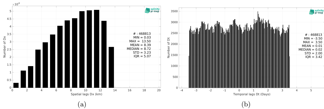
Figure 5: Histograms of the spatial (a) and temporal (b) lags between the location/time of the TSG (NCEI-0170743) measurement and the date of the corresponding SMOS SSS L4 v1 - Weekly (CMEMS-CNR) SSS pixel.
