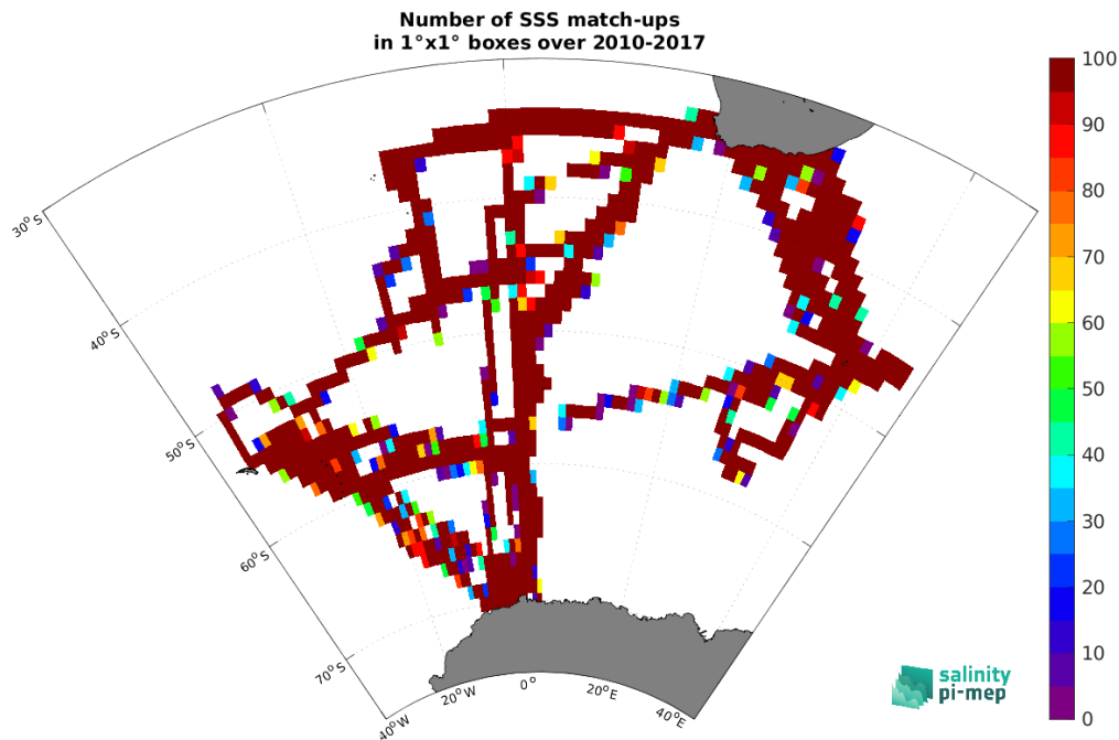
Figure 4: Number of SSS match-ups between TSG (NCEI-0170743) SSS and the SMOS SSS L4 v1 - Weekly (CMEMS-CNR) SSS product for the Global Ocean Pi-MEP region over 1^\circ \times 1^\circ boxes and for the full satellite product period.
