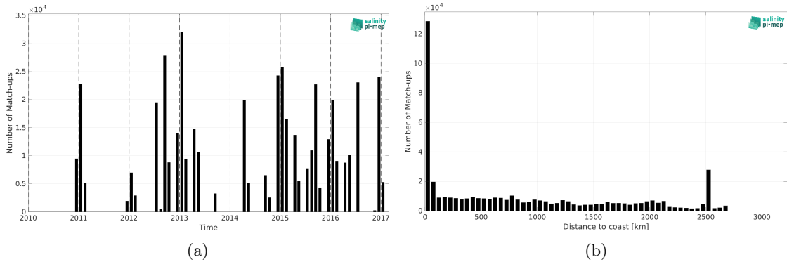
Figure 1: Number of match-ups between TSG (NCEI-0170743) and SMOS SSS L4 v1 - Weekly (CMEMS-CNR) SSS as a function of time (a) and as function of the distance to coast (b) over the Global Ocean Pi-MEP region and for the full satellite product period.
