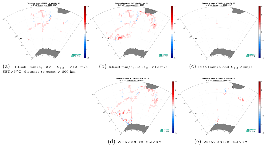
Figure 12: Temporal mean gridded over spatial boxes of size 1^\circ \times 1^\circ of \Delta SSS (SMOS SSS L4 v1 - Weekly (CMEMS-CNR) - TSG (NCEI-0170743)) for 5 different subdatasets corresponding to:RR=0 mm/h, 3 < U_{10} < 12 m/s, SST >5^\circ C, distance to coast > 800 km (a), RR=0 mm/h, 3 < U_{10} < 12 m/s (b), RR >1 mm/h and U_{10} < 4 m/s (c), WOA2013 SSS Std <0.2 (d), WOA2013 SSS Std >0.2 (e).
