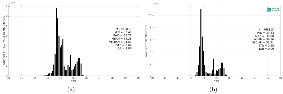
Figure 2: Histograms of SSS from TSG (NCEI-0170743) (a) and SMOS SSS L4 v1 - Weekly (CMEMS-CNR) (b) considering all match-up pairs per bins of 0.1 over the Global Ocean Pi-MEP region and for the full satellite product period.
