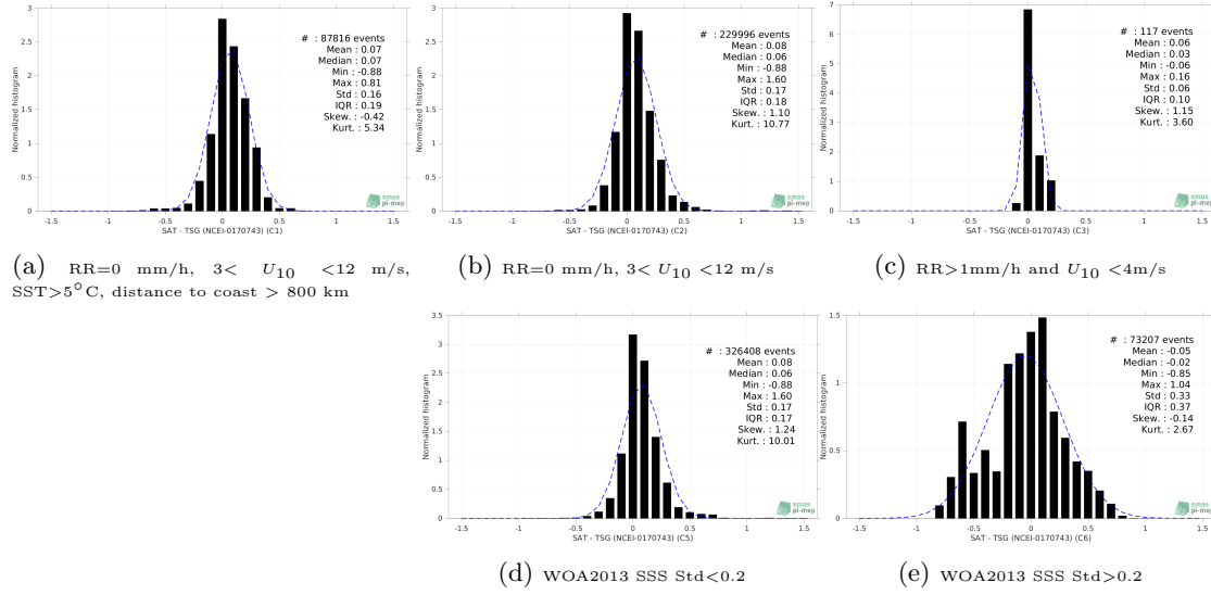
Figure 13: Normalized histogram of \Delta SSS (SMOS SSS L4 v1 - Weekly (CMEMS-CNR) - TSG (NCEI-0170743)) for 5 different subdatasets corresponding to: RR=0 mm/h, 3 < U_{10} < 12 m/s, SST > 5°C, distance to coast > 800 km (a), RR=0 mm/h, 3 < U_{10} < 12 m/s (b), RR > 1mm/h and U_{10} < 4 m/s (c), WOA2013 SSS Std < 0.2 (d), WOA2013 SSS Std > 0.2 (e).
