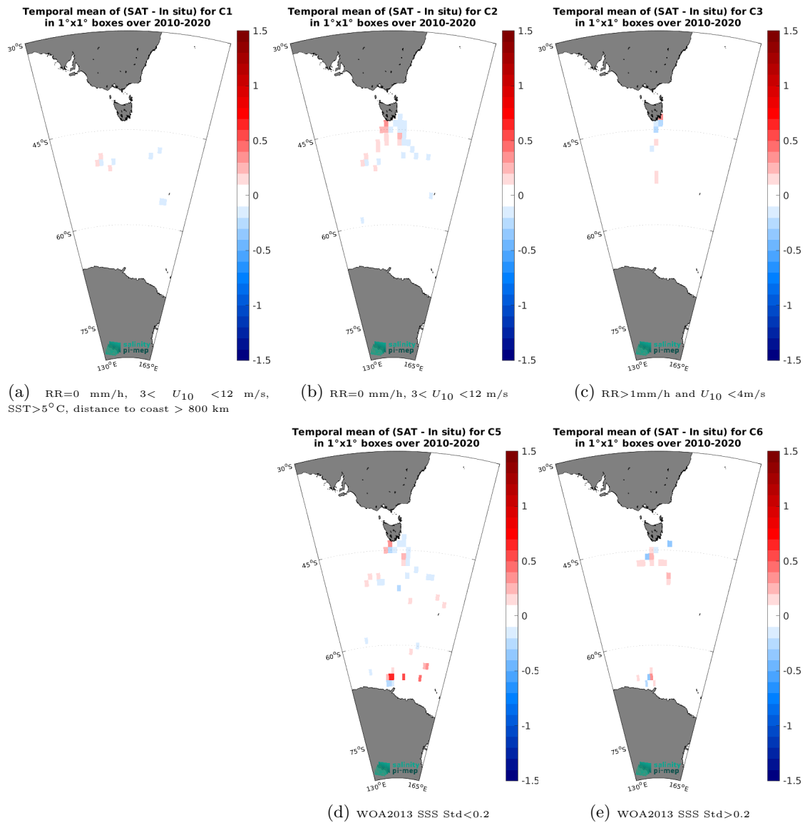
Figure 12: Temporal mean gridded over spatial boxes of size 1^\circ \times 1^\circ of \Delta SSS (SMOS SSS L4 v1 - Weekly (CMEMS-CNR) - TSG (LEGOS-Survostral)) for 5 different subdatasets corresponding to: RR=0 mm/h, 3 < U_{10} < 12 m/s, SST>5°C, distance to coast > 800 km (a), RR=0 mm/h, 3 < U_{10} < 12 m/s (b), RR>1mm/h and U_{10} < 4 m/s (c), WOA2013 SSS Std<0.2 (d), WOA2013 SSS Std>0.2 (e).
