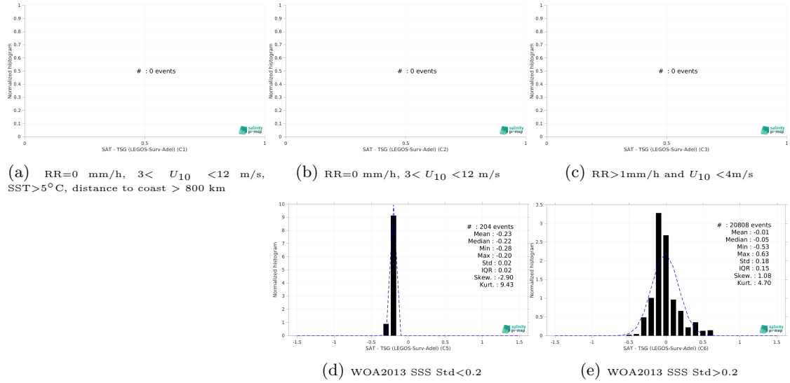
Figure 13: Normalized histogram of \Delta SSS (SMOS SSS L4 v1 - Weekly (CMEMS-CNR) - TSG (LEGOS-Surv-Adel)) for 5 different subdatasets corresponding to: RR=0 mm/h, 3 < U_{10} < 12 m/s, SST > 5°C, distance to coast > 800 km (a), RR=0 mm/h, 3 < U_{10} < 12 m/s (b), RR > 1mm/h and U_{10} < 4 m/s (c), WOA2013 SSS Std < 0.2 (d), WOA2013 SSS Std > 0.2 (e).
