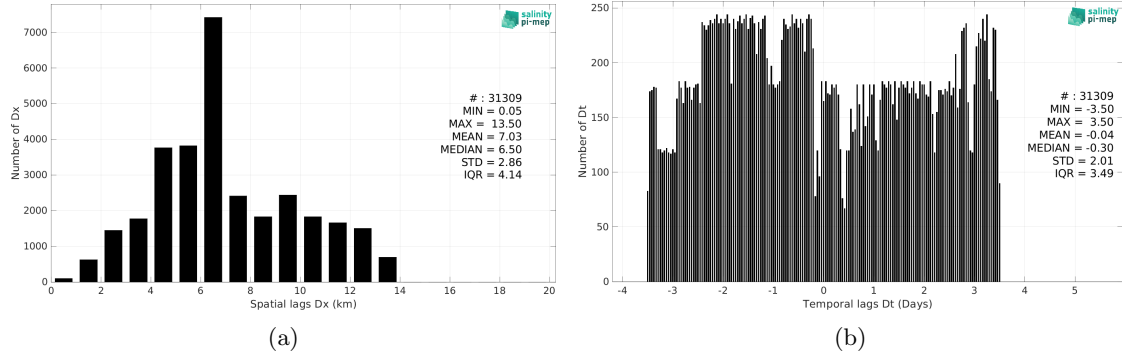
Figure 5: Histograms of the spatial (a) and temporal (b) lags between the location/time of the TSG (LEGOS-Surv-Adel) measurement and the date of the corresponding SMOS SSS L4 v1 - Weekly (CMEMS-CNR) SSS pixel.
