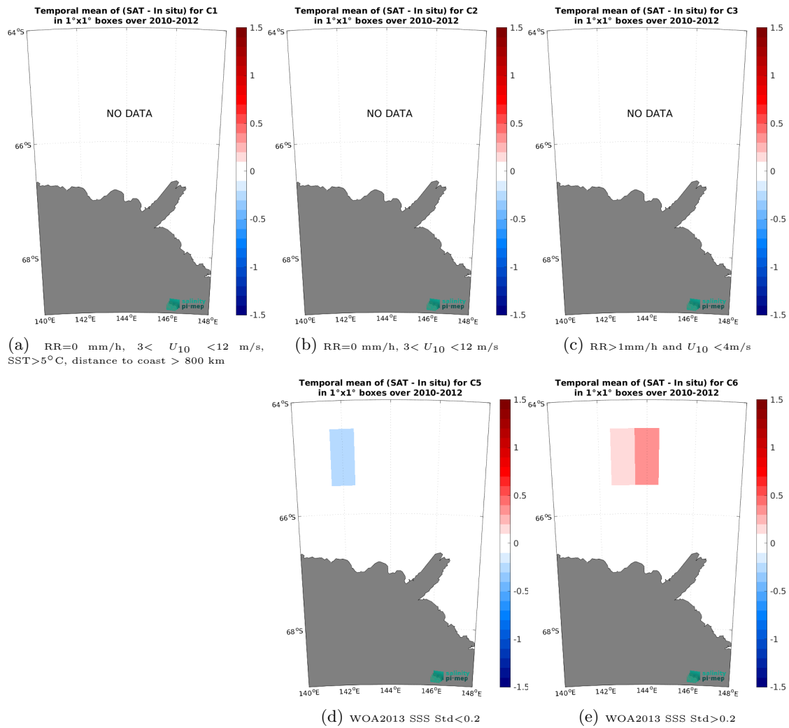
Figure 12: Temporal mean gridded over spatial boxes of size 1^\circ \times 1^\circ of \Delta SSS (SMOS SSS L4 v1 - Weekly (CMEMS-CNR) - TSG (LEGOS-Surv-Adel)) for 5 different subdatasets corresponding to: RR=0 mm/h, 3 < U_{10} < 12 m/s, SST>5°C, distance to coast > 800 km (a), RR=0 mm/h, 3 < U_{10} < 12 m/s (b), RR>1mm/h and U_{10} < 4 m/s (c), WOA2013 SSS Std<0.2 (d), WOA2013 SSS Std>0.2 (e).
