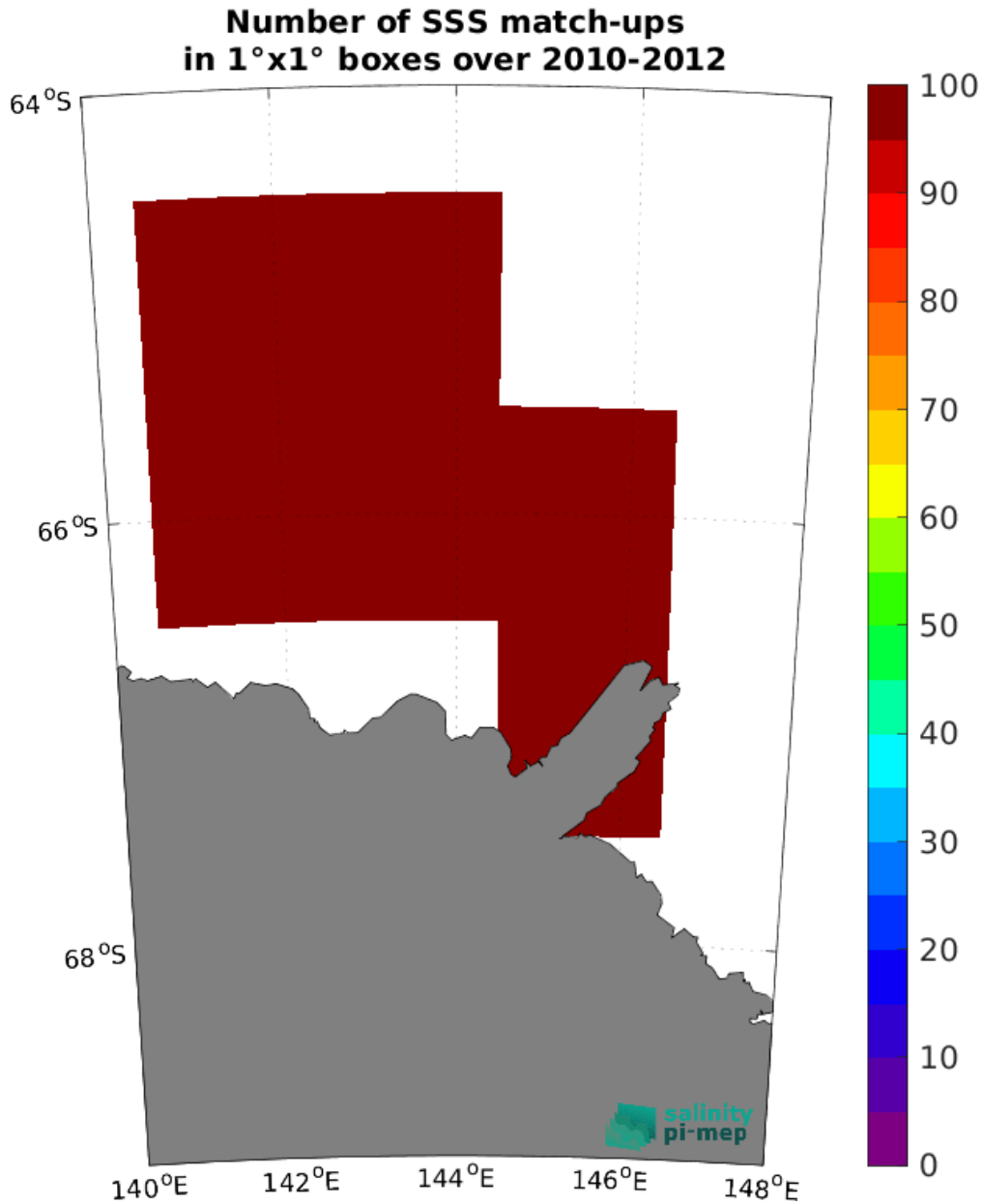
Figure 4: Number of SSS match-ups between TSG (LEGOS-Surv-Adel) SSS and the SMOS SSS L4 v1 - Weekly (CMEMS-CNR) SSS product for the Global Ocean Pi-MEP region over 1^\circ \times 1^\circ boxes and for the full satellite product period.
