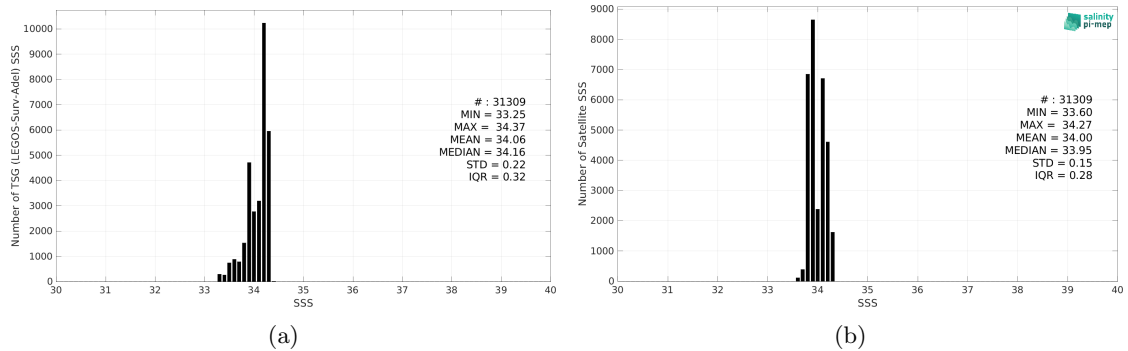
Figure 2: Histograms of SSS from TSG (LEGOS-Surv-Adel) (a) and SMOS SSS L4 v1 - Weekly (CMEMS-CNR) (b) considering all match-up pairs per bins of 0.1 over the Global Ocean Pi-MEP region and for the full satellite product period.
