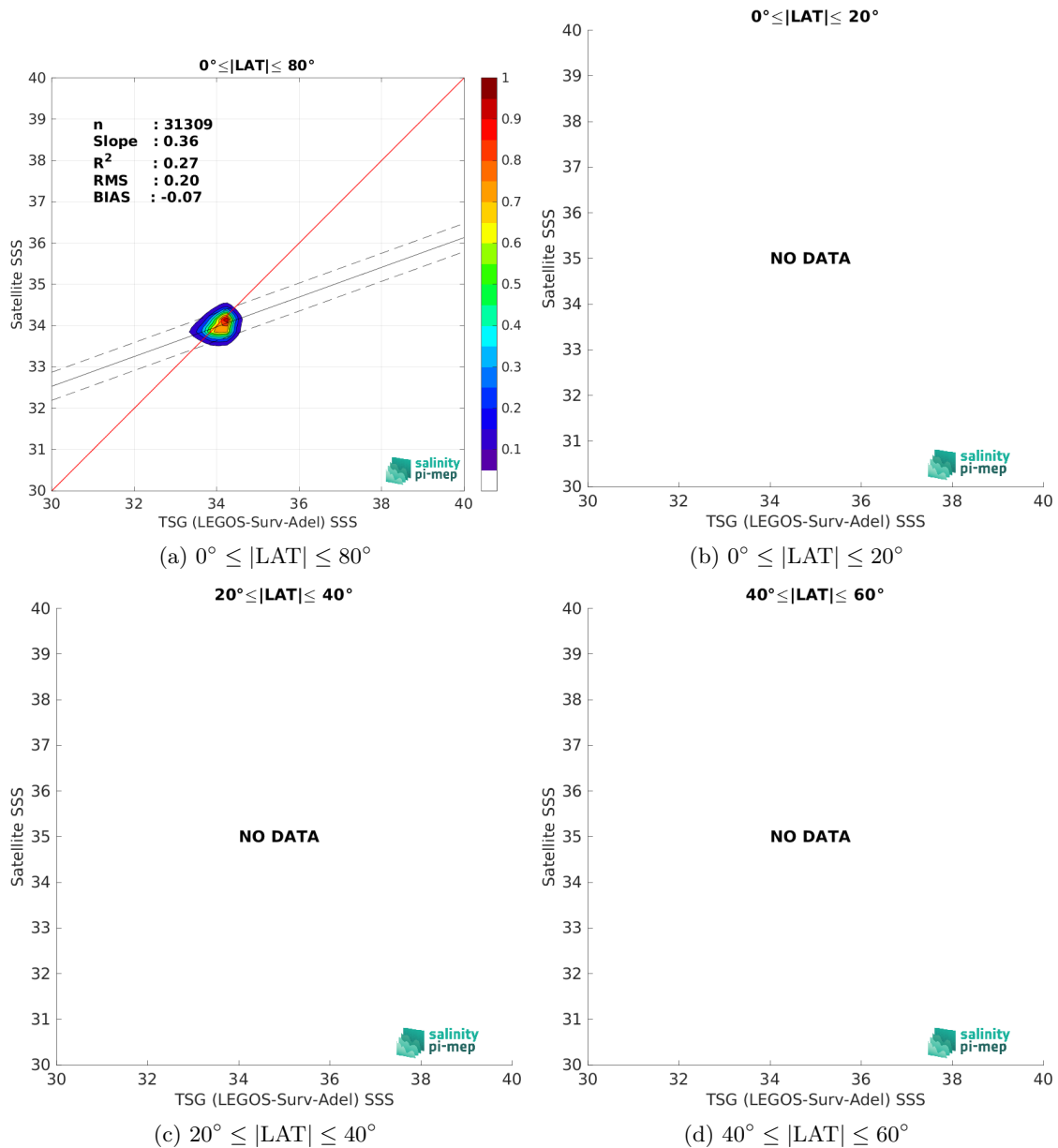
Figure 9: Contour maps of the concentration of SMOS SSS L4 v1 - Weekly (CMEMS-CNR) SSS (y-axis) versus TSG (LEGOS-Surv-Adel) SSS (x-axis) at match-up pairs for different latitude bands. For each plot, the red line shows x=y . The black thin and dashed lines indicate a linear fit through the data cloud and the \pm 95\% confidence levels, respectively. The number match-up pairs n , the slope and R^2 coefficient of the linear fit, the root mean square (RMS) and the mean bias between satellite and in situ data are indicated for each latitude band in each plots.
