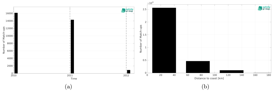
Figure 1: Number of match-ups between TSG (LEGOS-Surv-Adel) and SMOS SSS L4 v1 - Weekly (CMEMS-CNR) SSS as a function of time (a) and as function of the distance to coast (b) over the Global Ocean Pi-MEP region and for the full satellite product period.
