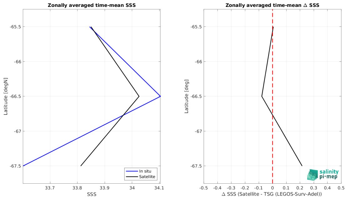
Figure 8: Left panel: Zonal mean SSS from SMOS SSS L4 v1 - Weekly (CMEMS-CNR) satellite product (black) and from TSG (LEGOS-Surv-Adel) (blue). Right panel: Zonal mean of \Delta SSS (Satellite - TSG (LEGOS-Surv-Adel)) for all the collected Pi-MEP match-up pairs estimated over the full satellite product period.
