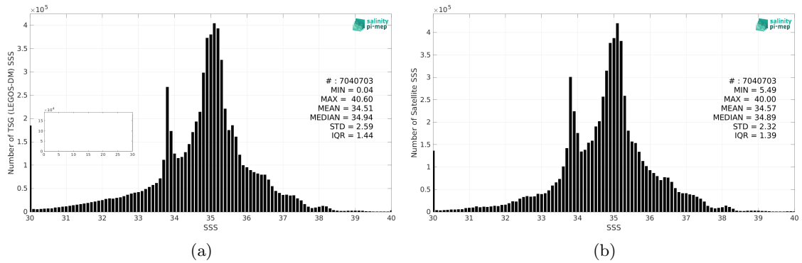
Figure 2: Histograms of SSS from TSG (LEGOS-DM) (a) and SMOS SSS L4 v1 - Weekly (CMEMS-CNR) (b) considering all match-up pairs per bins of 0.1 over the Global Ocean Pi-MEP region and for the full satellite product period.
