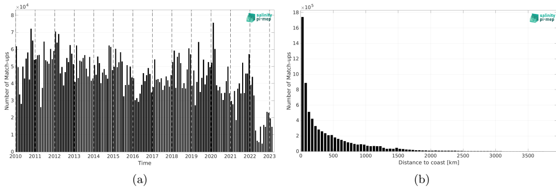
Figure 1: Number of match-ups between TSG (LEGOS-DM) and SMOS SSS L4 v1 - Weekly (CMEMS-CNR) SSS as a function of time (a) and as function of the distance to coast (b) over the Global Ocean Pi-MEP region and for the full satellite product period.
