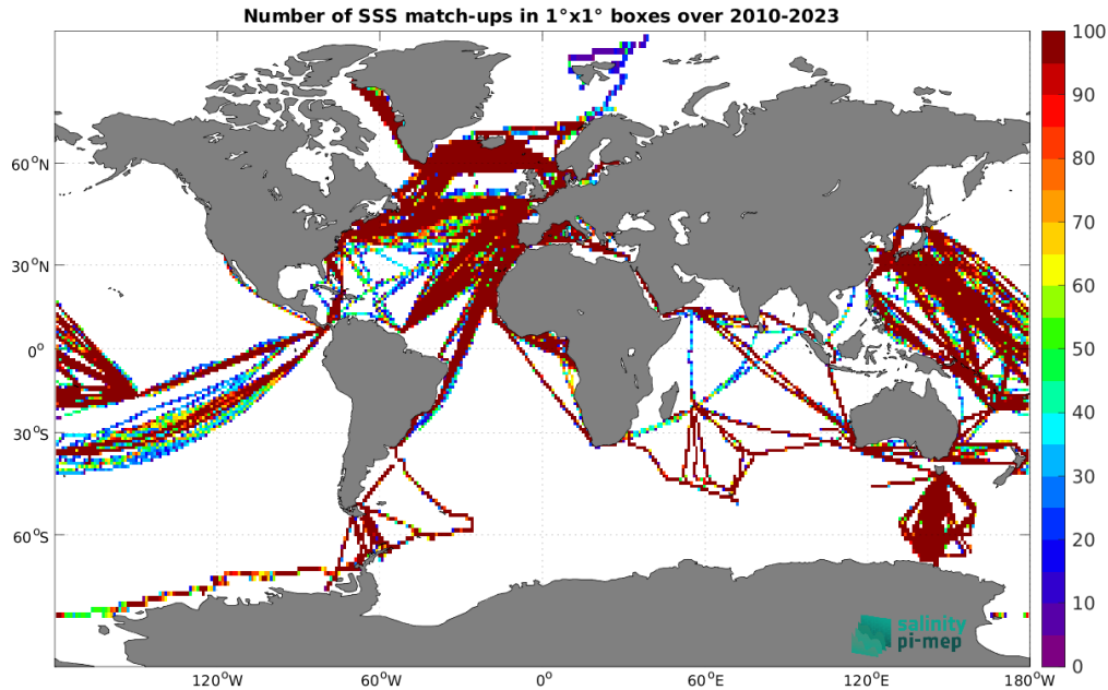
Figure 4: Number of SSS match-ups between TSG (LEGOS-DM) SSS and the SMOS SSS L4 v1 - Weekly (CMEMS-CNR) SSS product for the Global Ocean Pi-MEP region over 1^\circ \times 1^\circ boxes and for the full satellite product period.
