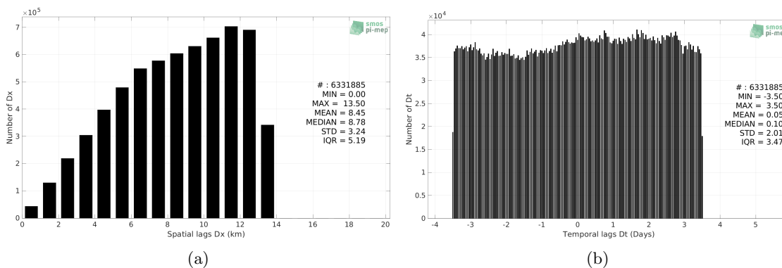
Figure 5: Histograms of the spatial (a) and temporal (b) lags between the location/time of the TSG (LEGOS-DM) measurement and the date of the corresponding SMOS SSS L4 v1 - Weekly (CMEMS-CNR) SSS pixel.
