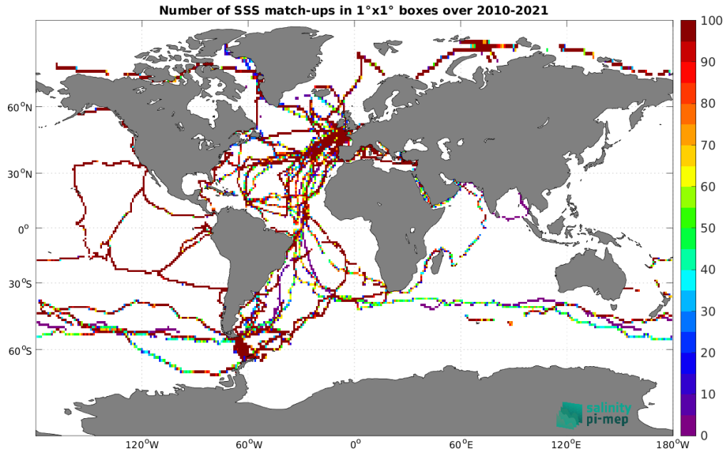
Figure 4: Number of SSS match-ups between TSG (GOSUD-Sailing-ship) SSS and the SMOS SSS L4 v1 - Weekly (CMEMS-CNR) SSS product for the Global Ocean Pi-MEP region over 1^\circ \times 1^\circ boxes and for the full satellite product period.
