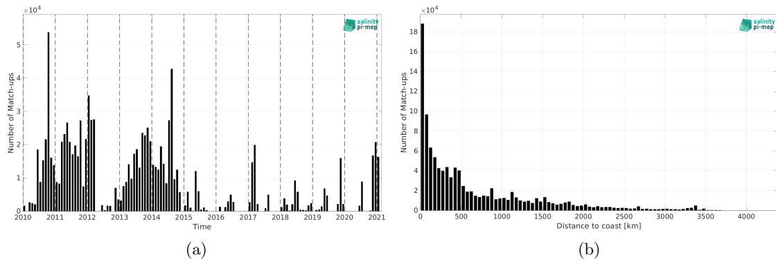
Figure 1: Number of match-ups between TSG (GOSUD-Sailing-ship) and SMOS SSS L4 v1 - Weekly (CMEMS-CNR) SSS as a function of time (a) and as function of the distance to coast (b) over the Global Ocean Pi-MEP region and for the full satellite product period.
