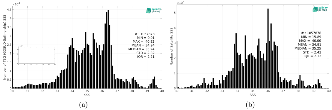
Figure 2: Histograms of SSS from TSG (GOSUD-Sailing-ship) (a) and SMOS SSS L4 v1 - Weekly (CMEMS-CNR) (b) considering all match-up pairs per bins of 0.1 over the Global Ocean Pi-MEP region and for the full satellite product period.
