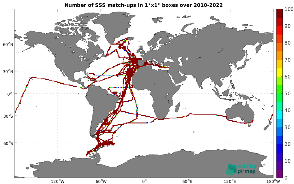
Figure 4: Number of SSS match-ups between TSG (CSIC-UTM) SSS and the SMOS SSS L4 v1 - Weekly (CMEMS-CNR) SSS product for the Global Ocean Pi-MEP region over 1^\circ \times 1^\circ boxes and for the full satellite product period.
