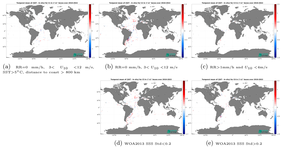
Figure 12: Temporal mean gridded over spatial boxes of size 1^\circ \times 1^\circ of \Delta SSS (SMOS SSS L4 v1 - Weekly (CMEMS-CNR) - TSG (CSIC-UTM)) for 5 different subdatasets corresponding to:RR=0 mm/h, 3 < U_{10} < 12 m/s, SST > 5^\circ\text{C} , distance to coast > 800 km (a), RR=0 mm/h, 3 < U_{10} < 12 m/s (b), RR > 1 mm/h and U_{10} < 4 m/s (c), WOA2013 SSS Std < 0.2 (d), WOA2013 SSS Std > 0.2 (e).
