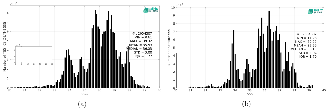
Figure 2: Histograms of SSS from TSG (CSIC-UTM) (a) and SMOS SSS L4 v1 - Weekly (CMEMS-CNR) (b) considering all match-up pairs per bins of 0.1 over the Global Ocean Pi-MEP region and for the full satellite product period.
