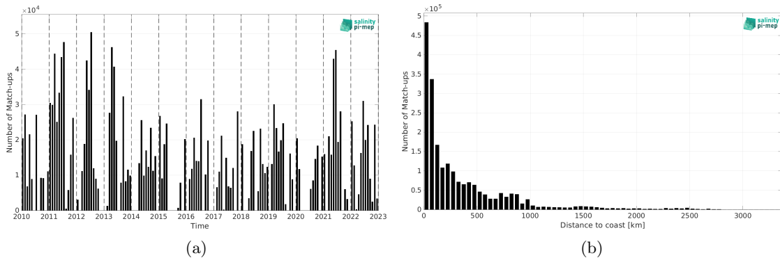
Figure 1: Number of match-ups between TSG (CSIC-UTM) and SMOS SSS L4 v1 - Weekly (CMEMS-CNR) SSS as a function of time (a) and as function of the distance to coast (b) over the Global Ocean Pi-MEP region and for the full satellite product period.
