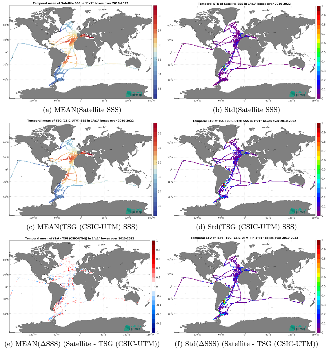
Figure 6: Temporal mean (left) and Std (right) of SSS from SMOS SSS L4 v1 - Weekly (CMEMS-CNR) (top), TSG (CSIC-UTM) (middle), and of \Delta SSS (Satellite - TSG (CSIC-UTM)). Only match-up pairs are used to generate these maps.
