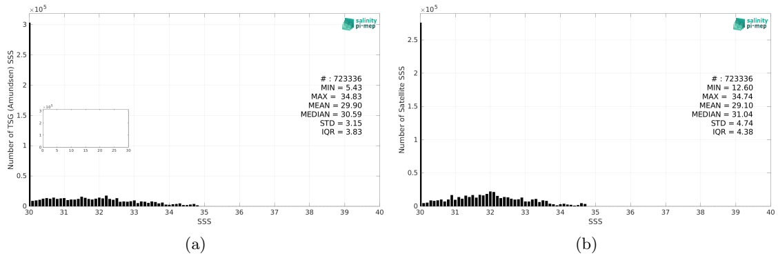
Figure 2: Histograms of SSS from TSG (Amundsen) (a) and SMOS SSS L4 v1 - Weekly (CMEMS-CNR) (b) considering all match-up pairs per bins of 0.1 over the Global Ocean Pi-MEP region and for the full satellite product period.
