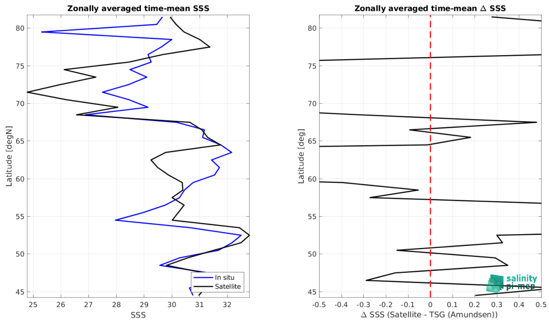
Figure 8: Left panel: Zonal mean SSS from SMOS SSS L4 v1 - Weekly (CMEMS-CNR) satellite product (black) and from TSG (Amundsen) (blue). Right panel: Zonal mean of \Delta SSS (Satellite - TSG (Amundsen)) for all the collected Pi-MEP match-up pairs estimated over the full satellite product period.
