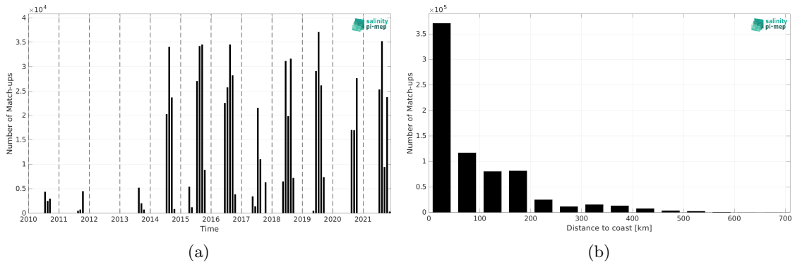
Figure 1: Number of match-ups between TSG (Amundsen) and SMOS SSS L4 v1 - Weekly (CMEMS-CNR) SSS as a function of time (a) and as function of the distance to coast (b) over the Global Ocean Pi-MEP region and for the full satellite product period.
