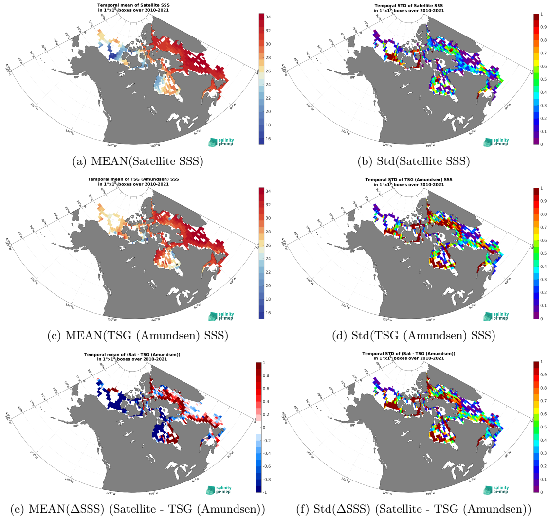
Figure 6: Temporal mean (left) and Std (right) of SSS from SMOS SSS L4 v1 - Weekly (CMEMS-CNR) (top), TSG (Amundsen) (middle), and of \Delta SSS (Satellite - TSG (Amundsen)). Only match-up pairs are used to generate these maps.
