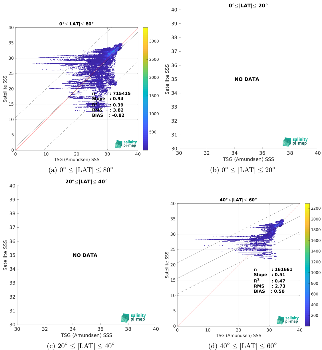
Figure 9: Contour maps of the concentration of SMOS SSS L4 v1 - Weekly (CMEMS-CNR) SSS (y-axis) versus TSG (Amundsen) SSS (x-axis) at match-up pairs for different latitude bands. For each plot, the red line shows x=y . The black thin and dashed lines indicate a linear fit through the data cloud and the \pm 95\% confidence levels, respectively. The number match-up pairs n , the slope and R^2 coefficient of the linear fit, the root mean square (RMS) and the mean bias between satellite and in situ data are indicated for each latitude band in each plot.
