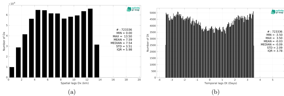
Figure 5: Histograms of the spatial (a) and temporal (b) lags between the location/time of the TSG (Amundsen) measurement and the date of the corresponding SMOS SSS L4 v1 - Weekly (CMEMS-CNR) SSS pixel.
