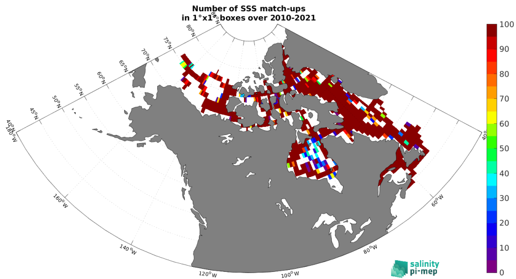
Figure 4: Number of SSS match-ups between TSG (Amundsen) SSS and the SMOS SSS L4 v1 - Weekly (CMEMS-CNR) SSS product for the Global Ocean Pi-MEP region over 1^\circ \times 1^\circ boxes and for the full satellite product period.
