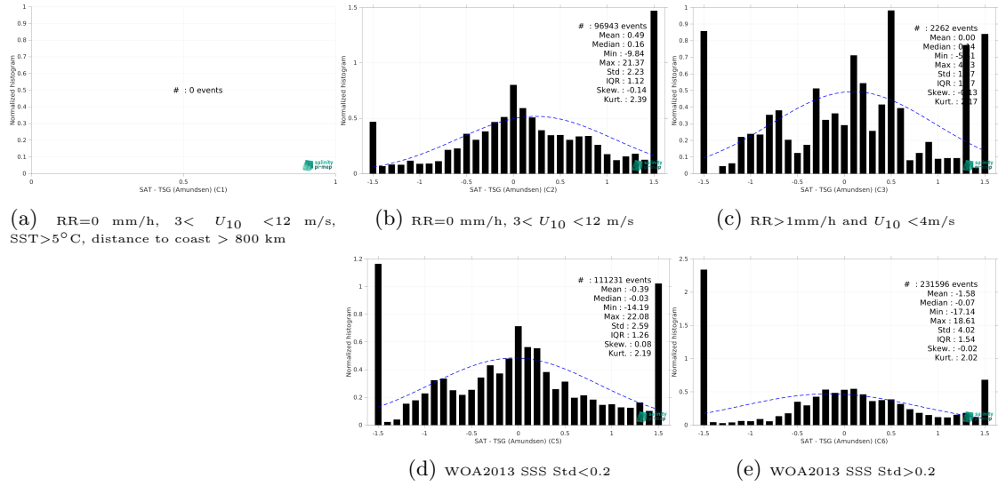
Figure 13: Normalized histogram of \Delta SSS (SMOS SSS L4 v1 - Weekly (CMEMS-CNR) - TSG (Amundsen)) for 5 different subdatasets corresponding to: RR=0 mm/h, 3 < U_{10} < 12 m/s, SST > 5°C, distance to coast > 800 km (a), RR=0 mm/h, 3 < U_{10} < 12 m/s (b), RR > 1mm/h and U_{10} < 4 m/s (c), WOA2013 SSS Std < 0.2 (d), WOA2013 SSS Std > 0.2 (e).
