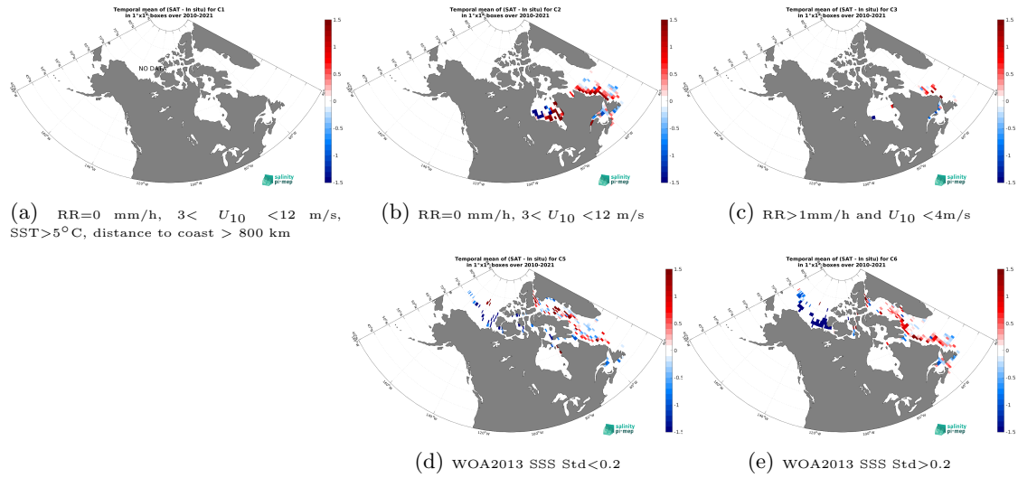
Figure 12: Temporal mean gridded over spatial boxes of size 1^{\circ}\times 1^{\circ} of \Delta\text{SSS} (SMOS SSS L4 v1 - Weekly (CMEMS-CNR) - TSG (Amundsen)) for 5 different subdatasets corresponding to:RR=0 mm/h, 3 < U_{10} < 12 m/s, SST >5^{\circ}\text{C} , distance to coast > 800 km (a), RR=0 mm/h, 3 < U_{10} < 12 m/s (b), RR >1 mm/h and U_{10} < 4 m/s (c), WOA2013 SSS Std <0.2 (d), WOA2013 SSS Std >0.2 (e).
