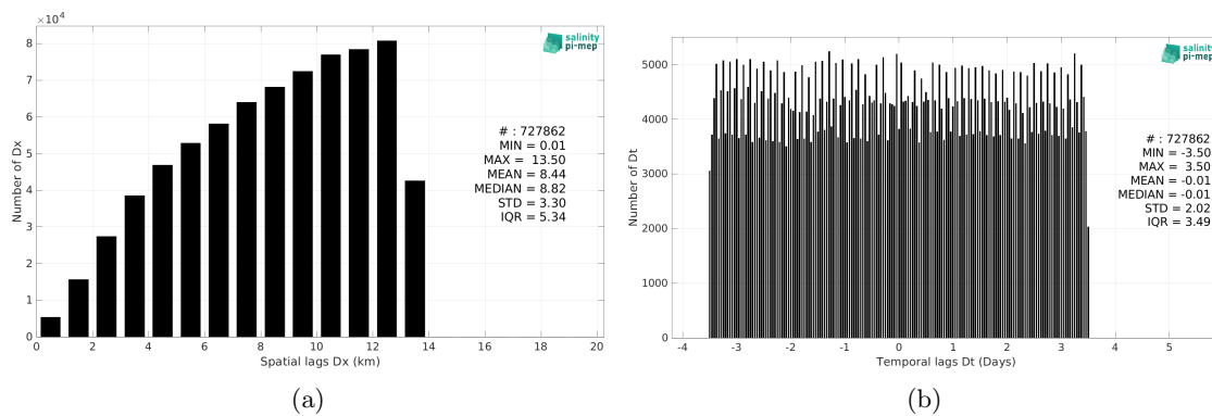
Figure 5: Histograms of the spatial (a) and temporal (b) lags between the location/time of the Sairdrone measurement and the date of the corresponding SMOS SSS L4 v1 - Weekly (CMEMS-CNR) SSS pixel.
