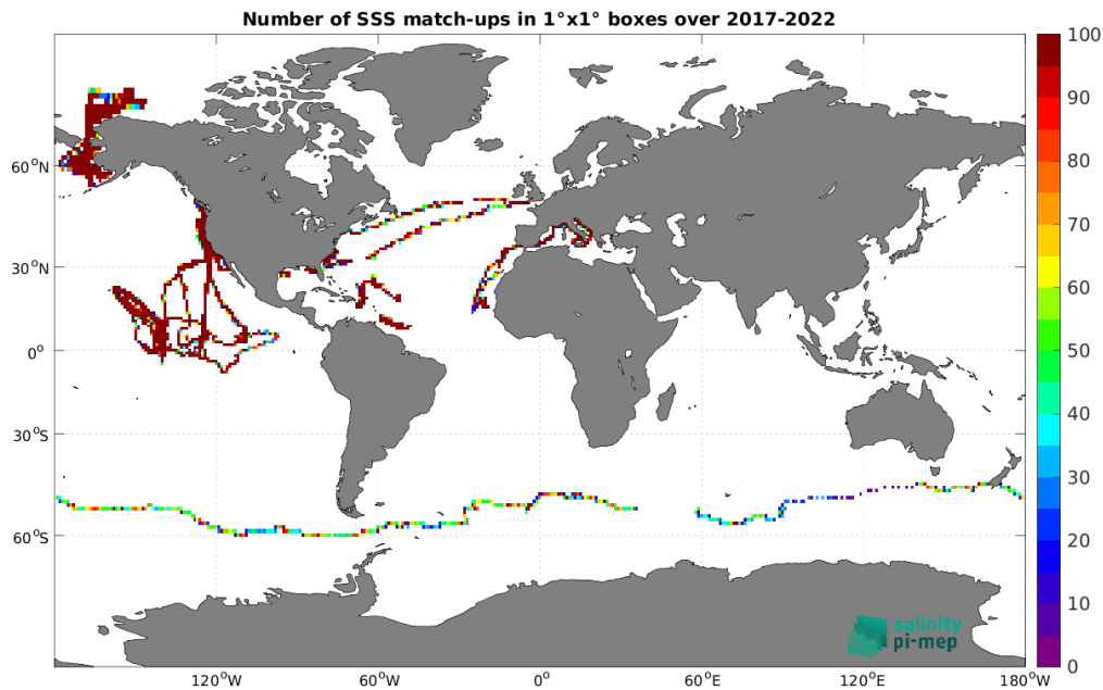
Figure 4: Number of SSS match-ups between Sairdrone SSS and the SMOS SSS L4 v1 - Weekly (CMEMS-CNR) SSS product for the Global Ocean Pi-MEP region over 1^\circ \times 1^\circ boxes and for the full satellite product period.
