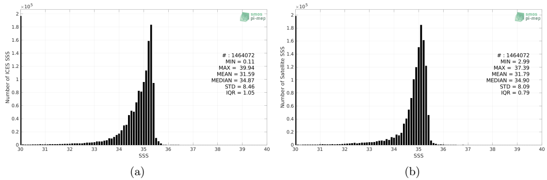
Figure 2: Histograms of SSS from ICES (a) and SMOS SSS L4 v1 - Weekly (CMEMS-CNR) (b) considering all match-up pairs per bins of 0.1 over the Global Ocean Pi-MEP region and for the full satellite product period.
