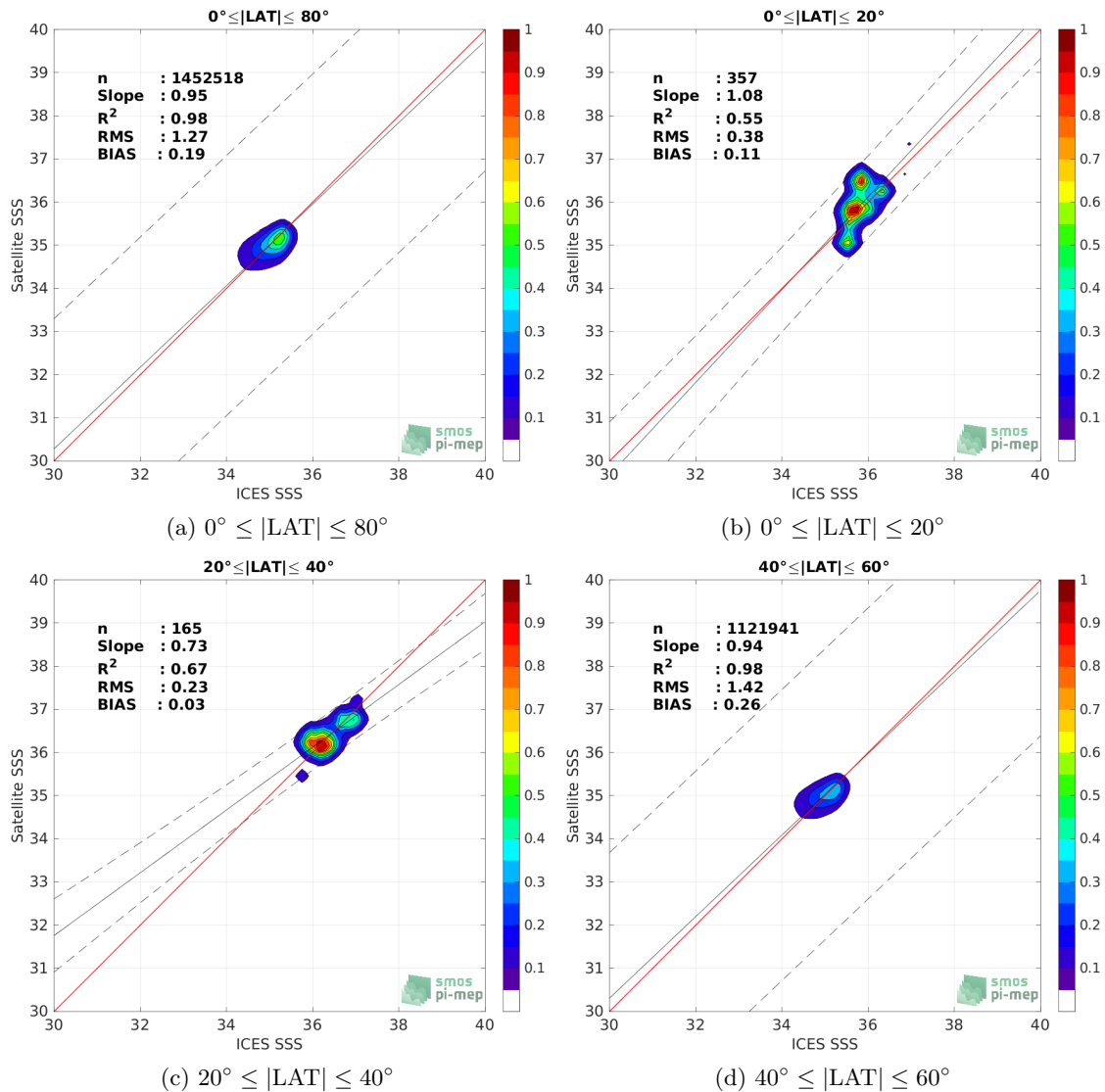
Figure 9: Contour maps of the concentration of SMOS SSS L4 v1 - Weekly (CMEMS-CNR) SSS (y-axis) versus ICES SSS (x-axis) at match-up pairs for different latitude bands. For each plot, the red line shows x=y . The black thin and dashed lines indicate a linear fit through the data cloud and the \pm 95\% confidence levels, respectively. The number match-up pairs n , the slope and R^2 coefficient of the linear fit, the root mean square (RMS) and the mean bias between satellite and in situ data are indicated for each latitude band in each plots.
