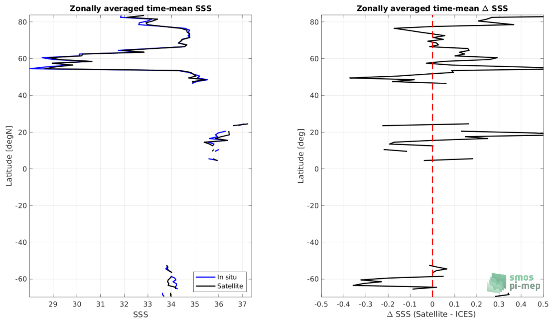
Figure 8: Left panel: Zonal mean SSS from SMOS SSS L4 v1 - Weekly (CMEMS-CNR) satellite product (black) and from ICES (blue). Right panel: Zonal mean of \Delta SSS (Satellite - ICES) for all the collected Pi-MEP match-up pairs estimated over the full satellite product period.
