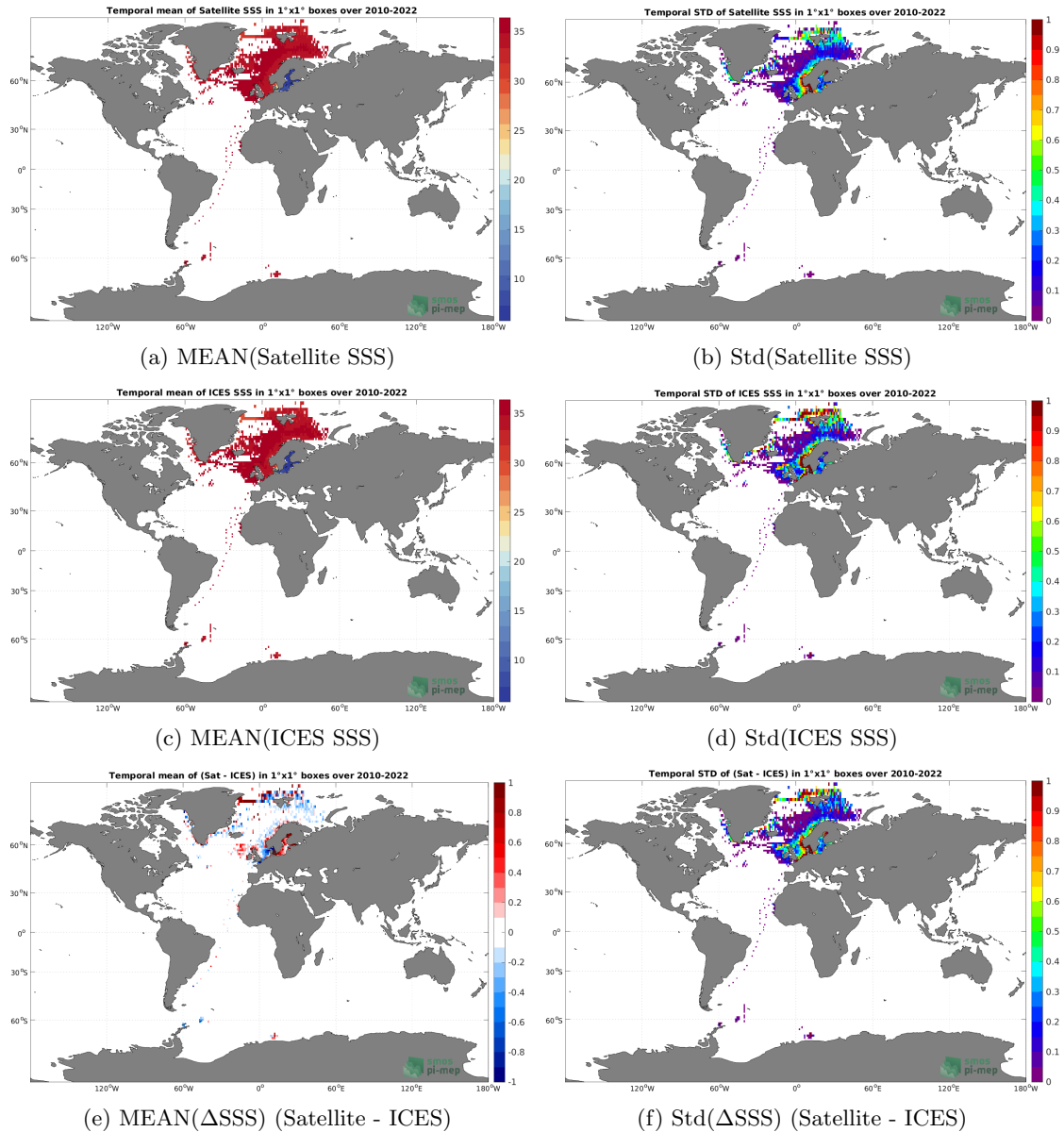
Figure 6: Temporal mean (left) and Std (right) of SSS from SMOS SSS L4 v1 - Weekly (CMEMS-CNR) (top), ICES (middle), and of \Delta SSS (Satellite - ICES). Only match-up pairs are used to generate these maps.
