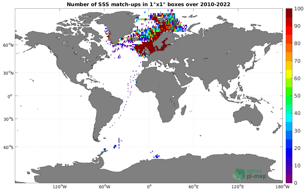
Figure 4: Number of SSS match-ups between ICES SSS and the SMOS SSS L4 v1 - Weekly (CMEMS-CNR) SSS product for the Global Ocean Pi-MEP region over 1^\circ \times 1^\circ boxes and for the full satellite product period.
