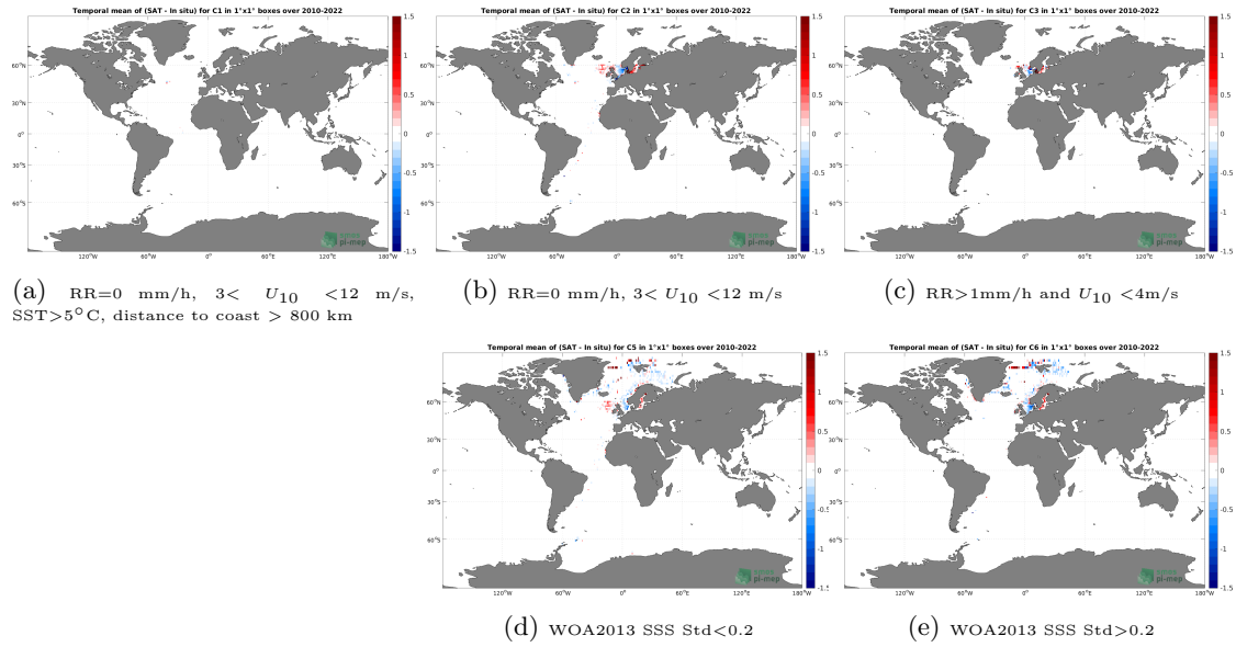
Figure 12: Temporal mean gridded over spatial boxes of size 1^\circ \times 1^\circ of \Delta SSS (SMOS SSS L4 v1 - Weekly (CMEMS-CNR) - ICES) for 5 different subdatasets corresponding to:RR=0 mm/h, 3 < U_{10} < 12 m/s, SST >5^\circ C, distance to coast > 800 km (a), RR=0 mm/h, 3 < U_{10} < 12 m/s (b), RR >1 mm/h and U_{10} < 4 m/s (c), WOA2013 SSS Std <0.2 (d), WOA2013 SSS Std >0.2 (e).
