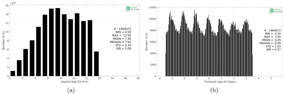
Figure 5: Histograms of the spatial (a) and temporal (b) lags between the location/time of the ICES measurement and the date of the corresponding SMOS SSS L4 v1 - Weekly (CMEMS-CNR) SSS pixel.
