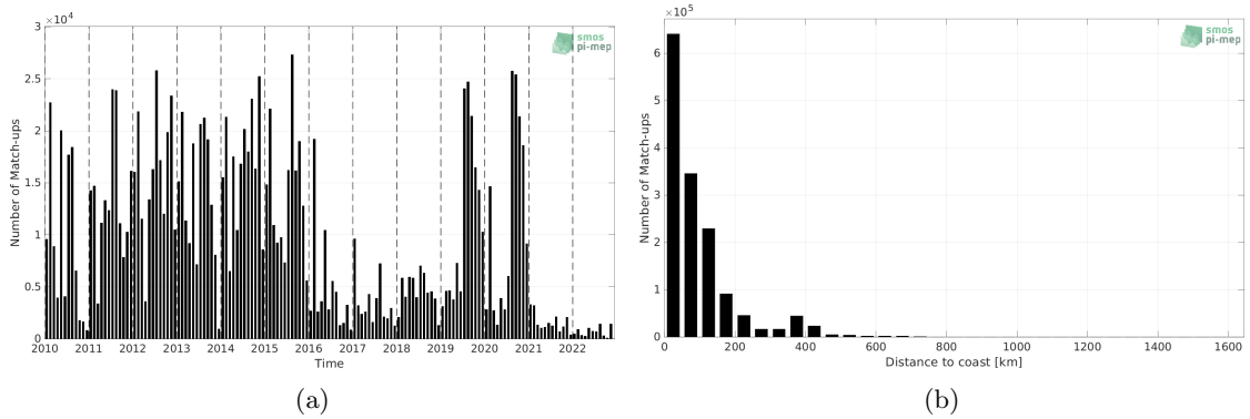
Figure 1: Number of match-ups between ICES and SMOS SSS L4 v1 - Weekly (CMEMS-CNR) SSS as a function of time (a) and as function of the distance to coast (b) over the Global Ocean Pi-MEP region and for the full satellite product period.
