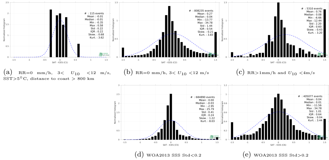
Figure 13: Normalized histogram of \Delta SSS (SMOS SSS L4 v1 - Weekly (CMEMS-CNR) - ICES) for 5 different subdatasets corresponding to: RR=0 mm/h, 3 < U_{10} < 12 m/s, SST > 5°C, distance to coast > 800 km (a), RR=0 mm/h, 3 < U_{10} < 12 m/s (b), RR > 1mm/h and U_{10} < 4 m/s (c), WOA2013 SSS Std < 0.2 (d), WOA2013 SSS Std > 0.2 (e).
