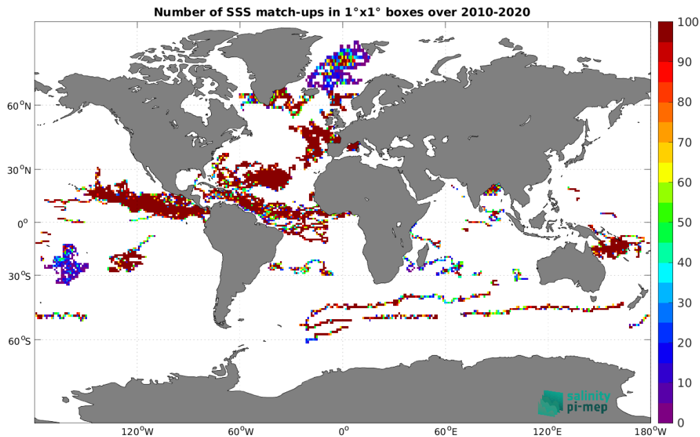
Figure 3: Number of SSS match-ups between Surface drifters SSS and the SMOS SSS L4 v1 - Weekly (CMEMS-CNR) SSS product for the Global Ocean Pi-MEP region over 1^\circ \times 1^\circ boxes and for the full satellite product period.
