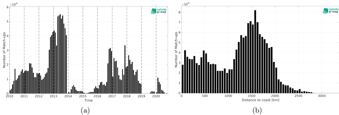
Figure 1: Number of match-ups between Surface drifters and SMOS SSS L4 v1 - Weekly (CMEMS-CNR) SSS as a function of time (a) and as function of the distance to coast (b) over the Global Ocean Pi-MEP region and for the full satellite product period.
