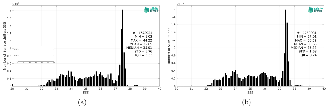
Figure 2: Histograms of SSS from Surface drifters (a) and SMOS SSS L4 v1 - Weekly (CMEMS-CNR) (b) considering all match-up pairs per bins of 0.1 over the Global Ocean Pi-MEP region and for the full satellite product period.
