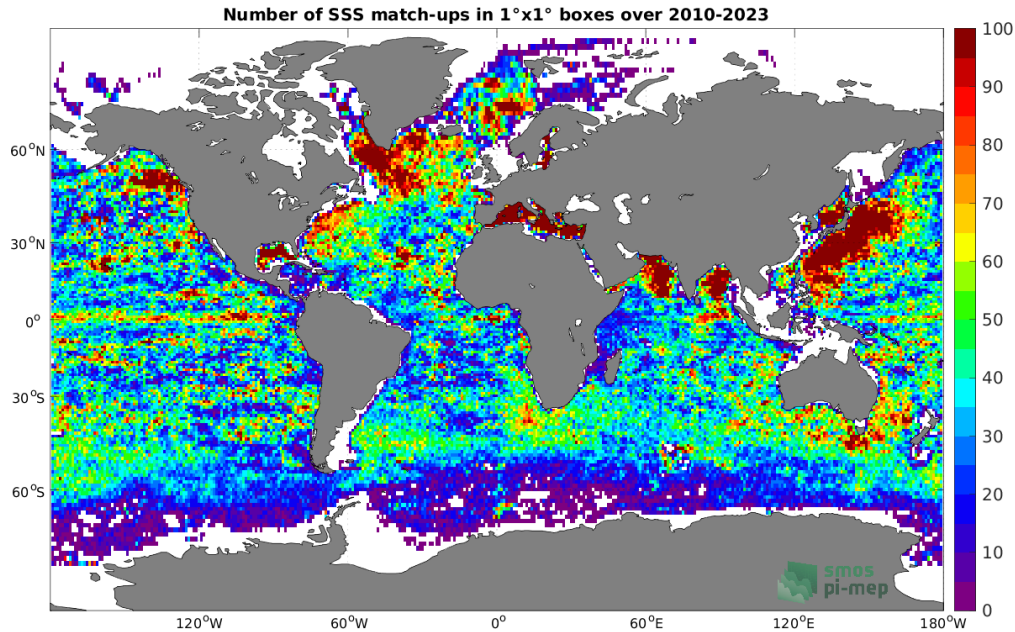
Figure 4: Number of SSS match-ups between Argo SSS and the SMOS SSS L4 v1 - Weekly (CMEMS-CNR) SSS product for the Global Ocean Pi-MEP region over 1^\circ \times 1^\circ boxes and for the full satellite product period.
