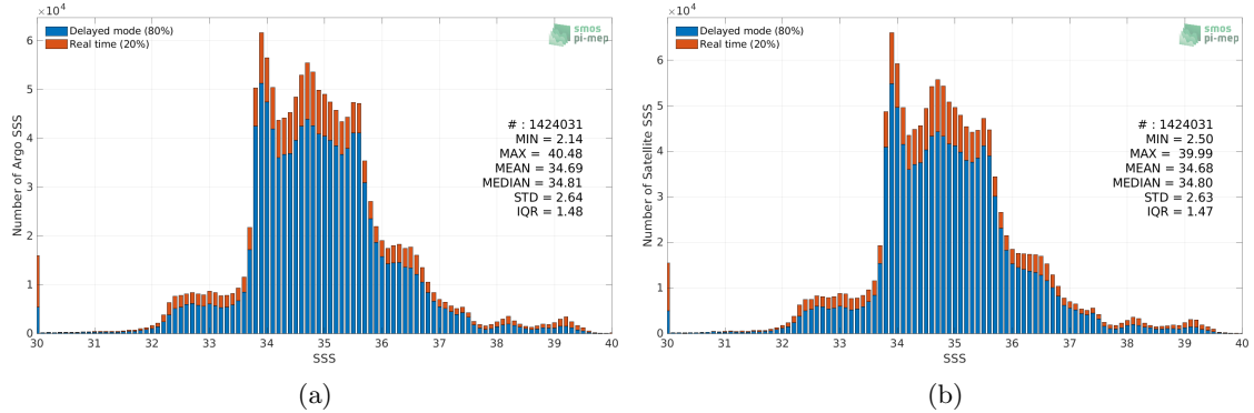
Figure 2: Histograms of SSS from Argo (a) and SMOS SSS L4 v1 - Weekly (CMEMS-CNR) (b) considering all match-up pairs per bins of 0.1 over the Global Ocean Pi-MEP region and for the full satellite product period.
