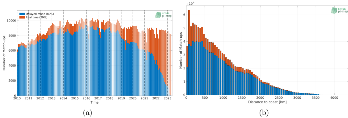
Figure 1: Number of match-ups between Argo and SMOS SSS L4 v1 - Weekly (CMEMS-CNR) SSS as a function of time (a) and as function of the distance to coast (b) over the Global Ocean Pi-MEP region and for the full satellite product period.
