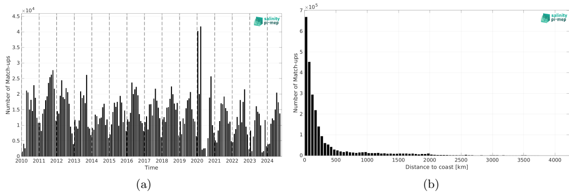
Figure 2: Number of match-ups between TSG (SAMOS) and SMOS SSS L4 v1 - Monthly (CMEMS-CNR) SSS as a function of time (a) and as function of the distance to coast (b) over the Global Ocean Pi-MEP region and for the full satellite product period.
