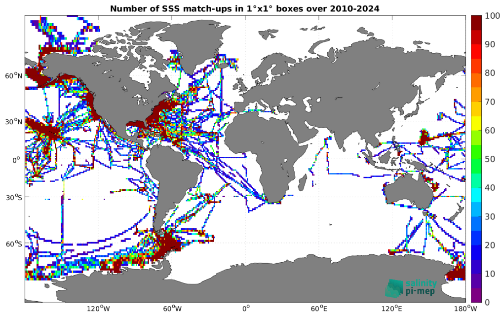
Figure 5: Number of SSS match-ups between TSG (SAMOS) SSS and the SMOS SSS L4 v1 - Monthly (CMEMS-CNR) SSS product for the Global Ocean Pi-MEP region over 1^\circ \times 1^\circ boxes and for the full satellite product period.
