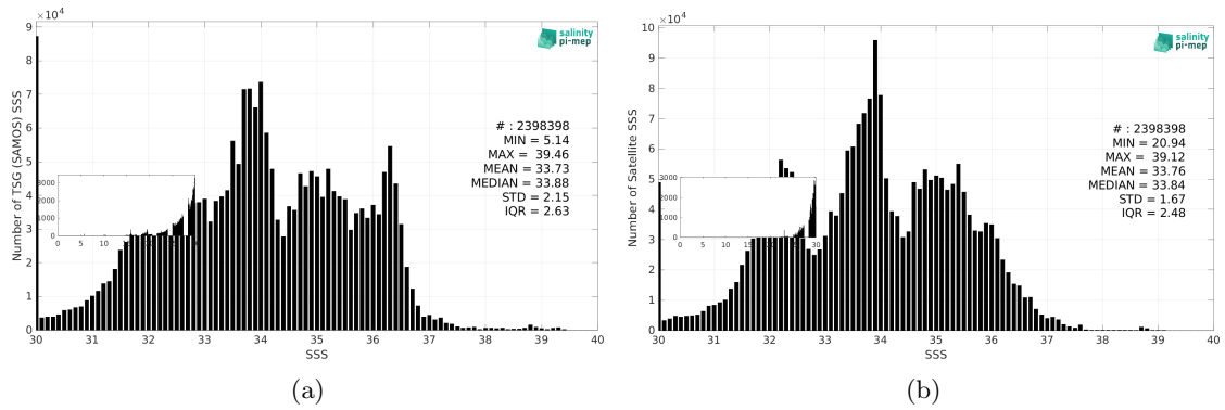
Figure 3: Histograms of SSS from TSG (SAMOS) (a) and SMOS SSS L4 v1 - Monthly (CMEMS-CNR) (b) considering all match-up pairs per bins of 0.1 over the Global Ocean Pi-MEP region and for the full satellite product period.
