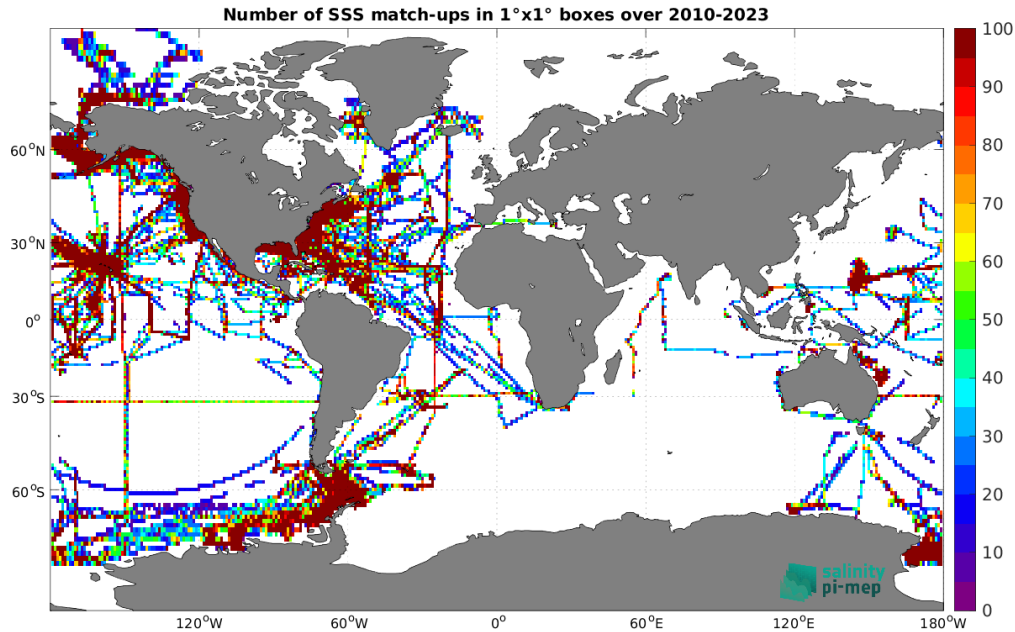
Figure 4: Number of SSS match-ups between TSG (SAMOS) SSS and the SMOS SSS L4 v1 - Monthly (CMEMS-CNR) SSS product for the Global Ocean Pi-MEP region over 1^{\circ} \times 1^{\circ} boxes and for the full satellite product period.
