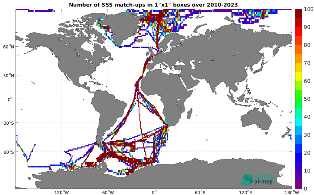
Figure 5: Number of SSS match-ups between TSG (Polarstern) SSS and the SMOS SSS L4 v1 - Monthly (CMEMS-CNR) SSS product for the Global Ocean Pi-MEP region over 1^\circ \times 1^\circ boxes and for the full satellite product period.
