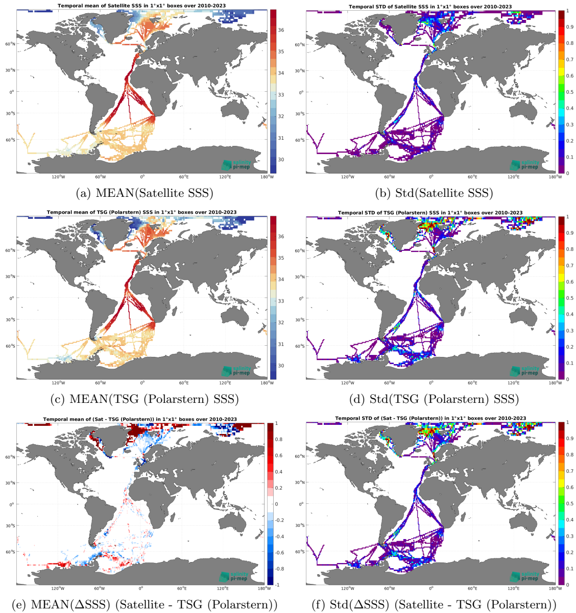
Figure 7: Temporal mean (left) and Std (right) of SSS from SMOS SSS L4 v1 - Monthly (CMEMS-CNR) (top), TSG (Polarstern) (middle), and of \Delta SSS (Satellite - TSG (Polarstern)). Only match-up pairs are used to generate these maps.
