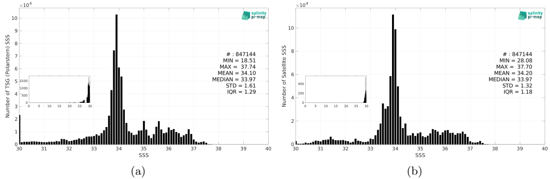
Figure 3: Histograms of SSS from TSG (Polarstern) (a) and SMOS SSS L4 v1 - Monthly (CMEMS-CNR) (b) considering all match-up pairs per bins of 0.1 over the Global Ocean Pi-MEP region and for the full satellite product period.
