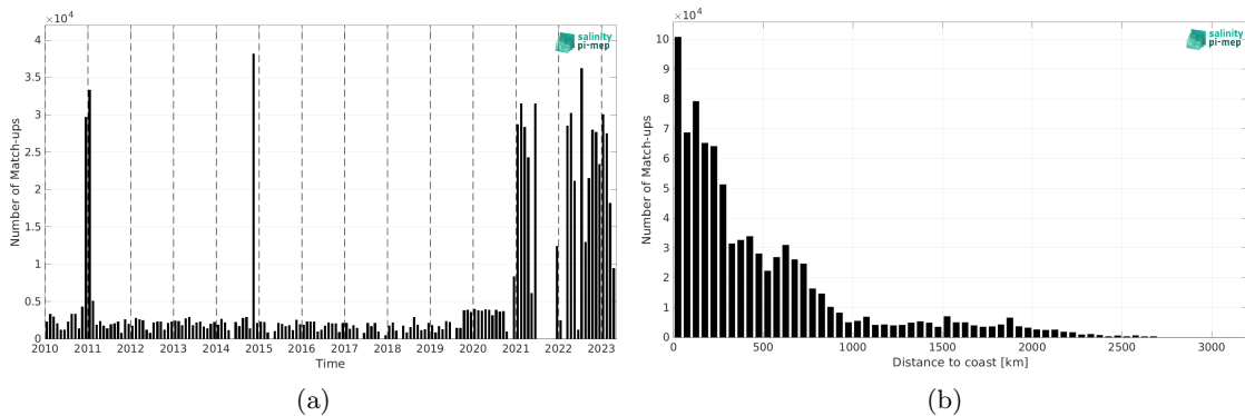
Figure 2: Number of match-ups between TSG (Polarstern) and SMOS SSS L4 v1 - Monthly (CMEMS-CNR) SSS as a function of time (a) and as function of the distance to coast (b) over the Global Ocean Pi-MEP region and for the full satellite product period.
