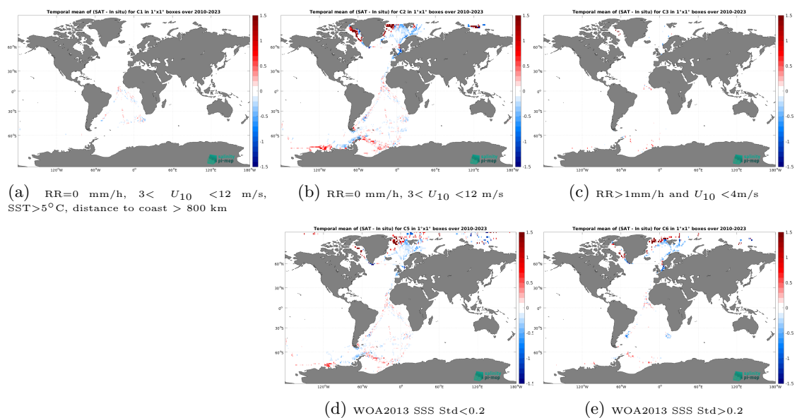
Figure 14: Temporal mean gridded over spatial boxes of size 1^\circ \times 1^\circ of \Delta\text{SSS} (SMOS SSS L4 v1 - Monthly (CMEMS-CNR) - TSG (Polarstern)) for 5 different subdatasets corresponding to:RR=0 mm/h, 3 < U_{10} < 12 m/s, SST > 5^\circ\text{C} , distance to coast > 800 km (a), RR=0 mm/h, 3 < U_{10} < 12 m/s (b), RR > 1 mm/h and U_{10} < 4 m/s (c), WOA2013 SSS Std < 0.2 (d), WOA2013 SSS Std > 0.2 (e).
