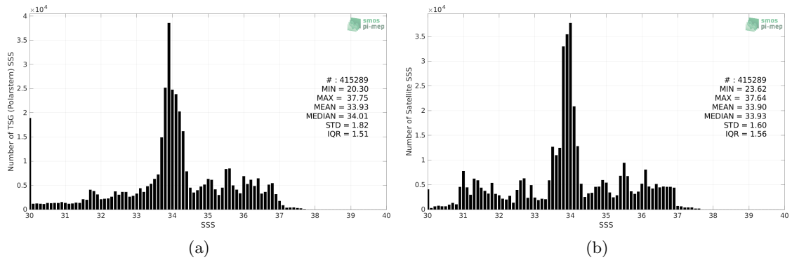
Figure 2: Histograms of SSS from TSG (Polarstern) (a) and SMOS SSS L4 v1 - Monthly (CMEMS-CNR) (b) considering all match-up pairs per bins of 0.1 over the Global Ocean Pi-MEP region and for the full satellite product period.
