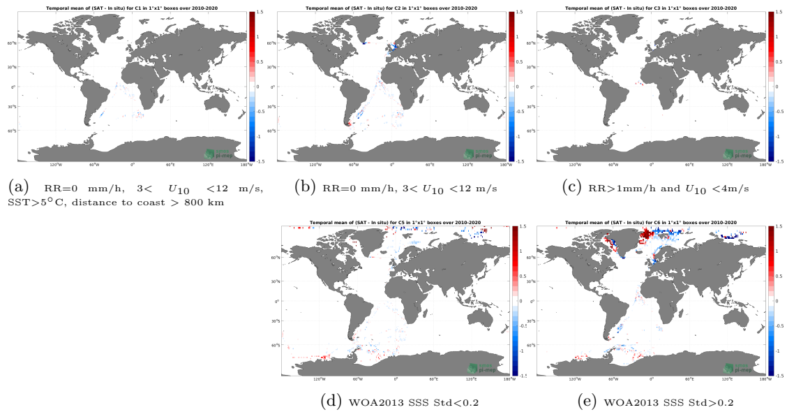
Figure 12: Temporal mean gridded over spatial boxes of size 1^\circ \times 1^\circ of \Delta SSS (SMOS SSS L4 v1 - Monthly (CMEMS-CNR) - TSG (Polarstern)) for 5 different subdatasets corresponding to:RR=0 mm/h, 3 < U_{10} < 12 m/s, SST > 5^\circ\text{C} , distance to coast > 800 km (a), RR=0 mm/h, 3 < U_{10} < 12 m/s (b), RR > 1 mm/h and U_{10} < 4 m/s (c), WOA2013 SSS Std < 0.2 (d), WOA2013 SSS Std > 0.2 (e).
