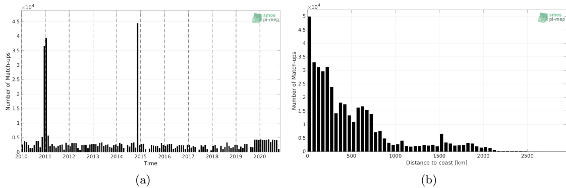
Figure 1: Number of match-ups between TSG (Polarstern) and SMOS SSS L4 v1 - Monthly (CMEMS-CNR) SSS as a function of time (a) and as function of the distance to coast (b) over the Global Ocean Pi-MEP region and for the full satellite product period.
