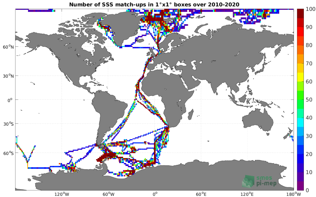
Figure 4: Number of SSS match-ups between TSG (Polarstern) SSS and the SMOS SSS L4 v1 - Monthly (CMEMS-CNR) SSS product for the Global Ocean Pi-MEP region over 1^\circ \times 1^\circ boxes and for the full satellite product period.
