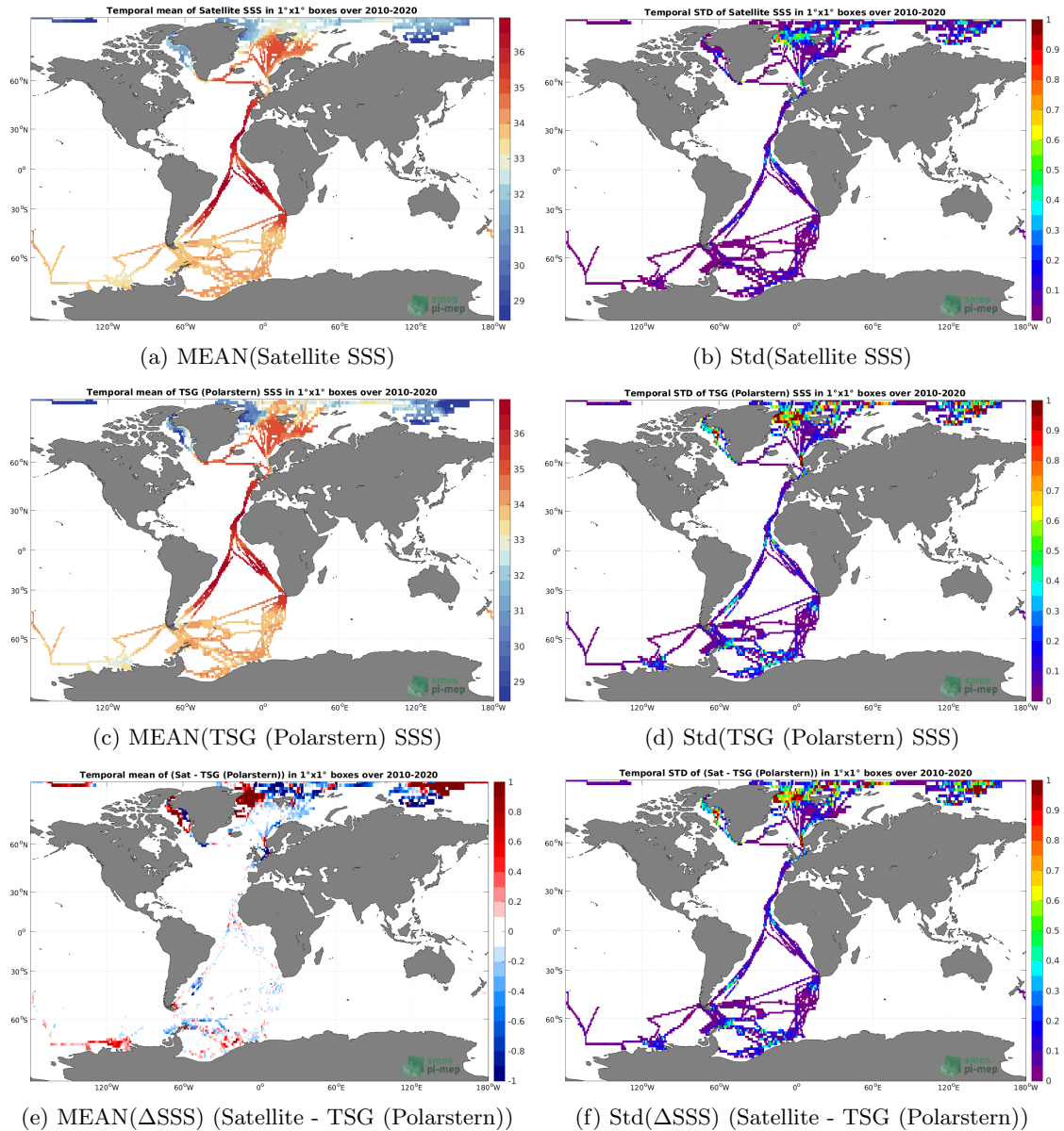
Figure 6: Temporal mean (left) and Std (right) of SSS from SMOS SSS L4 v1 - Monthly (CMEMS-CNR) (top), TSG (Polarstern) (middle), and of \Delta SSS (Satellite - TSG (Polarstern)). Only match-up pairs are used to generate these maps.
