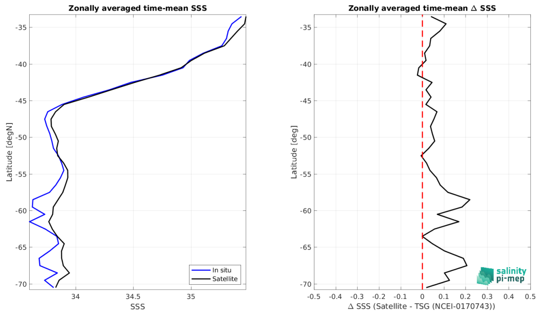
Figure 9: Left panel: Zonal mean SSS from SMOS SSS L4 v1 - Monthly (CMEMS-CNR) satellite product (black) and from TSG (NCEI-0170743) (blue). Right panel: Zonal mean of \Delta SSS (Satellite - TSG (NCEI-0170743)) for all the collected Pi-MEP match-up pairs estimated over the full satellite product period.
