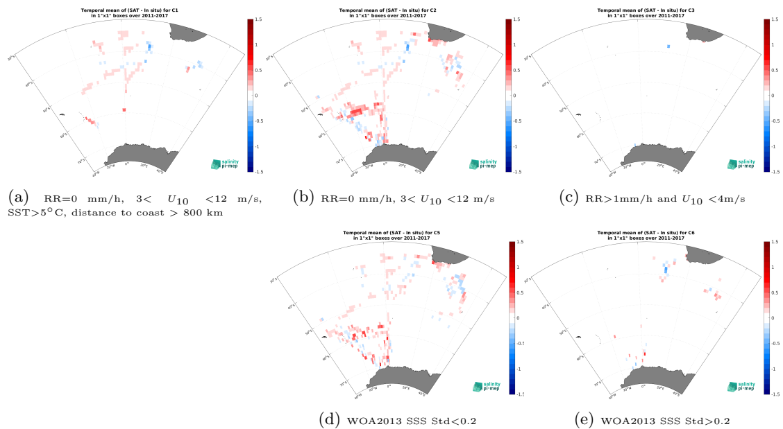
Figure 14: Temporal mean gridded over spatial boxes of size 1^\circ \times 1^\circ of \Delta SSS (SMOS SSS L4 v1 - Monthly (CMEMS-CNR) - TSG (NCEI-0170743)) for 5 different subdatasets corresponding to:RR=0 mm/h, 3 < U_{10} < 12 m/s, SST >5^\circ\text{C} , distance to coast > 800 km (a), RR=0 mm/h, 3 < U_{10} < 12 m/s (b), RR >1 mm/h and U_{10} < 4 m/s (c), WOA2013 SSS Std <0.2 (d), WOA2013 SSS Std >0.2 (e).
