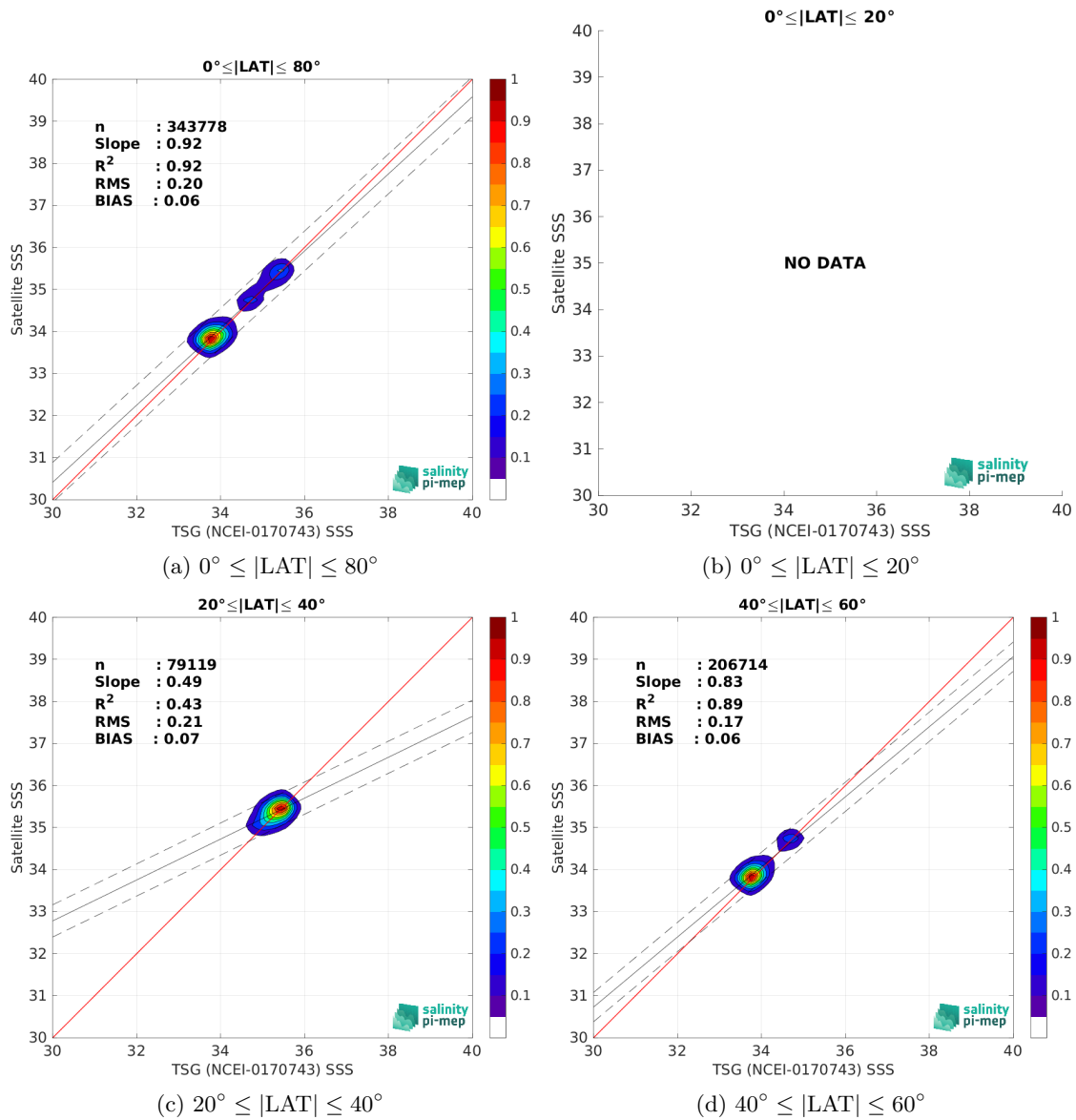
Figure 10: Contour maps of the concentration of SMOS SSS L4 v1 - Monthly (CMEMS-CNR) SSS (y-axis) versus TSG (NCEI-0170743) SSS (x-axis) at match-up pairs for different latitude bands. For each plot, the red line shows x=y . The black thin and dashed lines indicate a linear fit through the data cloud and the \pm 95\% confidence levels, respectively. The number match-up pairs n , the slope and R^2 coefficient of the linear fit, the root mean square (RMS) and the mean bias between satellite and in situ data are indicated for each latitude band in each plots.
