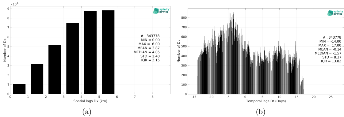
Figure 6: Histograms of the spatial (a) and temporal (b) lags between the location/time of the TSG (NCEI-0170743) measurement and the date of the corresponding SMOS SSS L4 v1 - Monthly (CMEMS-CNR) SSS pixel.
