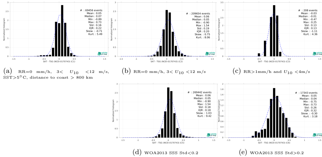
Figure 15: Normalized histogram of \Delta SSS (SMOS SSS L4 v1 - Monthly (CMEMS-CNR) - TSG (NCEI-0170743)) for 5 different subdatasets corresponding to: RR=0 mm/h, 3 < U_{10} < 12 m/s, SST > 5°C, distance to coast > 800 km (a), RR=0 mm/h, 3 < U_{10} < 12 m/s (b), RR > 1mm/h and U_{10} < 4 m/s (c), WOA2013 SSS Std < 0.2 (d), WOA2013 SSS Std > 0.2 (e).
