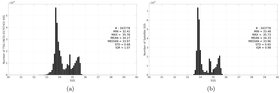
Figure 3: Histograms of SSS from TSG (NCEI-0170743) (a) and SMOS SSS L4 v1 - Monthly (CMEMS-CNR) (b) considering all match-up pairs per bins of 0.1 over the Global Ocean Pi-MEP region and for the full satellite product period.
