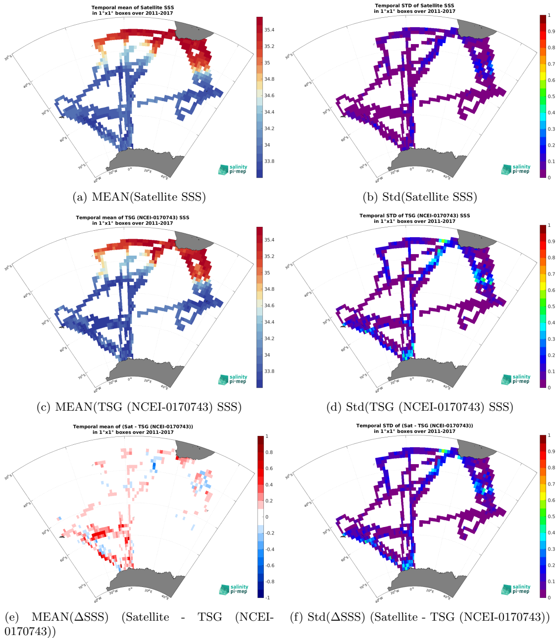
Figure 7: Temporal mean (left) and Std (right) of SSS from SMOS SSS L4 v1 - Monthly (CMEMS-CNR) (top), TSG (NCEI-0170743) (middle), and of \Delta SSS (Satellite - TSG (NCEI-0170743)). Only match-up pairs are used to generate these maps.
