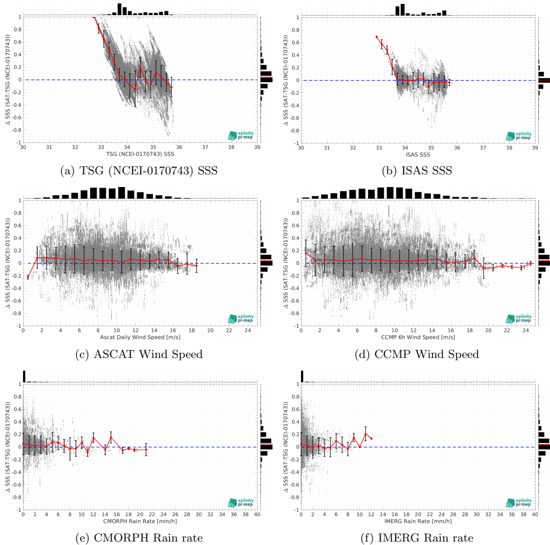
Figure 12: \Delta \text{SSS (Satellite - TSG (NCEI-0170743))} sorted as function of TSG (NCEI-0170743) SSS values (a), ISAS SSS (b), ASCAT Wind speed (c), CCMP Wind speed (d), CMORPH rain rate (e) and IMERG rain rate (f). In all plots the median and Std of \Delta \text{SSS} for each bin is indicated by the red curves and black vertical thick bars ( \pm 1 Std).
