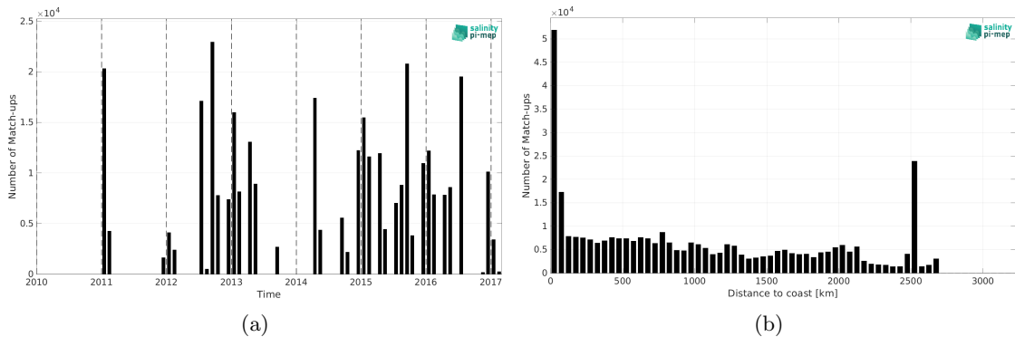
Figure 2: Number of match-ups between TSG (NCEI-0170743) and SMOS SSS L4 v1 - Monthly (CMEMS-CNR) SSS as a function of time (a) and as function of the distance to coast (b) over the Global Ocean Pi-MEP region and for the full satellite product period.
