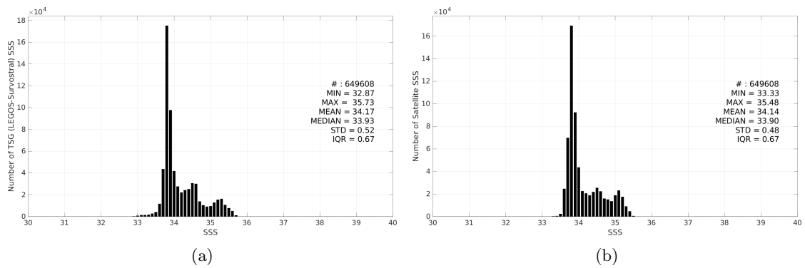
Figure 3: Histograms of SSS from TSG (LEGOS-Survostral) (a) and SMOS SSS L4 v1 - Monthly (CMEMS-CNR) (b) considering all match-up pairs per bins of 0.1 over the Global Ocean Pi-MEP region and for the full satellite product period.
