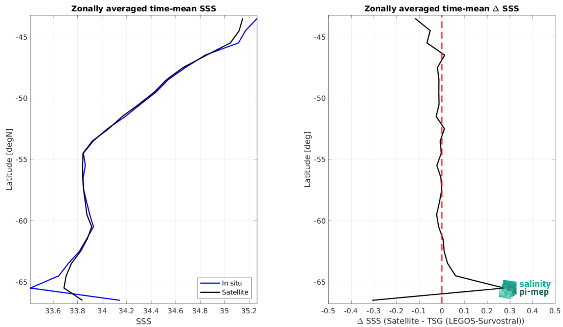
Figure 9: Left panel: Zonal mean SSS from SMOS SSS L4 v1 - Monthly (CMEMS-CNR) satellite product (black) and from TSG (LEGOS-Survostral) (blue). Right panel: Zonal mean of \Delta SSS (Satellite - TSG (LEGOS-Survostral)) for all the collected Pi-MEP match-up pairs estimated over the full satellite product period.
