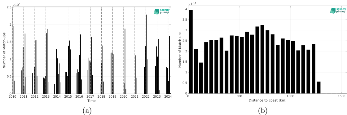
Figure 2: Number of match-ups between TSG (LEGOS-Survostral) and SMOS SSS L4 v1 - Monthly (CMEMS-CNR) SSS as a function of time (a) and as function of the distance to coast (b) over the Global Ocean Pi-MEP region and for the full satellite product period.
