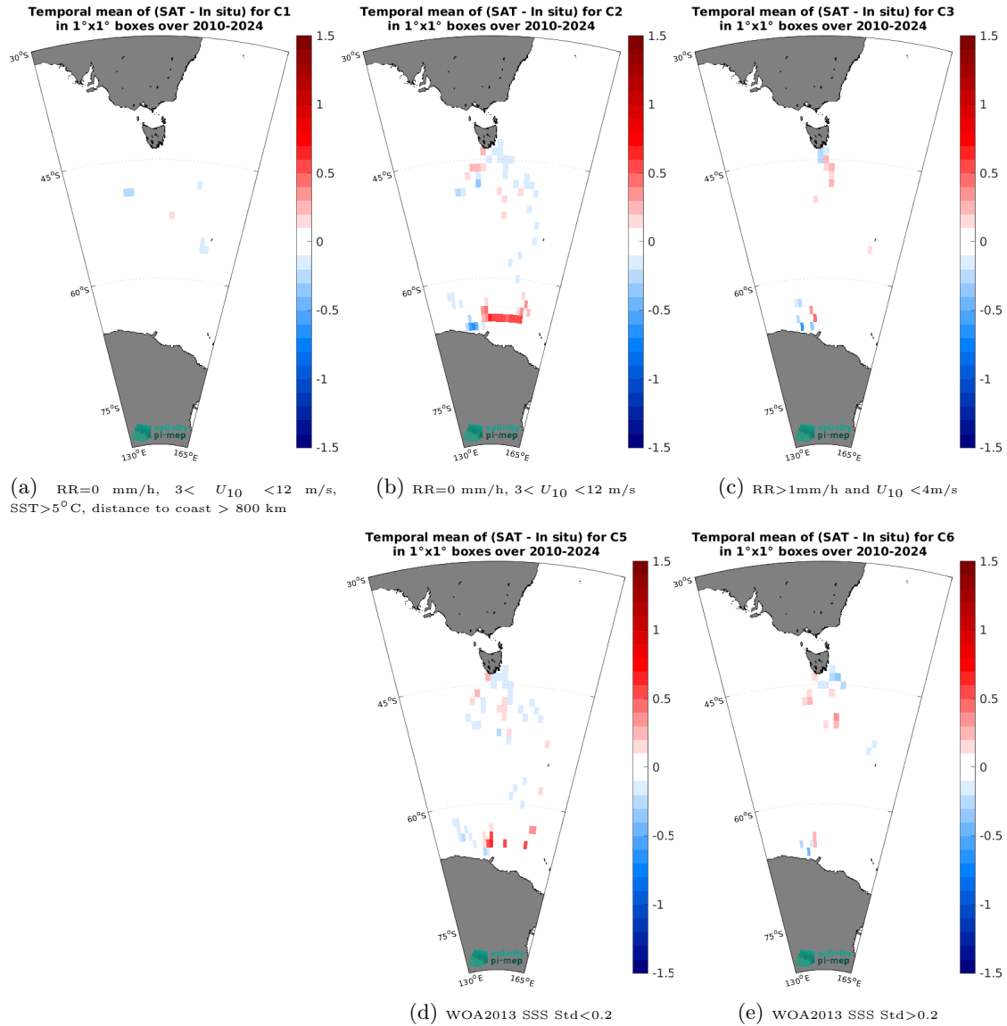
Figure 14: Temporal mean gridded over spatial boxes of size 1^\circ \times 1^\circ of \Delta SSS (SMOS SSS L4 v1 - Monthly (CMEMS-CNR) - TSG (LEGOS-Survostral)) for 5 different subdatasets corresponding to: RR=0 mm/h, 3 < U_{10} < 12 m/s, SST>5°C, distance to coast > 800 km (a), RR=0 mm/h, 3 < U_{10} < 12 m/s (b), RR>1mm/h and U_{10} < 4 m/s (c), WOA2013 SSS Std<0.2 (d), WOA2013 SSS Std>0.2 (e).
