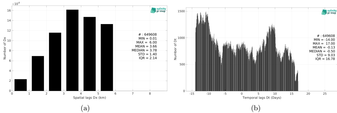
Figure 6: Histograms of the spatial (a) and temporal (b) lags between the location/time of the TSG (LEGOS-Survostral) measurement and the date of the corresponding SMOS SSS L4 v1 - Monthly (CMEMS-CNR) SSS pixel.
