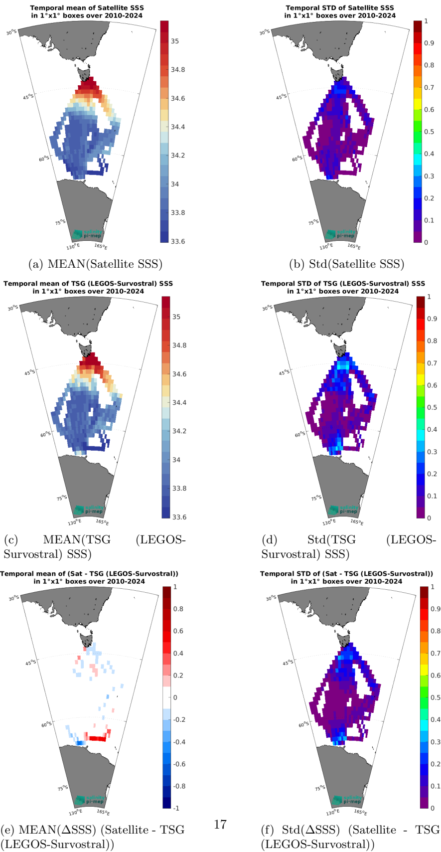
Figure 7: Temporal mean (left) and Std (right) of SSS from SMOS SSS L4 v1 - Monthly (CMEMS-CNR) (top), TSG (LEGOS-Survostral) (middle), and of \Delta SSS (Satellite - TSG (LEGOS-Survostral)). Only match-up pairs are used to generate these maps.
