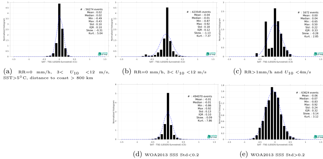
Figure 15: Normalized histogram of \Delta SSS (SMOS SSS L4 v1 - Monthly (CMEMS-CNR) - TSG (LEGOs-Survostral)) for 5 different subdatasets corresponding to: RR=0 mm/h, 3 < U_{10} < 12 m/s, SST>5°C, distance to coast > 800 km (a), RR=0 mm/h, 3 < U_{10} < 12 m/s (b), RR>1mm/h and U_{10} < 4 m/s (c), WOA2013 SSS Std<0.2 (d), WOA2013 SSS Std>0.2 (e).
