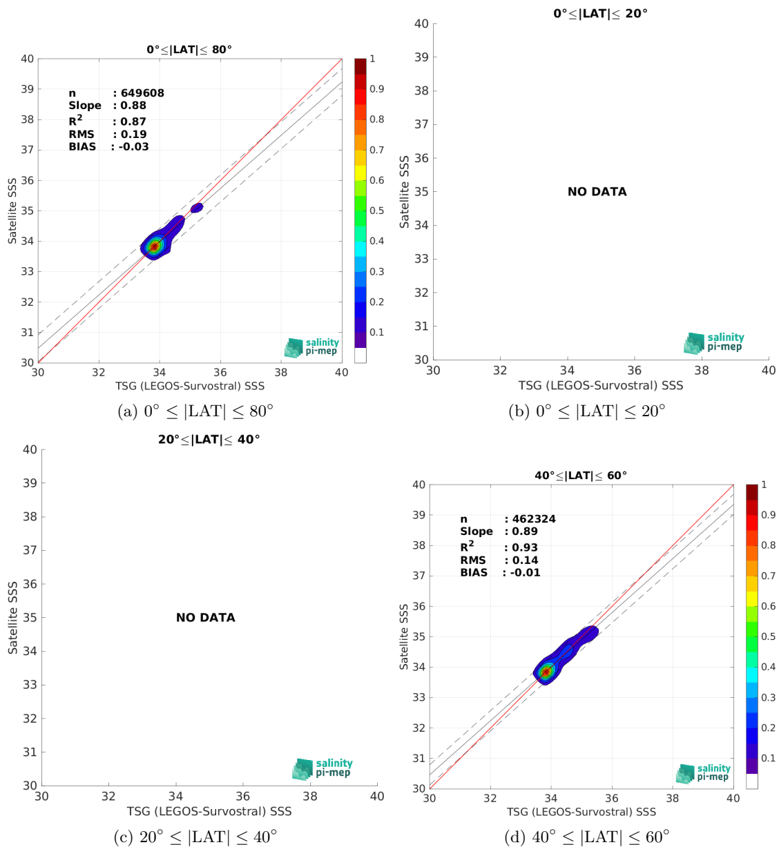
Figure 10: Contour maps of the concentration of SMOS SSS L4 v1 - Monthly (CMEMS-CNR) SSS (y-axis) versus TSG (LEGOS-Survostral) SSS (x-axis) at match-up pairs for different latitude bands. For each plot, the red line shows x=y . The black thin and dashed lines indicate a linear fit through the data cloud and the \pm 95\% confidence levels, respectively. The number match-up pairs n , the slope and R^2 coefficient of the linear fit, the root mean square (RMS) and the mean bias between satellite and in situ data are indicated for each latitude band in each plots.
