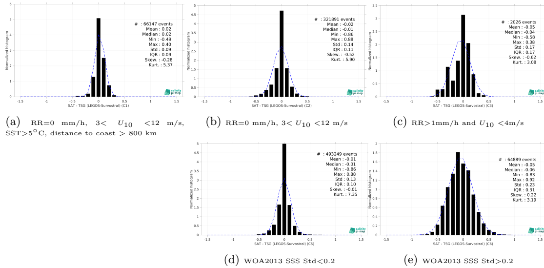
Figure 13: Normalized histogram of \Delta SSS (SMOS SSS L4 v1 - Monthly (CMEMS-CNR) - TSG (LEGOS-Survostral)) for 5 different subdatasets corresponding to: RR=0 mm/h, 3 < U_{10} < 12 m/s, SST>5°C, distance to coast > 800 km (a), RR=0 mm/h, 3 < U_{10} < 12 m/s (b), RR>1mm/h and U_{10} < 4 m/s (c), WOA2013 SSS Std<0.2 (d), WOA2013 SSS Std>0.2 (e).
