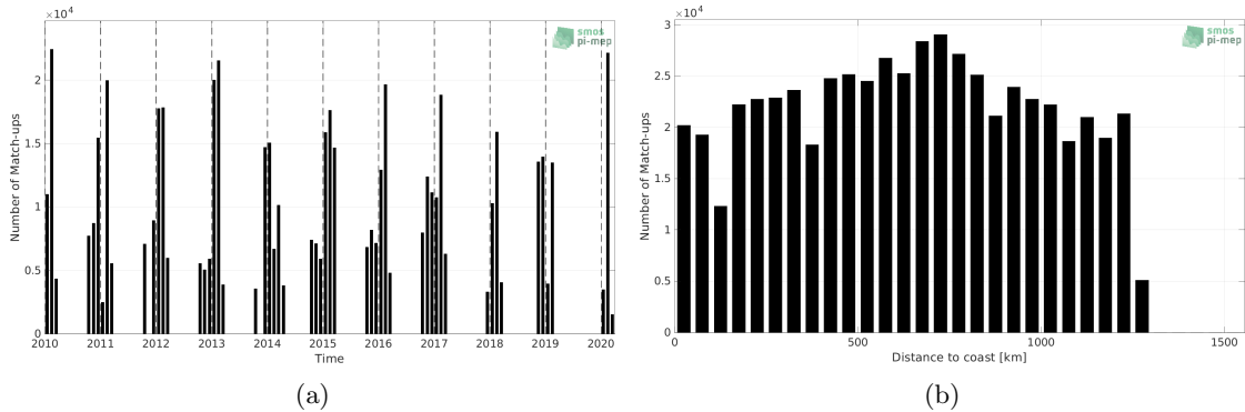
Figure 1: Number of match-ups between TSG (LEGOS-Survostral) and SMOS SSS L4 v1 - Monthly (CMEMS-CNR) SSS as a function of time (a) and as function of the distance to coast (b) over the Global Ocean Pi-MEP region and for the full satellite product period.
