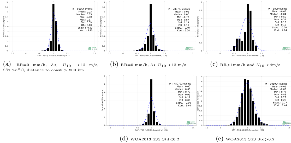
Figure 13: Normalized histogram of \Delta SSS (SMOS SSS L4 v1 - Monthly (CMEMS-CNR) - TSG (LEGOS-Survostral)) for 5 different subdatasets corresponding to: RR=0 mm/h, 3 < U_{10} < 12 m/s, SST > 5°C, distance to coast > 800 km (a), RR=0 mm/h, 3 < U_{10} < 12 m/s (b), RR > 1mm/h and U_{10} < 4 m/s (c), WOA2013 SSS Std < 0.2 (d), WOA2013 SSS Std > 0.2 (e).
