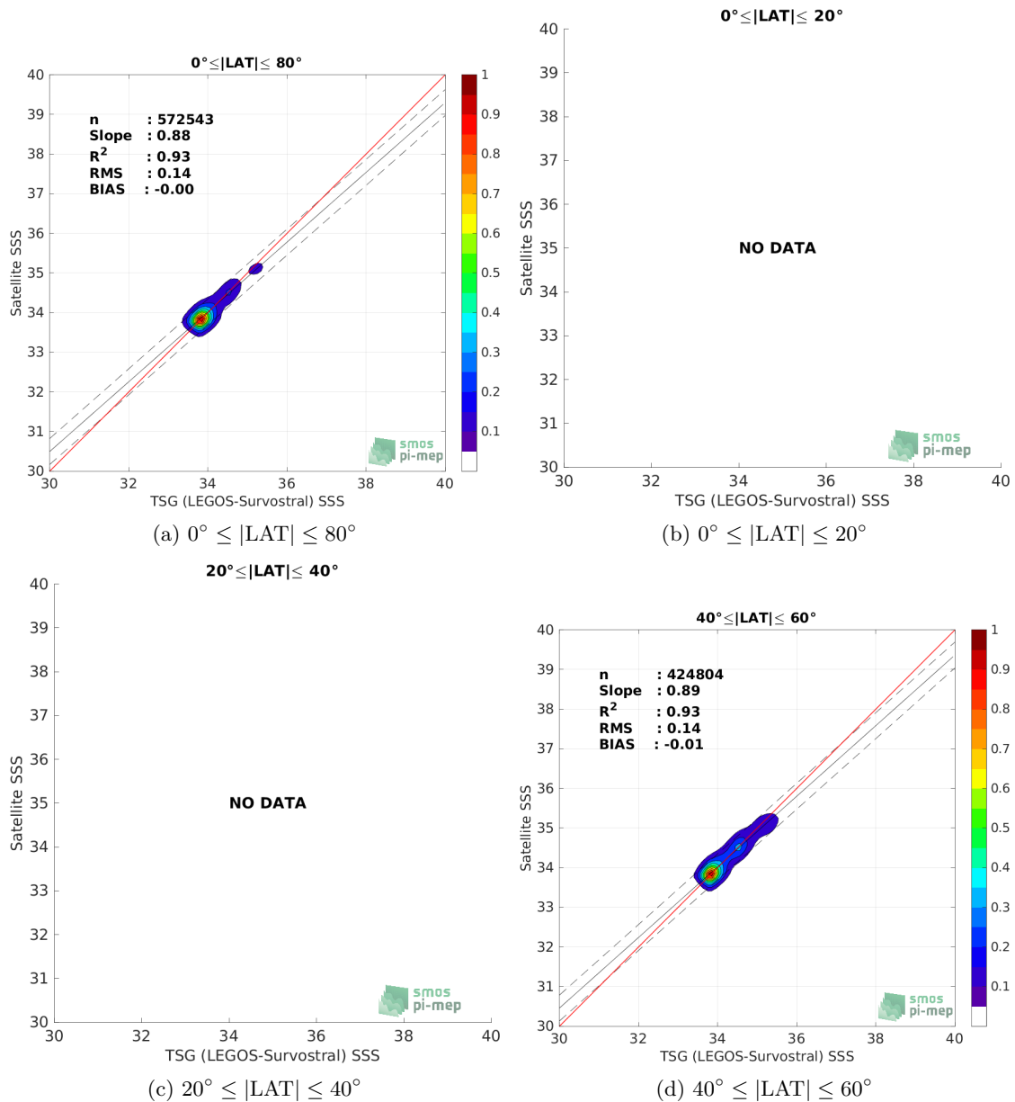
Figure 9: Contour maps of the concentration of SMOS SSS L4 v1 - Monthly (CMEMS-CNR) SSS (y-axis) versus TSG (LEGOS-Survostral) SSS (x-axis) at match-up pairs for different latitude bands. For each plot, the red line shows x=y . The black thin and dashed lines indicate a linear fit through the data cloud and the \pm 95\% confidence levels, respectively. The number match-up pairs n , the slope and R^2 coefficient of the linear fit, the root mean square (RMS) and the mean bias between satellite and in situ data are indicated for each latitude band in each plots.
