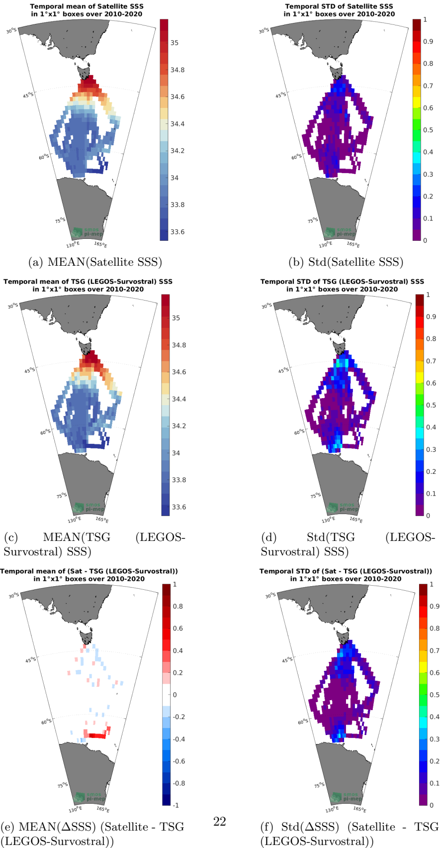
Figure 6: Temporal mean (left) and Std (right) of SSS from SMOS SSS L4 v1 - Monthly (CMEMS-CNR) (top), TSG (LEGOS-Survostral) (middle), and of \Delta SSS (Satellite - TSG (LEGOS-Survostral)). Only match-up pairs are used to generate these maps.
