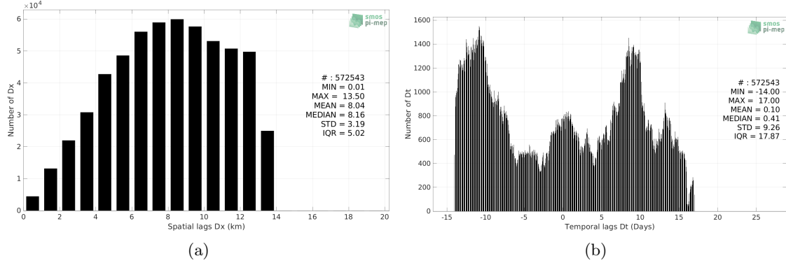
Figure 5: Histograms of the spatial (a) and temporal (b) lags between the location/time of the TSG (LEGOS-Survostral) measurement and the date of the corresponding SMOS SSS L4 v1 - Monthly (CMEMS-CNR) SSS pixel.
