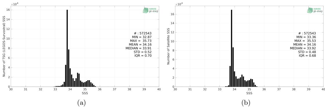
Figure 2: Histograms of SSS from TSG (LEGOS-Survostral) (a) and SMOS SSS L4 v1 - Monthly (CMEMS-CNR) (b) considering all match-up pairs per bins of 0.1 over the Global Ocean Pi-MEP region and for the full satellite product period.
