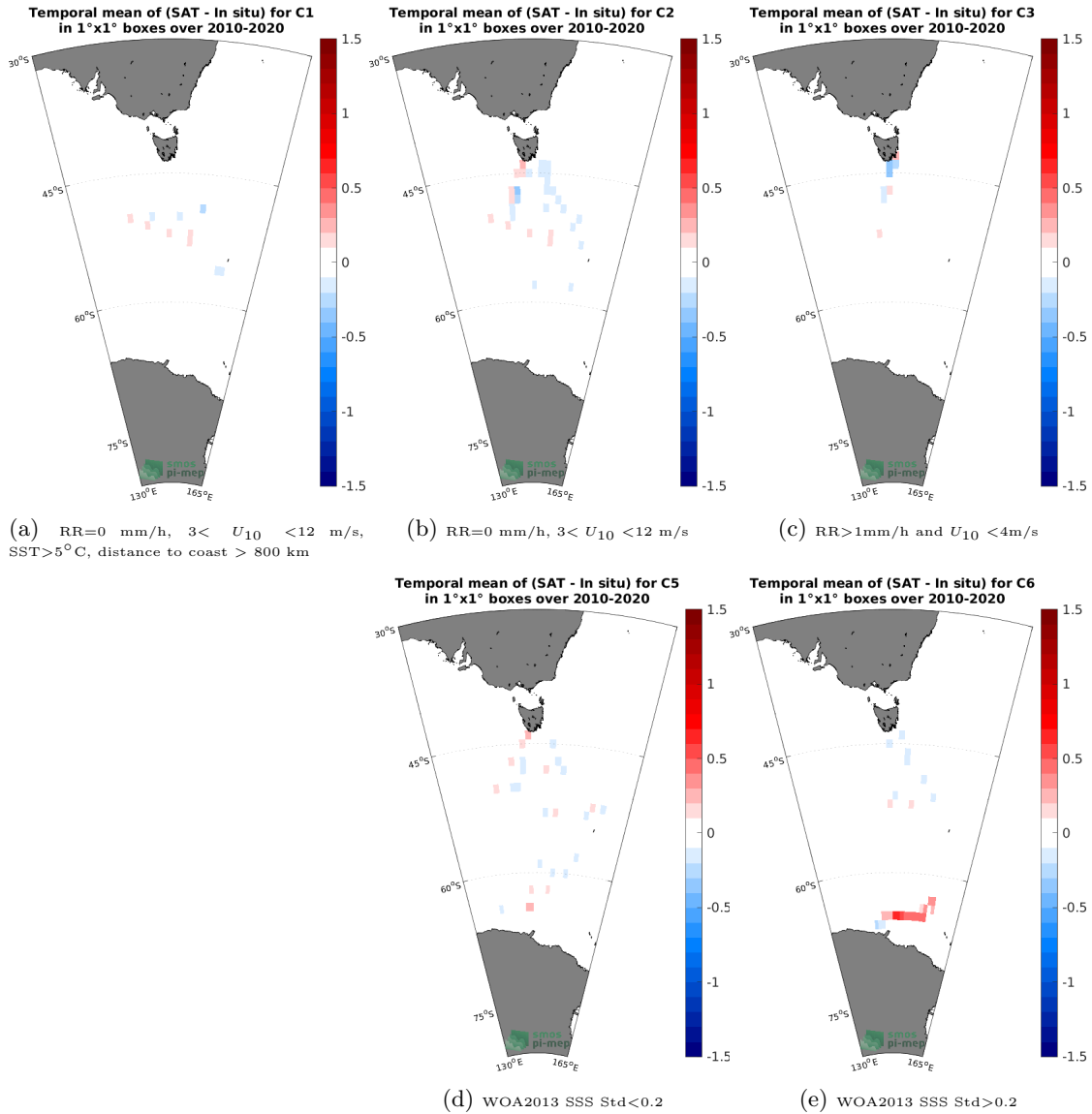
Figure 12: Temporal mean gridded over spatial boxes of size 1^\circ \times 1^\circ of \Delta SSS (SMOS SSS L4 v1 - Monthly (CMEMS-CNR) - TSG (LEGOS-Survostral)) for 5 different subdatasets corresponding to:RR=0 mm/h, 3 < U_{10} < 12 m/s, SST>5°C, distance to coast > 800 km (a), RR=0 mm/h, 3 < U_{10} < 12 m/s (b), RR>1mm/h and U_{10} < 4 m/s (c), WOA2013 SSS Std<0.2 (d), WOA2013 SSS Std>0.2 (e).
