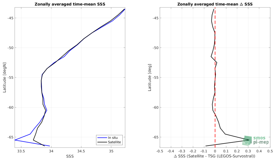
Figure 8: Left panel: Zonal mean SSS from SMOS SSS L4 v1 - Monthly (CMEMS-CNR) satellite product (black) and from TSG (LEGOS-Survostral) (blue). Right panel: Zonal mean of \Delta SSS (Satellite - TSG (LEGOS-Survostral)) for all the collected Pi-MEP match-up pairs estimated over the full satellite product period.
