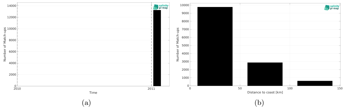
Figure 2: Number of match-ups between TSG (LEGOS-Surv-Adel) and SMOS SSS L4 v1 - Monthly (CMEMS-CNR) SSS as a function of time (a) and as function of the distance to coast (b) over the Global Ocean Pi-MEP region and for the full satellite product period.
