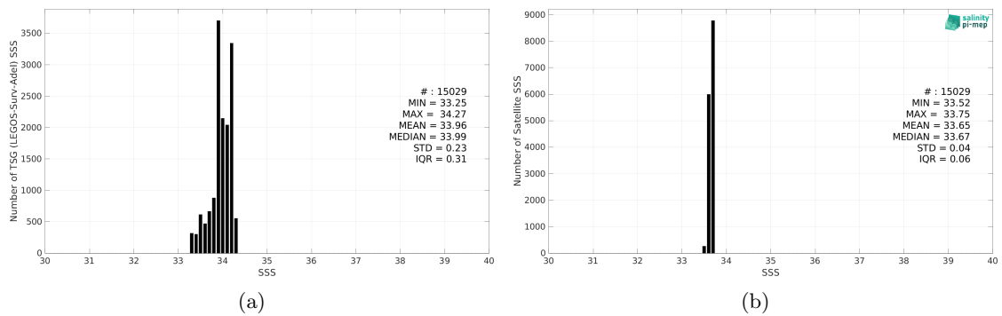
Figure 2: Histograms of SSS from TSG (LEGOS-Surv-Adel) (a) and SMOS SSS L4 v1 - Monthly (CMEMS-CNR) (b) considering all match-up pairs per bins of 0.1 over the Global Ocean Pi-MEP region and for the full satellite product period.
