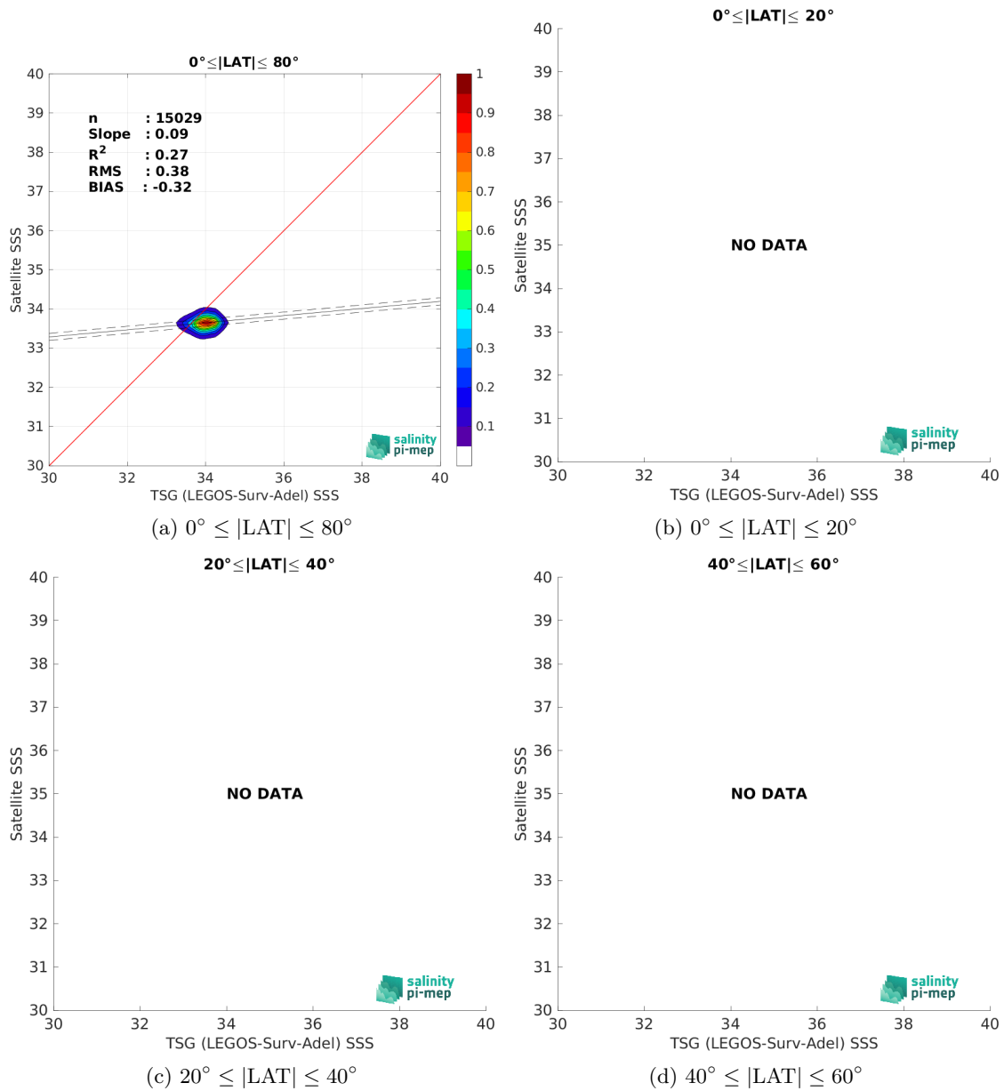
Figure 9: Contour maps of the concentration of SMOS SSS L4 v1 - Monthly (CMEMS-CNR) SSS (y-axis) versus TSG (LEGOS-Surv-Adel) SSS (x-axis) at match-up pairs for different latitude bands. For each plot, the red line shows x=y . The black thin and dashed lines indicate a linear fit through the data cloud and the \pm 95\% confidence levels, respectively. The number match-up pairs n , the slope and R^2 coefficient of the linear fit, the root mean square (RMS) and the mean bias between satellite and in situ data are indicated for each latitude band in each plots.
