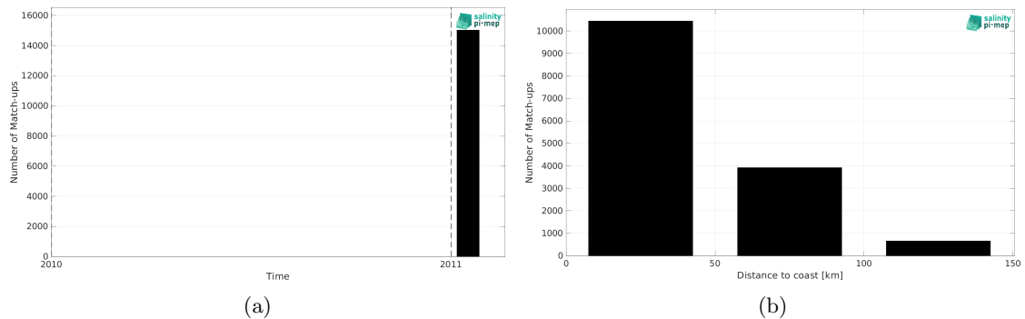
Figure 1: Number of match-ups between TSG (LEGOS-Surv-Adel) and SMOS SSS L4 v1 - Monthly (CMEMS-CNR) SSS as a function of time (a) and as function of the distance to coast (b) over the Global Ocean Pi-MEP region and for the full satellite product period.
