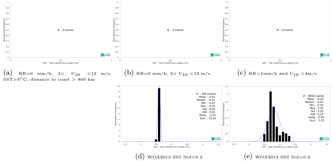
Figure 13: Normalized histogram of \Delta SSS (SMOS SSS L4 v1 - Monthly (CMEMS-CNR) - TSG (LEGOS-Surv-Adel)) for 5 different subdatasets corresponding to: RR=0 mm/h, 3 < U_{10} < 12 m/s, SST > 5°C, distance to coast > 800 km (a), RR=0 mm/h, 3 < U_{10} < 12 m/s (b), RR > 1mm/h and U_{10} < 4 m/s (c), WOA2013 SSS Std < 0.2 (d), WOA2013 SSS Std > 0.2 (e).
