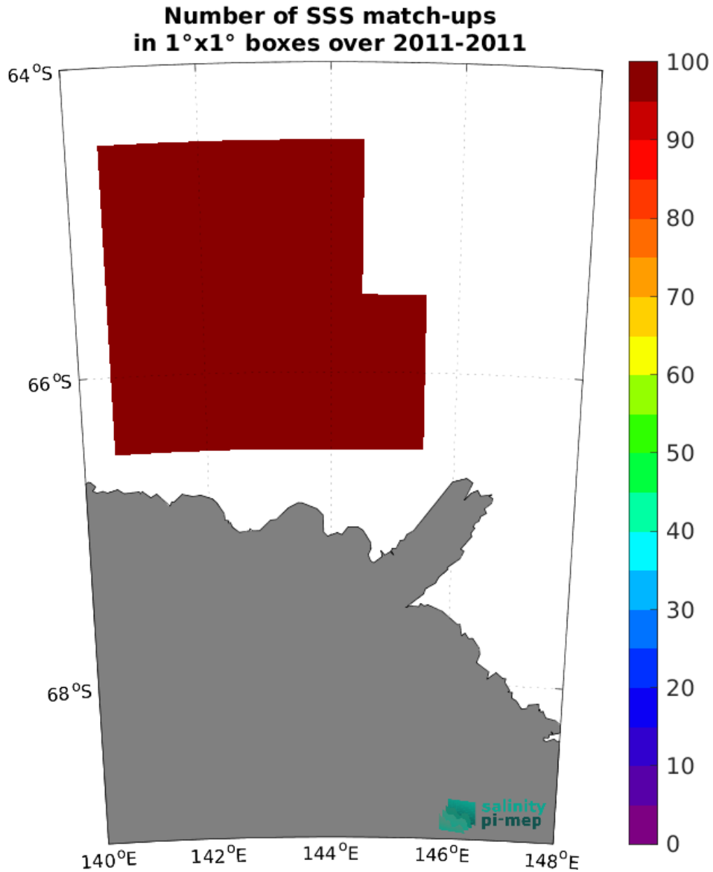
Figure 4: Number of SSS match-ups between TSG (LEGOS-Surv-Adel) SSS and the SMOS SSS L4 v1 - Monthly (CMEMS-CNR) SSS product for the Global Ocean Pi-MEP region over 1^\circ \times 1^\circ boxes and for the full satellite product period.
