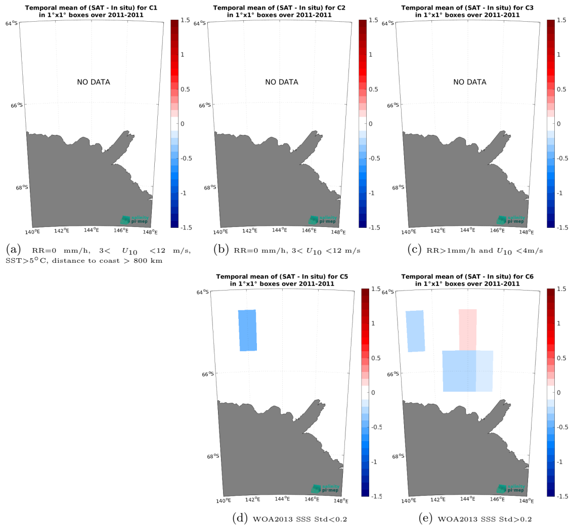
Figure 12: Temporal mean gridded over spatial boxes of size 1^\circ \times 1^\circ of \Delta SSS (SMOS SSS L4 v1 - Monthly (CMEMS-CNR) - TSG (LEGOS-Surv-Adel)) for 5 different subdatasets corresponding to: RR=0 mm/h, 3 < U_{10} < 12 m/s, SST>5°C, distance to coast > 800 km (a), RR=0 mm/h, 3 < U_{10} < 12 m/s (b), RR>1mm/h and U_{10} < 4 m/s (c), WOA2013 SSS Std<0.2 (d), WOA2013 SSS Std>0.2 (e).
