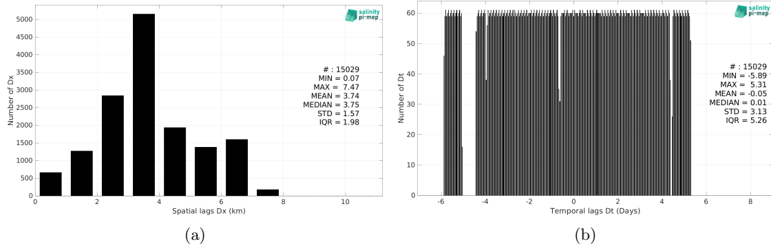
Figure 5: Histograms of the spatial (a) and temporal (b) lags between the location/time of the TSG (LEGOS-Surv-Adel) measurement and the date of the corresponding SMOS SSS L4 v1 - Monthly (CMEMS-CNR) SSS pixel.
