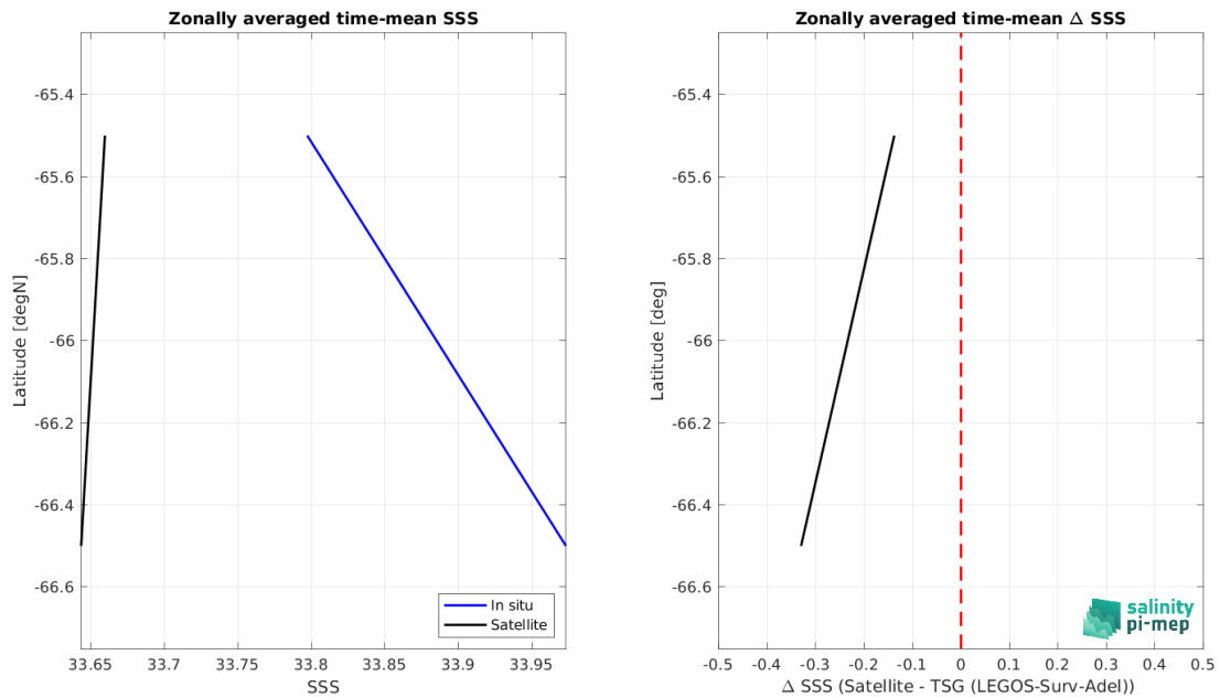
Figure 8: Left panel: Zonal mean SSS from SMOS SSS L4 v1 - Monthly (CMEMS-CNR) satellite product (black) and from TSG (LEGOS-Surv-Adel) (blue). Right panel: Zonal mean of \Delta SSS (Satellite - TSG (LEGOS-Surv-Adel)) for all the collected Pi-MEP match-up pairs estimated over the full satellite product period.
