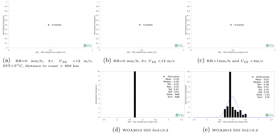
Figure 13: Normalized histogram of \Delta SSS (SMOS SSS L4 v1 - Monthly (CMEMS-CNR) - TSG (LEGOS-Surv-Adel)) for 5 different subdatasets corresponding to: RR=0 mm/h, 3 < U_{10} < 12 m/s, SST > 5°C, distance to coast > 800 km (a), RR=0 mm/h, 3 < U_{10} < 12 m/s (b), RR > 1mm/h and U_{10} < 4 m/s (c), WOA2013 SSS Std < 0.2 (d), WOA2013 SSS Std > 0.2 (e).
