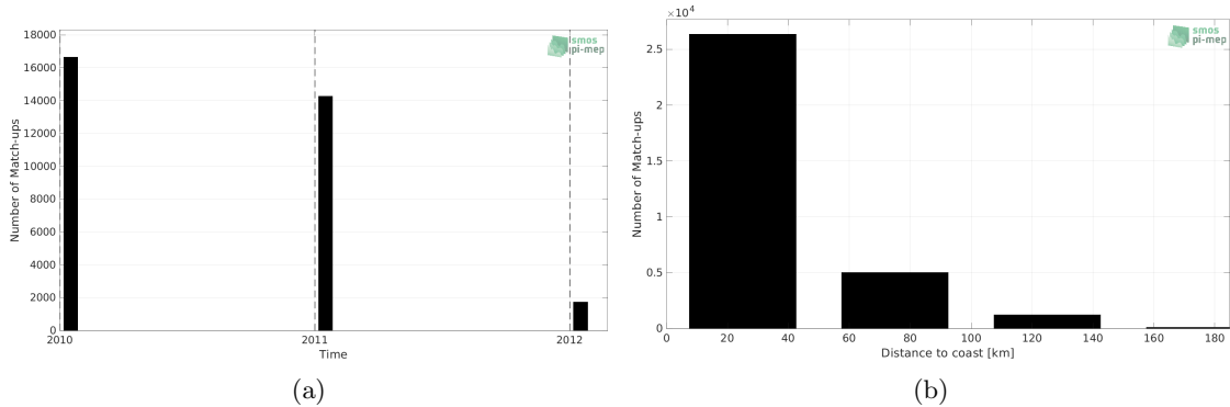
Figure 1: Number of match-ups between TSG (LEGOS-Surv-Adel) and SMOS SSS L4 v1 - Monthly (CMEMS-CNR) SSS as a function of time (a) and as function of the distance to coast (b) over the Global Ocean Pi-MEP region and for the full satellite product period.
