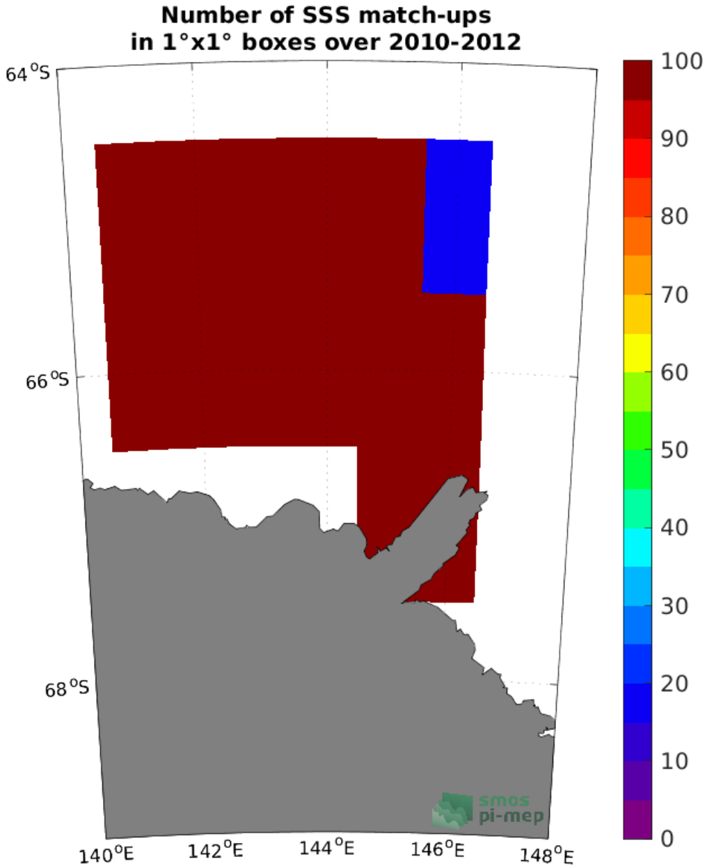
Figure 4: Number of SSS match-ups between TSG (LEGOS-Surv-Adel) SSS and the SMOS SSS L4 v1 - Monthly (CMEMS-CNR) SSS product for the Global Ocean Pi-MEP region over 1°x1° boxes and for the full satellite product period.
