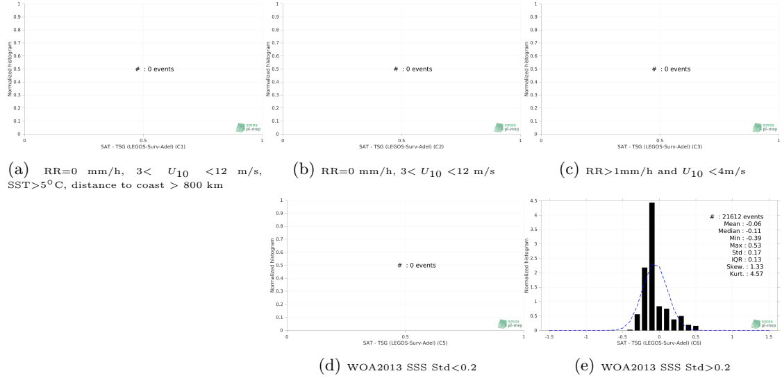
Figure 13: Normalized histogram of \Delta SSS (SMOS SSS L4 v1 - Monthly (CMEMS-CNR) - TSG (LEGOS-Surv-Adel)) for 5 different subdatasets corresponding to: RR=0 mm/h, 3 < U_{10} < 12 m/s, SST >5^{\circ} C, distance to coast > 800 km (a), RR=0 mm/h, 3 < U_{10} < 12 m/s (b), RR >1 mm/h and U_{10} < 4 m/s (c), WOA2013 SSS Std <0.2 (d), WOA2013 SSS Std >0.2 (e).
