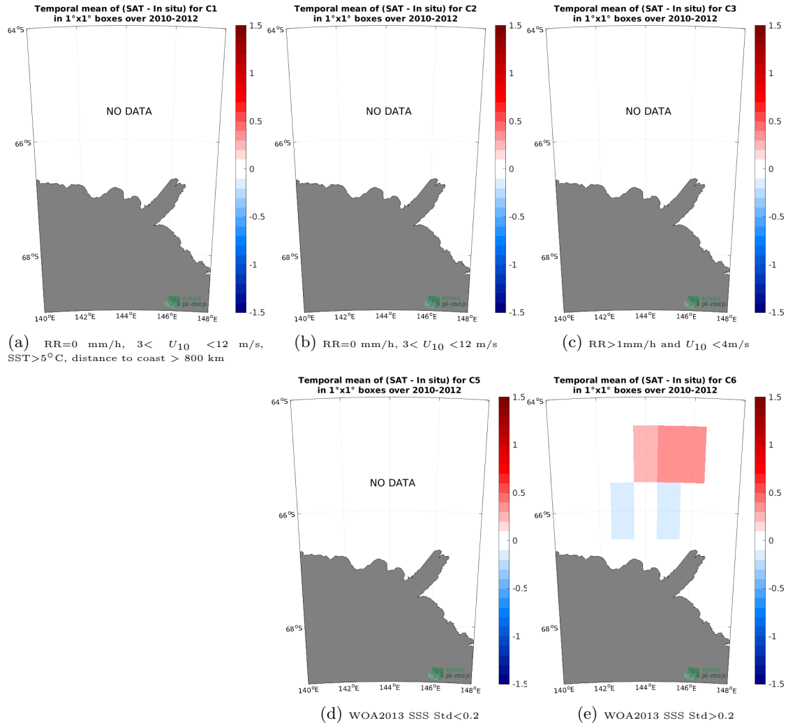
Figure 12: Temporal mean gridded over spatial boxes of size 1°×1° of \Delta SSS (SMOS SSS L4 v1 - Monthly (CMEMS-CNR) - TSG (LEGOS-Surv-Adel)) for 5 different subdatasets corresponding to: RR=0 mm/h, 3 < U_{10} < 12 m/s, SST>5°C, distance to coast > 800 km (a), RR=0 mm/h, 3 < U_{10} < 12 m/s (b), RR>1mm/h and U_{10} < 4 m/s (c), WOA2013 SSS Std<0.2 (d), WOA2013 SSS Std>0.2 (e).
