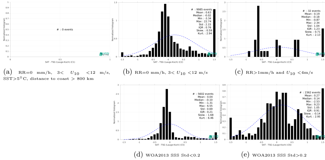
Figure 15: Normalized histogram of \Delta SSS (SMOS SSS L4 v1 - Monthly (CMEMS-CNR) - TSG (Laugue-Koch)) for 5 different subdatasets corresponding to: RR=0 mm/h, 3 < U_{10} < 12 m/s, SST > 5°C, distance to coast > 800 km (a), RR=0 mm/h, 3 < U_{10} < 12 m/s (b), RR > 1mm/h and U_{10} < 4 m/s (c), WOA2013 SSS Std < 0.2 (d), WOA2013 SSS Std > 0.2 (e).
