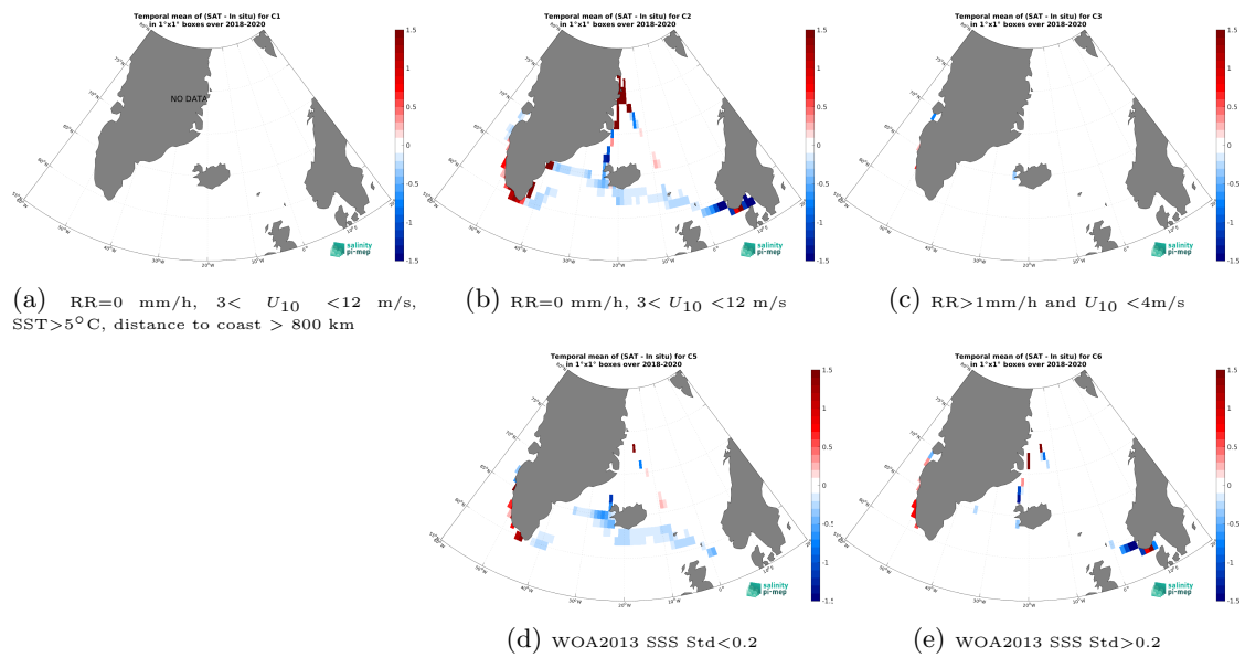
Figure 14: Temporal mean gridded over spatial boxes of size 1^\circ \times 1^\circ of \Delta SSS (SMOS SSS L4 v1 - Monthly (CMEMS-CNR) - TSG (Lauge-Koch)) for 5 different subdatasets corresponding to:RR=0 mm/h, 3 < U_{10} < 12 m/s, SST >5^\circ C, distance to coast > 800 km (a), RR=0 mm/h, 3 < U_{10} < 12 m/s (b), RR >1 mm/h and U_{10} < 4 m/s (c), WOA2013 SSS Std <0.2 (d), WOA2013 SSS Std >0.2 (e).
