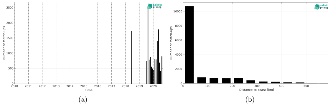
Figure 2: Number of match-ups between TSG (Lauge-Koch) and SMOS SSS L4 v1 - Monthly (CMEMS-CNR) SSS as a function of time (a) and as function of the distance to coast (b) over the Global Ocean Pi-MEP region and for the full satellite product period.
