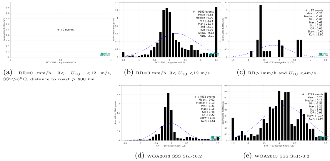
Figure 15: Normalized histogram of \Delta SSS (SMOS SSS L4 v1 - Monthly (CMEMS-CNR) - TSG (Lauge-Koch)) for 5 different subdatasets corresponding to: RR=0 mm/h, 3 < U_{10} < 12 m/s, SST>5°C, distance to coast > 800 km (a), RR=0 mm/h, 3 < U_{10} < 12 m/s (b), RR>1mm/h and U_{10} < 4 m/s (c), WOA2013 SSS Std<0.2 (d), WOA2013 SSS Std>0.2 (e).
