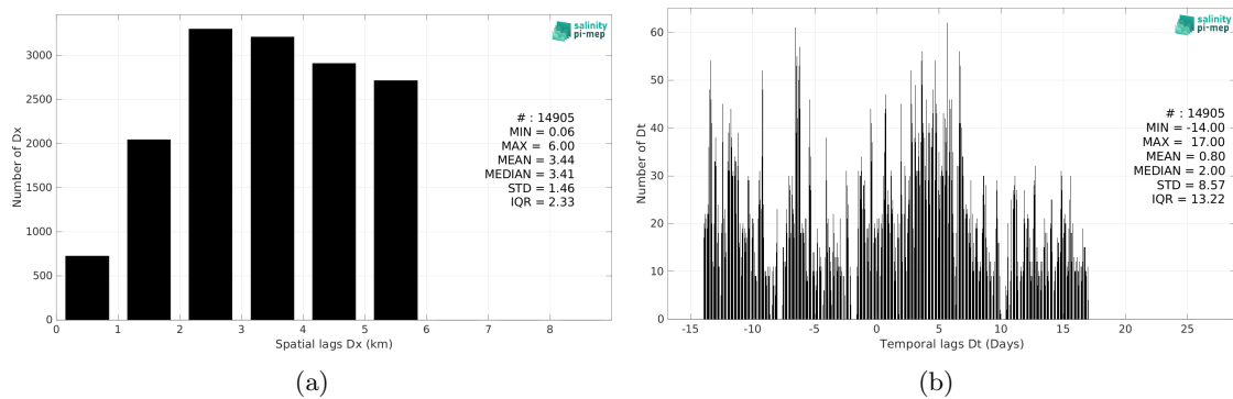
Figure 6: Histograms of the spatial (a) and temporal (b) lags between the location/time of the TSG (Lauge-Koch) measurement and the date of the corresponding SMOS SSS L4 v1 - Monthly (CMEMS-CNR) SSS pixel.
