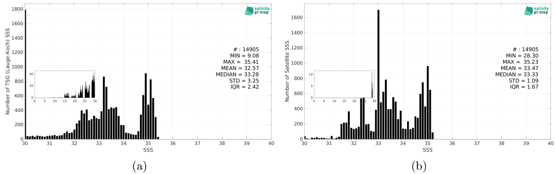
Figure 3: Histograms of SSS from TSG (Lauge-Koch) (a) and SMOS SSS L4 v1 - Monthly (CMEMS-CNR) (b) considering all match-up pairs per bins of 0.1 over the Global Ocean Pi-MEP region and for the full satellite product period.
