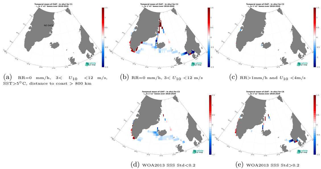
Figure 14: Temporal mean gridded over spatial boxes of size 1^\circ \times 1^\circ of \Delta\text{SSS} (SMOS SSS L4 v1 - Monthly (CMEMS-CNR) - TSG (Lauge-Koch)) for 5 different subdatasets corresponding to: RR=0 mm/h, 3 < U_{10} < 12 m/s, SST > 5^\circ\text{C} , distance to coast > 800 km (a), RR=0 mm/h, 3 < U_{10} < 12 m/s (b), RR > 1 mm/h and U_{10} < 4 m/s (c), WOA2013 SSS Std < 0.2 (d), WOA2013 SSS Std > 0.2 (e).
