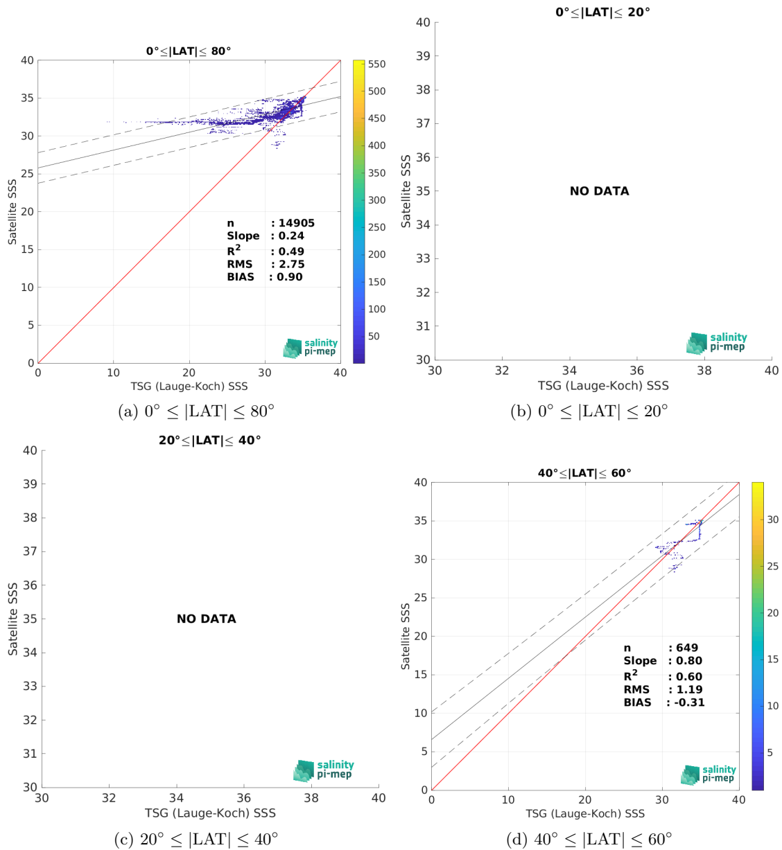
Figure 10: Contour maps of the concentration of SMOS SSS L4 v1 - Monthly (CMEMS-CNR) SSS (y-axis) versus TSG (Lauge-Koch) SSS (x-axis) at match-up pairs for different latitude bands. For each plot, the red line shows x=y . The black thin and dashed lines indicate a linear fit through the data cloud and the \pm 95\% confidence levels, respectively. The number match-up pairs n , the slope and R^2 coefficient of the linear fit, the root mean square (RMS) and the mean bias between satellite and in situ data are indicated for each latitude band in each plots.
