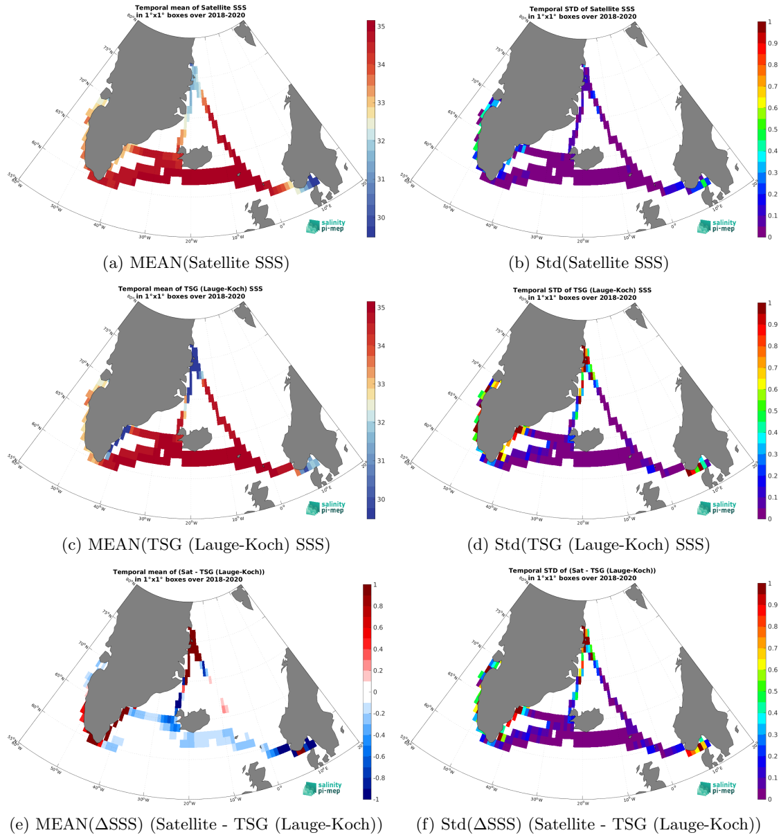
Figure 7: Temporal mean (left) and Std (right) of SSS from SMOS SSS L4 v1 - Monthly (CMEMS-CNR) (top), TSG (Lauge-Koch) (middle), and of \Delta SSS (Satellite - TSG (Lauge-Koch)). Only match-up pairs are used to generate these maps.
