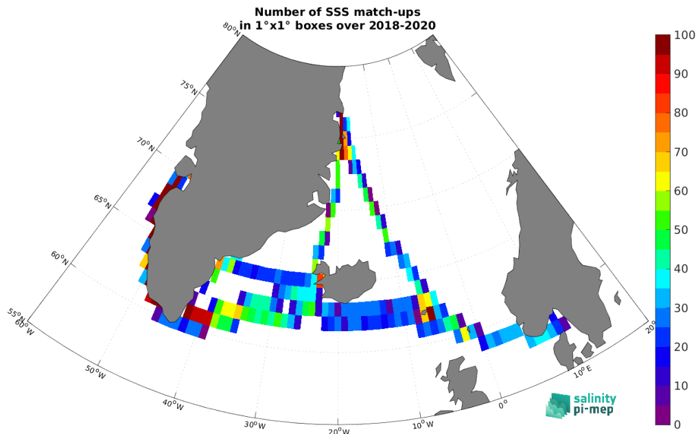
Figure 5: Number of SSS match-ups between TSG (Lauge-Koch) SSS and the SMOS SSS L4 v1 - Monthly (CMEMS-CNR) SSS product for the Global Ocean Pi-MEP region over 1^\circ \times 1^\circ boxes and for the full satellite product period.
