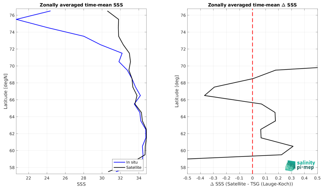
Figure 9: Left panel: Zonal mean SSS from SMOS SSS L4 v1 - Monthly (CMEMS-CNR) satellite product (black) and from TSG (Lauge-Koch) (blue). Right panel: Zonal mean of \Delta SSS (Satellite - TSG (Lauge-Koch)) for all the collected Pi-MEP match-up pairs estimated over the full satellite product period.
