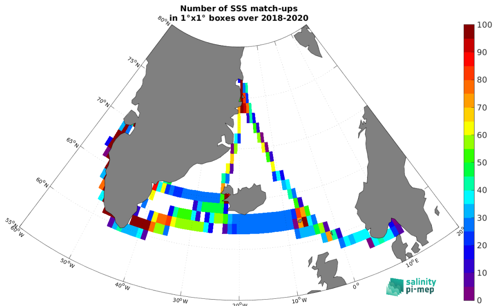
Figure 4: Number of SSS match-ups between TSG (Lauge-Koch) SSS and the SMOS SSS L4 v1 - Monthly (CMEMS-CNR) SSS product for the Global Ocean Pi-MEP region over 1^\circ \times 1^\circ boxes and for the full satellite product period.
