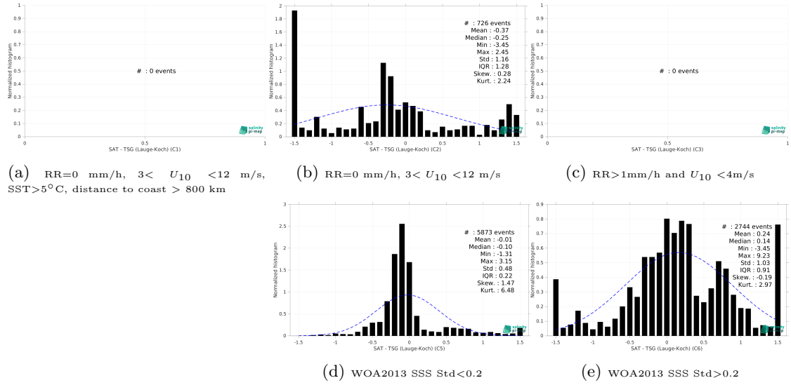
Figure 13: Normalized histogram of \Delta SSS (SMOS SSS L4 v1 - Monthly (CMEMS-CNR) - TSG (Lauge-Koch)) for 5 different subdatasets corresponding to: RR=0 mm/h, 3 < U_{10} < 12 m/s, SST > 5°C, distance to coast > 800 km (a), RR=0 mm/h, 3 < U_{10} < 12 m/s (b), RR > 1mm/h and U_{10} < 4 m/s (c), WOA2013 SSS Std < 0.2 (d), WOA2013 SSS Std > 0.2 (e).
