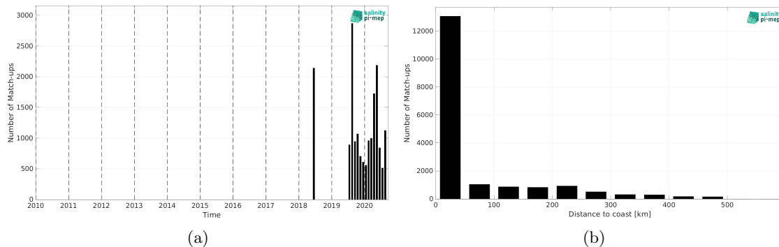
Figure 1: Number of match-ups between TSG (Lauge-Koch) and SMOS SSS L4 v1 - Monthly (CMEMS-CNR) SSS as a function of time (a) and as function of the distance to coast (b) over the Global Ocean Pi-MEP region and for the full satellite product period.
