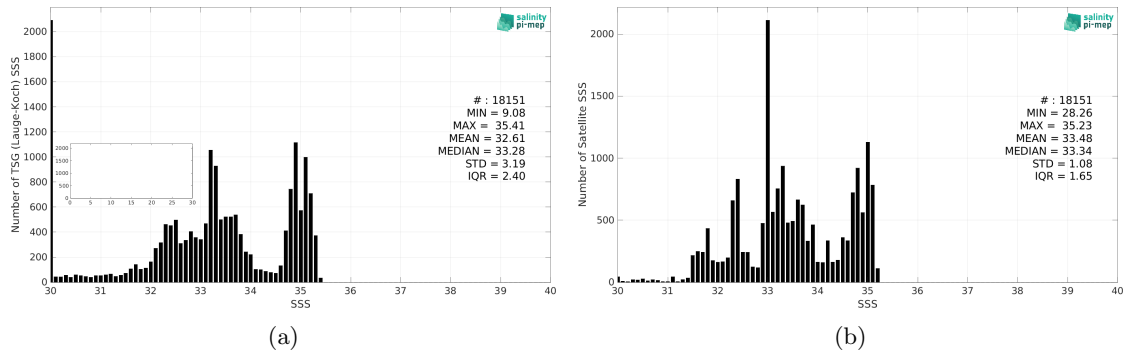
Figure 2: Histograms of SSS from TSG (Lauge-Koch) (a) and SMOS SSS L4 v1 - Monthly (CMEMS-CNR) (b) considering all match-up pairs per bins of 0.1 over the Global Ocean Pi-MEP region and for the full satellite product period.
