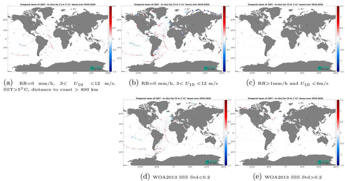
Figure 14: Temporal mean gridded over spatial boxes of size 1^\circ \times 1^\circ of \Delta\text{SSS} (SMOS SSS L4 v1 - Monthly (CMEMS-CNR) - TSG (GOSUD-Sailing-ship)) for 5 different subdatasets corresponding to:RR=0 mm/h, 3 < U_{10} < 12 m/s, SST >5^\circ\text{C} , distance to coast > 800 km (a), RR=0 mm/h, 3 < U_{10} < 12 m/s (b), RR >1 mm/h and U_{10} < 4 m/s (c), WOA2013 SSS Std <0.2 (d), WOA2013 SSS Std >0.2 (e).
