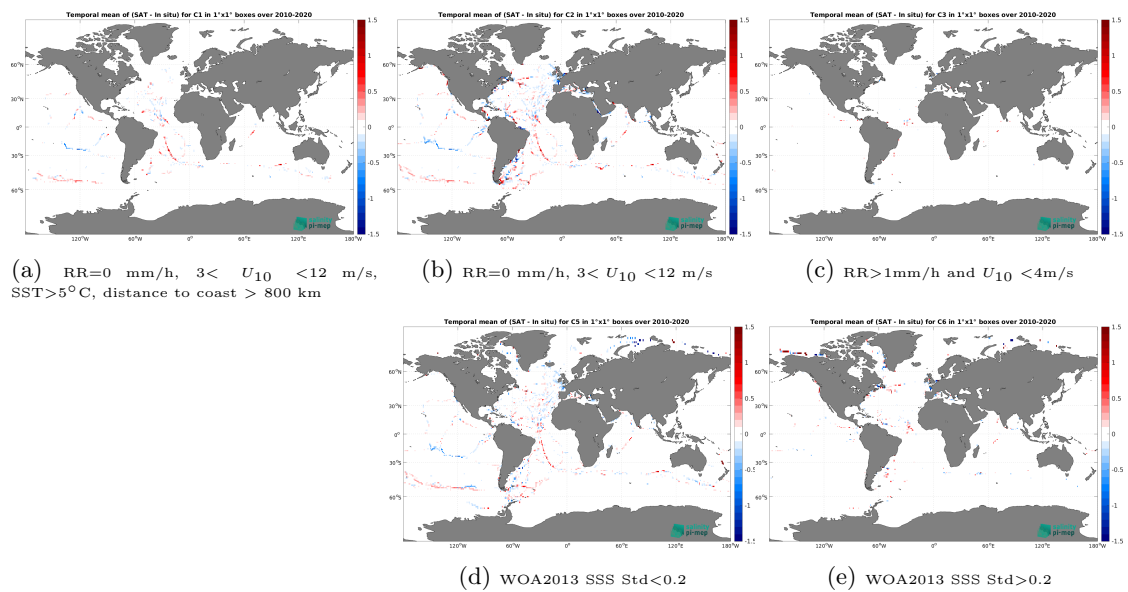
Figure 12: Temporal mean gridded over spatial boxes of size 1^\circ \times 1^\circ of \Delta\text{SSS} (SMOS SSS L4 v1 - Monthly (CMEMS-CNR) - TSG (GOSUD-Sailing-ship)) for 5 different subdatasets corresponding to:RR=0 mm/h, 3 < U_{10} < 12 m/s, SST >5^\circ\text{C} , distance to coast > 800 km (a), RR=0 mm/h, 3 < U_{10} < 12 m/s (b), RR >1 mm/h and U_{10} < 4 m/s (c), WOA2013 SSS Std <0.2 (d), WOA2013 SSS Std >0.2 (e).
