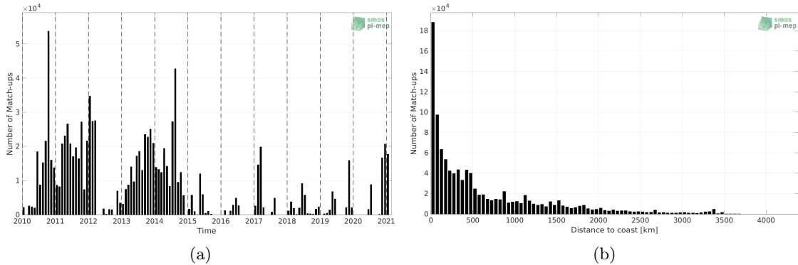
Figure 1: Number of match-ups between TSG (GOSUD-Sailing-ship) and SMOS SSS L4 v1 - Monthly (CMEMS-CNR) SSS as a function of time (a) and as function of the distance to coast (b) over the Global Ocean Pi-MEP region and for the full satellite product period.
