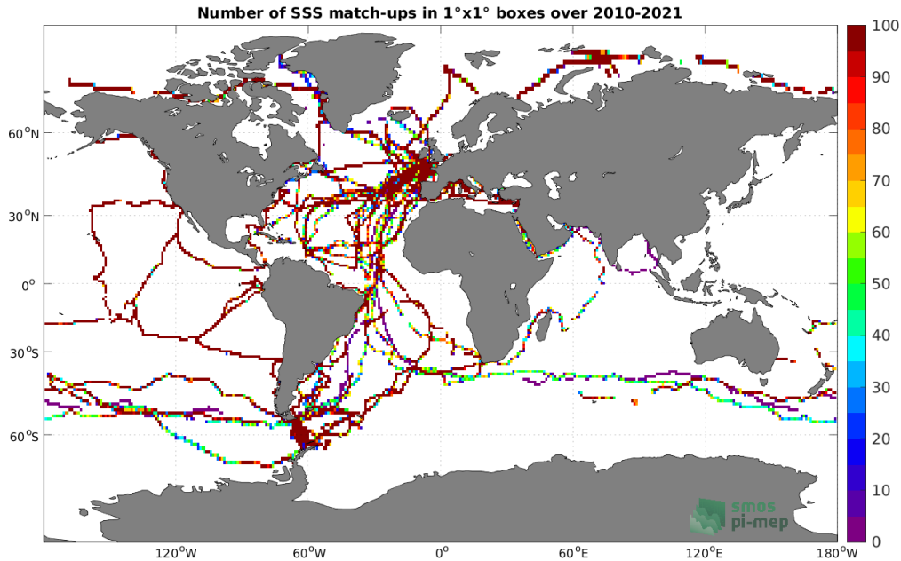
Figure 4: Number of SSS match-ups between TSG (GOSUD-Sailing-ship) SSS and the SMOS SSS L4 v1 - Monthly (CMEMS-CNR) SSS product for the Global Ocean Pi-MEP region over 1^\circ \times 1^\circ boxes and for the full satellite product period.
