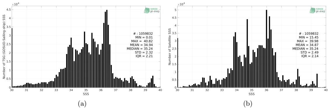
Figure 2: Histograms of SSS from TSG (GOSUD-Sailing-ship) (a) and SMOS SSS L4 v1 - Monthly (CMEMS-CNR) (b) considering all match-up pairs per bins of 0.1 over the Global Ocean Pi-MEP region and for the full satellite product period.
