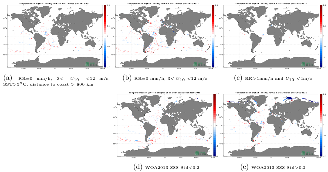
Figure 12: Temporal mean gridded over spatial boxes of size 1^\circ \times 1^\circ of \Delta SSS (SMOS SSS L4 v1 - Monthly (CMEMS-CNR) - TSG (GOSUD-Sailing-ship)) for 5 different subdatasets corresponding to:RR=0 mm/h, 3 < U_{10} < 12 m/s, SST > 5°C, distance to coast > 800 km (a), RR=0 mm/h, 3 < U_{10} < 12 m/s (b), RR > 1mm/h and U_{10} < 4 m/s (c), WOA2013 SSS Std < 0.2 (d), WOA2013 SSS Std > 0.2 (e).
