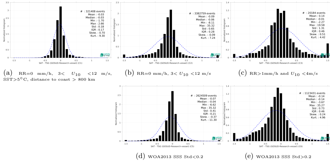
Figure 15: Normalized histogram of \Delta SSS (SMOS SSS L4 v1 - Monthly (CMEMS-CNR) - TSG (GOSUD-Research-vessel)) for 5 different subdatasets corresponding to: RR=0 mm/h, 3 < U_{10} < 12 m/s, SST > 5°C, distance to coast > 800 km (a), RR=0 mm/h, 3 < U_{10} < 12 m/s (b), RR > 1mm/h and U_{10} < 4 m/s (c), WOA2013 SSS Std < 0.2 (d), WOA2013 SSS Std > 0.2 (e).
