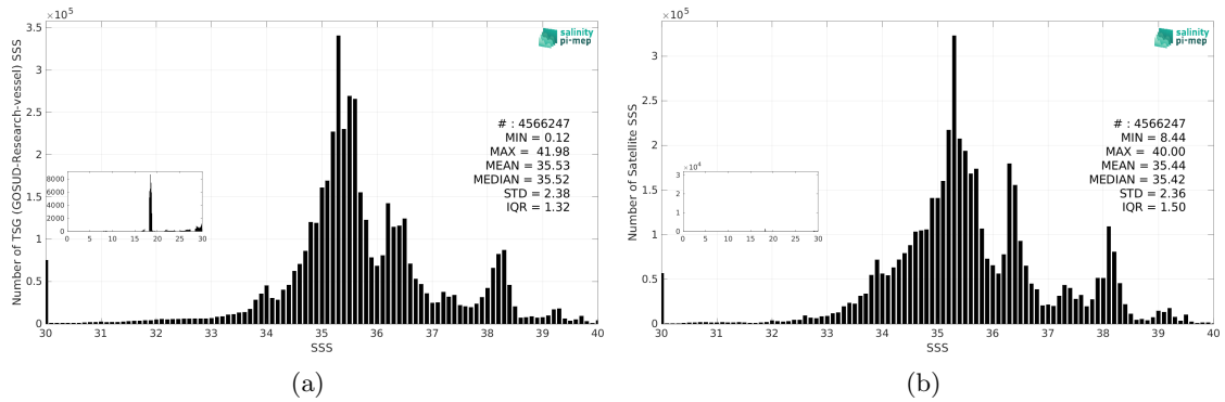
Figure 3: Histograms of SSS from TSG (GOSUD-Research-vessel) (a) and SMOS SSS L4 v1 - Monthly (CMEMS-CNR) (b) considering all match-up pairs per bins of 0.1 over the Global Ocean Pi-MEP region and for the full satellite product period.
