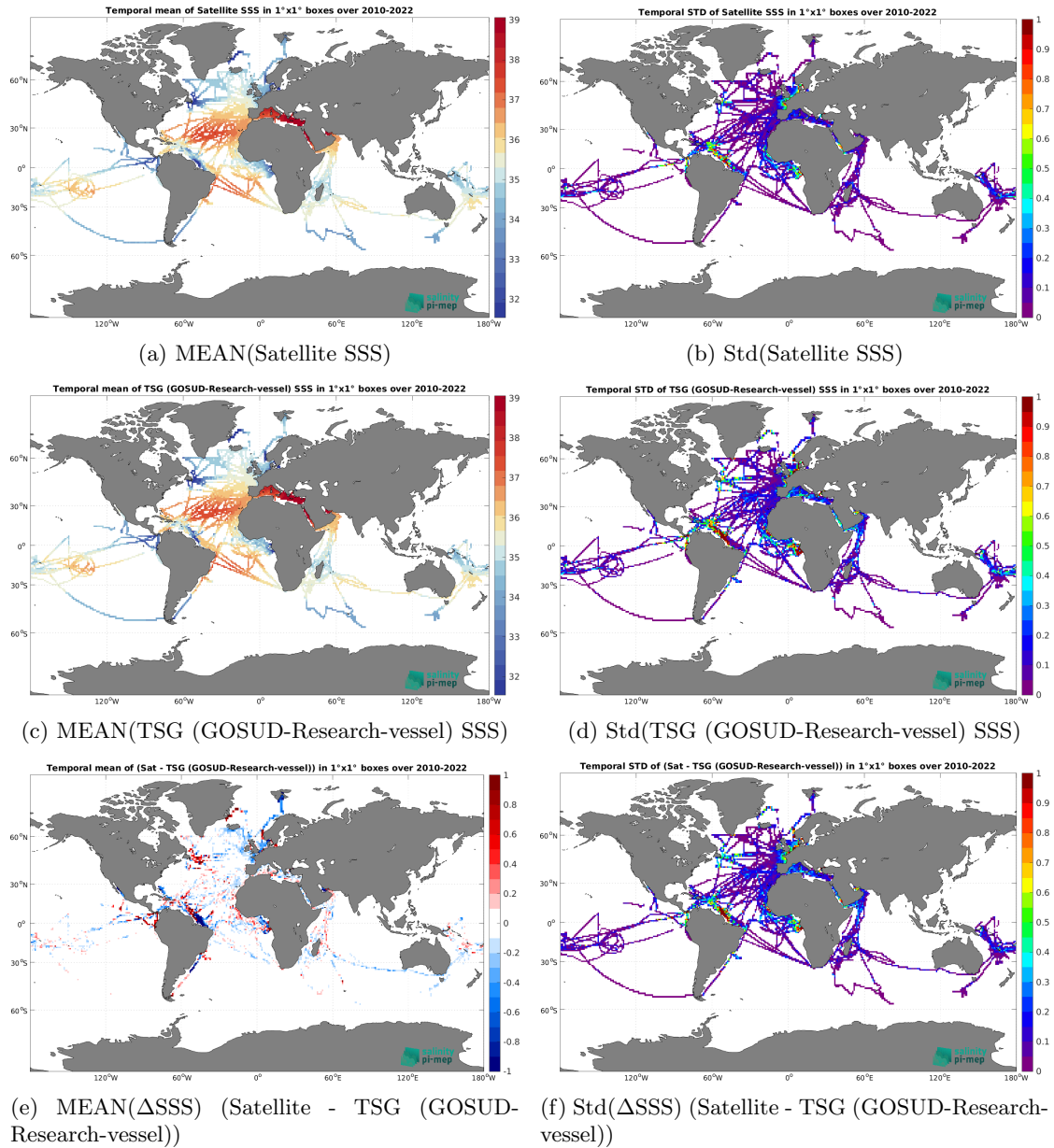
Figure 7: Temporal mean (left) and Std (right) of SSS from SMOS SSS L4 v1 - Monthly (CMEMS-CNR) (top), TSG (GOSUD-Research-vessel) (middle), and of \Delta SSS (Satellite - TSG (GOSUD-Research-vessel)). Only match-up pairs are used to generate these maps.
