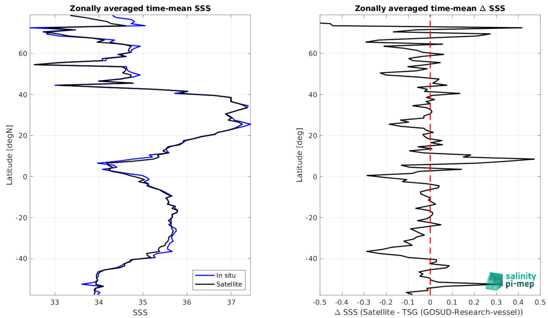
Figure 9: Left panel: Zonal mean SSS from SMOS SSS L4 v1 - Monthly (CMEMS-CNR) satellite product (black) and from TSG (GOSUD-Research-vessel) (blue). Right panel: Zonal mean of \Delta SSS (Satellite - TSG (GOSUD-Research-vessel)) for all the collected Pi-MEP match-up pairs estimated over the full satellite product period.
