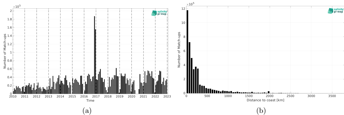
Figure 2: Number of match-ups between TSG (GOSUD-Research-vessel) and SMOS SSS L4 v1 - Monthly (CMEMS-CNR) SSS as a function of time (a) and as function of the distance to coast (b) over the Global Ocean Pi-MEP region and for the full satellite product period.
