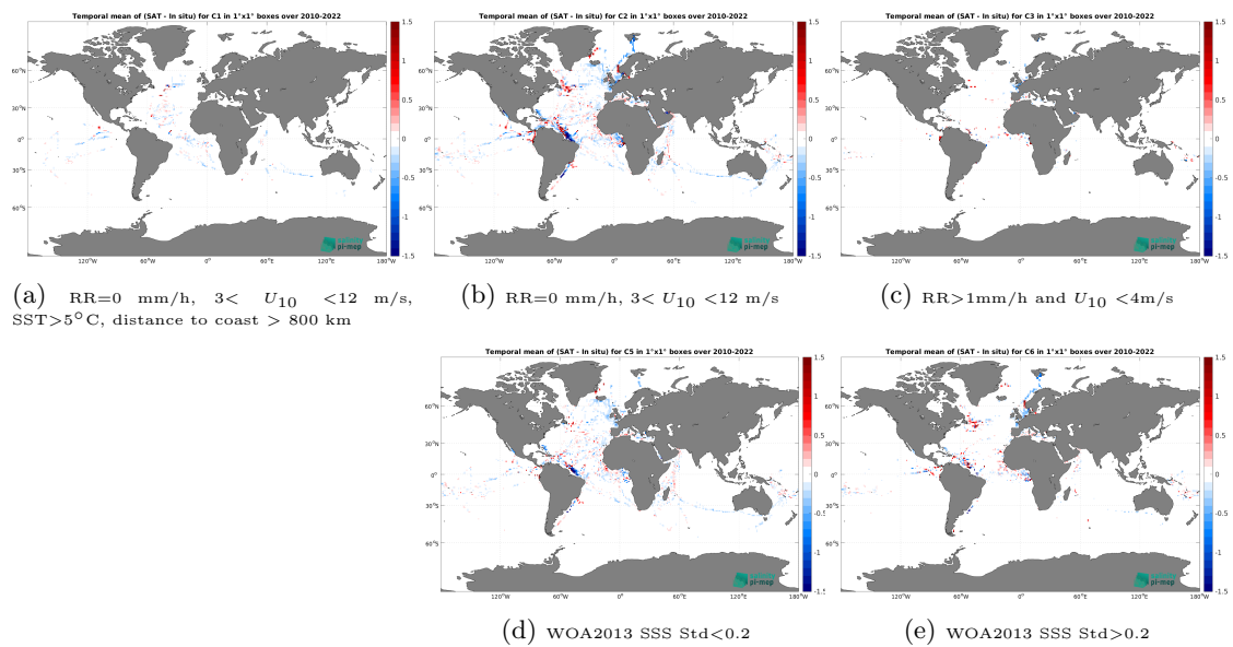
Figure 14: Temporal mean gridded over spatial boxes of size 1^\circ \times 1^\circ of \Delta SSS (SMOS SSS L4 v1 - Monthly (CMEMS-CNR) - TSG (GOSUD-Research-vessel)) for 5 different subdatasets corresponding to: RR=0 mm/h, 3 < U_{10} < 12 m/s, SST > 5°C, distance to coast > 800 km (a), RR=0 mm/h, 3 < U_{10} < 12 m/s (b), RR > 1mm/h and U_{10} < 4 m/s (c), WOA2013 SSS Std < 0.2 (d), WOA2013 SSS Std > 0.2 (e).
