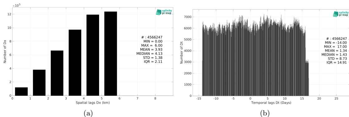
Figure 6: Histograms of the spatial (a) and temporal (b) lags between the location/time of the TSG (GOSUD-Research-vessel) measurement and the date of the corresponding SMOS SSS L4 v1 - Monthly (CMEMS-CNR) SSS pixel.
