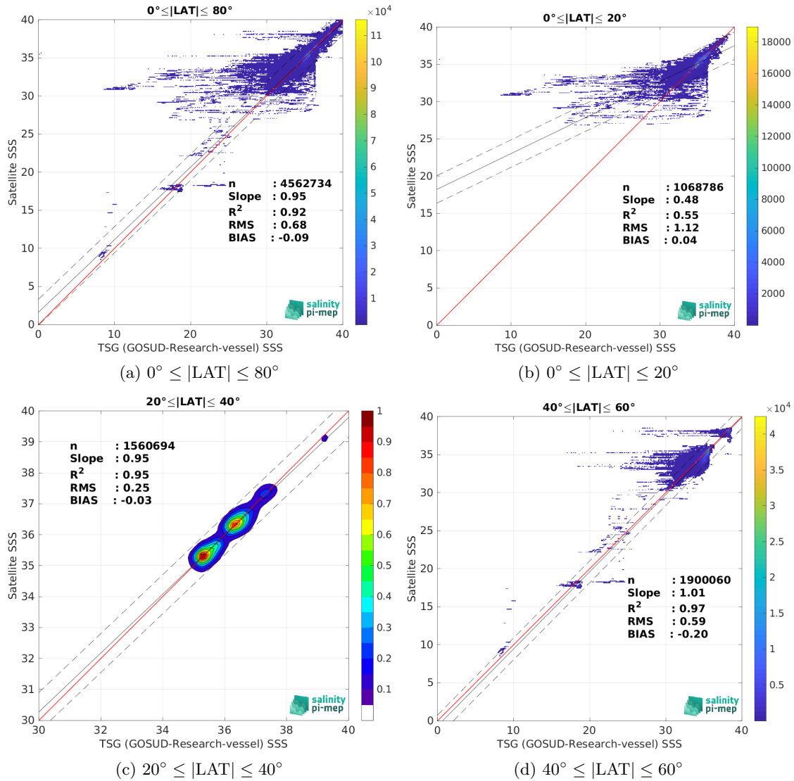
Figure 10: Contour maps of the concentration of SMOS SSS L4 v1 - Monthly (CMEMS-CNR) SSS (y-axis) versus TSG (GOSUD-Research-vessel) SSS (x-axis) at match-up pairs for different latitude bands. For each plot, the red line shows x=y . The black thin and dashed lines indicate a linear fit through the data cloud and the \pm 95\% confidence levels, respectively. The number match-up pairs n , the slope and R^2 coefficient of the linear fit, the root mean square (RMS) and the mean bias between satellite and in situ data are indicated for each latitude band in each plots.
