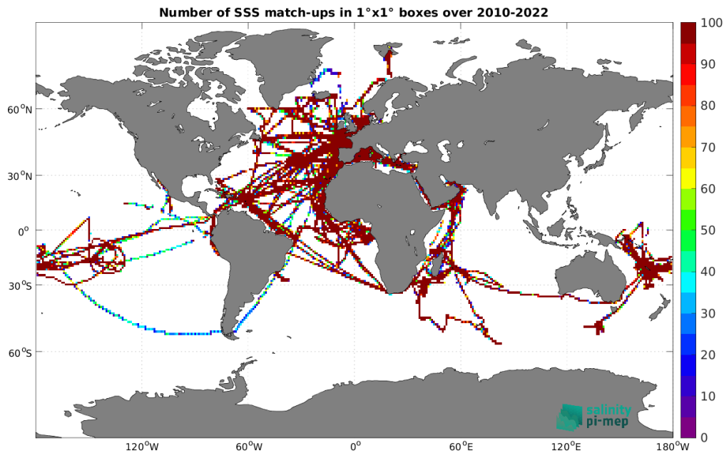
Figure 5: Number of SSS match-ups between TSG (GOSUD-Research-vessel) SSS and the SMOS SSS L4 v1 - Monthly (CMEMS-CNR) SSS product for the Global Ocean Pi-MEP region over 1^\circ \times 1^\circ boxes and for the full satellite product period.
