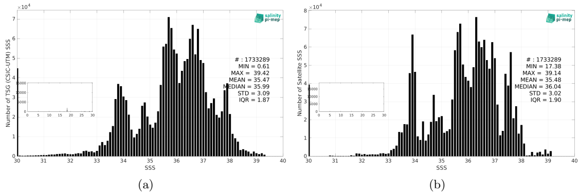
Figure 3: Histograms of SSS from TSG (CSIC-UTM) (a) and SMOS SSS L4 v1 - Monthly (CMEMS-CNR) (b) considering all match-up pairs per bins of 0.1 over the Global Ocean Pi-MEP region and for the full satellite product period.
