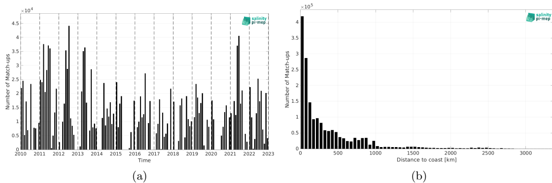
Figure 2: Number of match-ups between TSG (CSIC-UTM) and SMOS SSS L4 v1 - Monthly (CMEMS-CNR) SSS as a function of time (a) and as function of the distance to coast (b) over the Global Ocean Pi-MEP region and for the full satellite product period.
