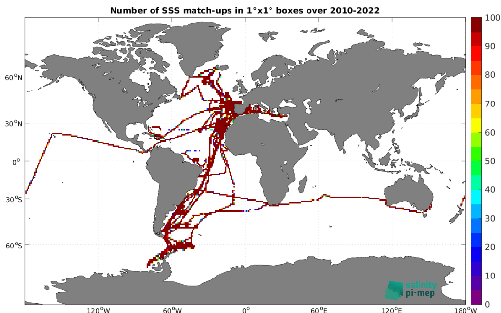
Figure 5: Number of SSS match-ups between TSG (CSIC-UTM) SSS and the SMOS SSS L4 v1 - Monthly (CMEMS-CNR) SSS product for the Global Ocean Pi-MEP region over 1^\circ \times 1^\circ boxes and for the full satellite product period.
