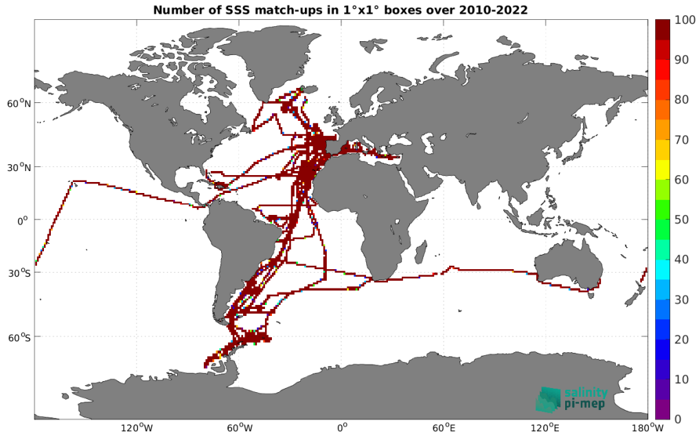
Figure 4: Number of SSS match-ups between TSG (CSIC-UTM) SSS and the SMOS SSS L4 v1 - Monthly (CMEMS-CNR) SSS product for the Global Ocean Pi-MEP region over 1°x1° boxes and for the full satellite product period.
