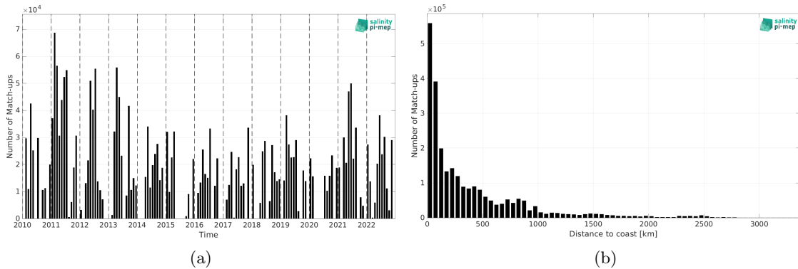
Figure 1: Number of match-ups between TSG (CSIC-UTM) and SMOS SSS L4 v1 - Monthly (CMEMS-CNR) SSS as a function of time (a) and as function of the distance to coast (b) over the Global Ocean Pi-MEP region and for the full satellite product period.
