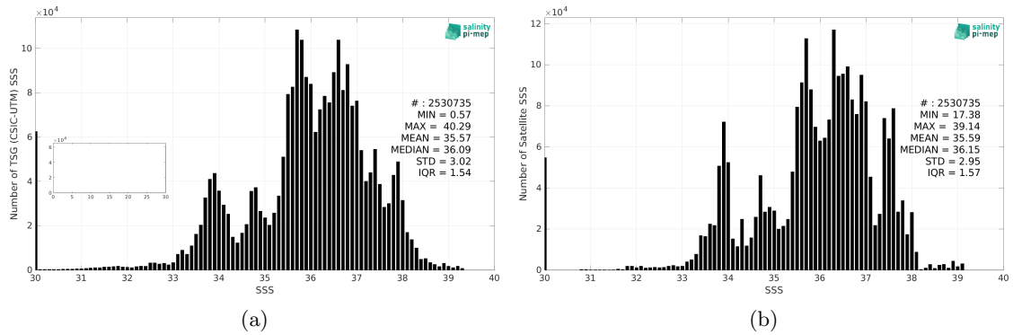
Figure 2: Histograms of SSS from TSG (CSIC-UTM) (a) and SMOS SSS L4 v1 - Monthly (CMEMS-CNR) (b) considering all match-up pairs per bins of 0.1 over the Global Ocean Pi-MEP region and for the full satellite product period.
