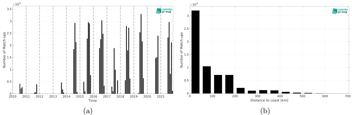
Figure 2: Number of match-ups between TSG (Amundsen) and SMOS SSS L4 v1 - Monthly (CMEMS-CNR) SSS as a function of time (a) and as function of the distance to coast (b) over the Global Ocean Pi-MEP region and for the full satellite product period.
