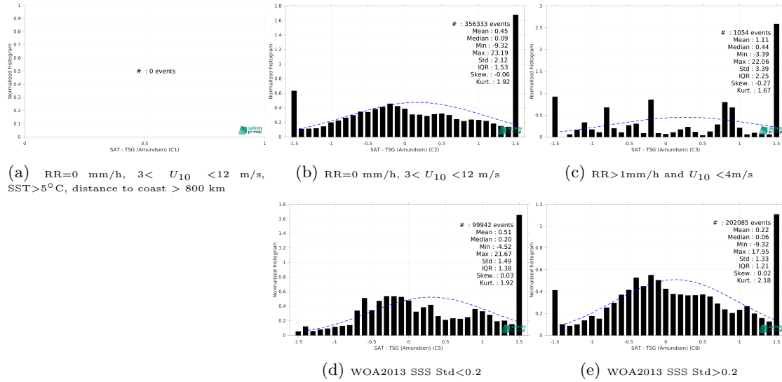
Figure 15: Normalized histogram of \Delta SSS (SMOS SSS L4 v1 - Monthly (CMEMS-CNR) - TSG (Amundsen)) for 5 different subdatasets corresponding to: RR=0 mm/h, 3 < U_{10} < 12 m/s, SST>5°C, distance to coast > 800 km (a), RR=0 mm/h, 3 < U_{10} < 12 m/s (b), RR>1mm/h and U_{10} < 4 m/s (c), WOA2013 SSS Std<0.2 (d), WOA2013 SSS Std>0.2 (e).
