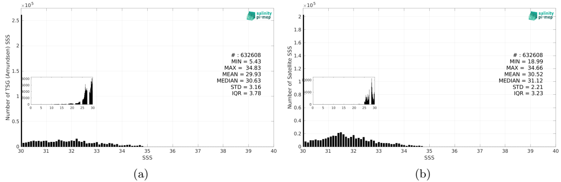
Figure 3: Histograms of SSS from TSG (Amundsen) (a) and SMOS SSS L4 v1 - Monthly (CMEMS-CNR) (b) considering all match-up pairs per bins of 0.1 over the Global Ocean Pi-MEP region and for the full satellite product period.
