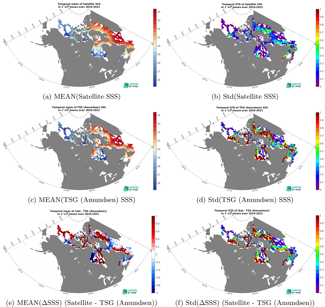
Figure 7: Temporal mean (left) and Std (right) of SSS from SMOS SSS L4 v1 - Monthly (CMEMS-CNR) (top), TSG (Amundsen) (middle), and of \Delta SSS (Satellite - TSG (Amundsen)). Only match-up pairs are used to generate these maps.
