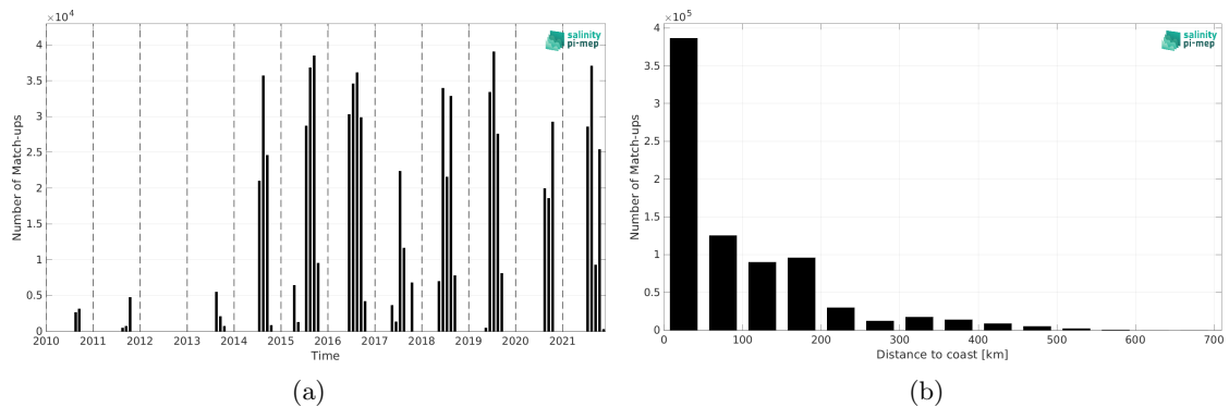
Figure 1: Number of match-ups between TSG (Amundsen) and SMOS SSS L4 v1 - Monthly (CMEMS-CNR) SSS as a function of time (a) and as function of the distance to coast (b) over the Global Ocean Pi-MEP region and for the full satellite product period.
