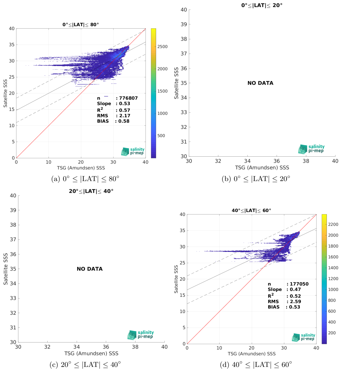
Figure 9: Contour maps of the concentration of SMOS SSS L4 v1 - Monthly (CMEMS-CNR) SSS (y-axis) versus TSG (Amundsen) SSS (x-axis) at match-up pairs for different latitude bands. For each plot, the red line shows x=y . The black thin and dashed lines indicate a linear fit through the data cloud and the \pm 95\% confidence levels, respectively. The number match-up pairs n , the slope and R^2 coefficient of the linear fit, the root mean square (RMS) and the mean bias between satellite and in situ data are indicated for each latitude band in each plots.
