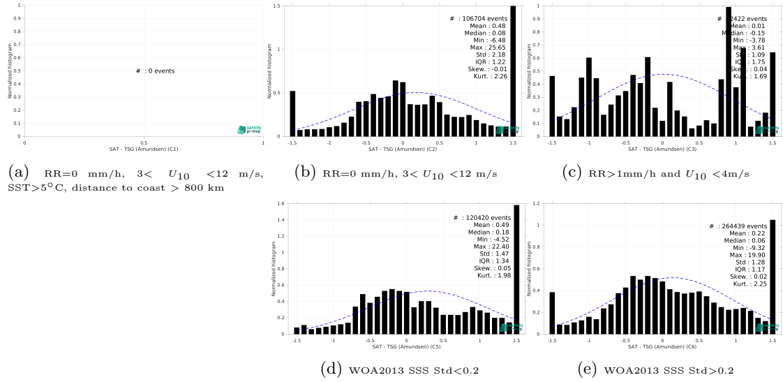
Figure 13: Normalized histogram of \Delta SSS (SMOS SSS L4 v1 - Monthly (CMEMS-CNR) - TSG (Amundsen)) for 5 different subdatasets corresponding to: RR=0 mm/h, 3 < U_{10} < 12 m/s, SST > 5°C, distance to coast > 800 km (a), RR=0 mm/h, 3 < U_{10} < 12 m/s (b), RR > 1mm/h and U_{10} < 4 m/s (c), WOA2013 SSS Std < 0.2 (d), WOA2013 SSS Std > 0.2 (e).
