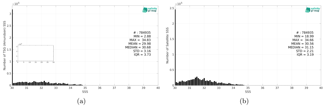
Figure 2: Histograms of SSS from TSG (Amundsen) (a) and SMOS SSS L4 v1 - Monthly (CMEMS-CNR) (b) considering all match-up pairs per bins of 0.1 over the Global Ocean Pi-MEP region and for the full satellite product period.
