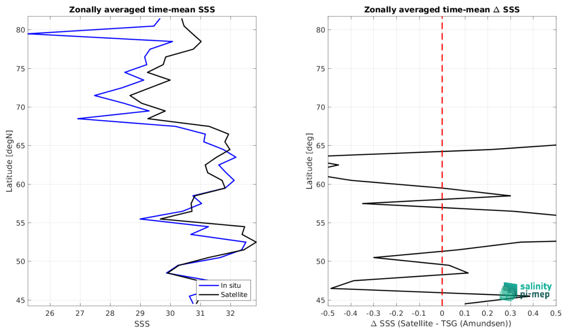
Figure 8: Left panel: Zonal mean SSS from SMOS SSS L4 v1 - Monthly (CMEMS-CNR) satellite product (black) and from TSG (Amundsen) (blue). Right panel: Zonal mean of \Delta SSS (Satellite - TSG (Amundsen)) for all the collected Pi-MEP match-up pairs estimated over the full satellite product period.
