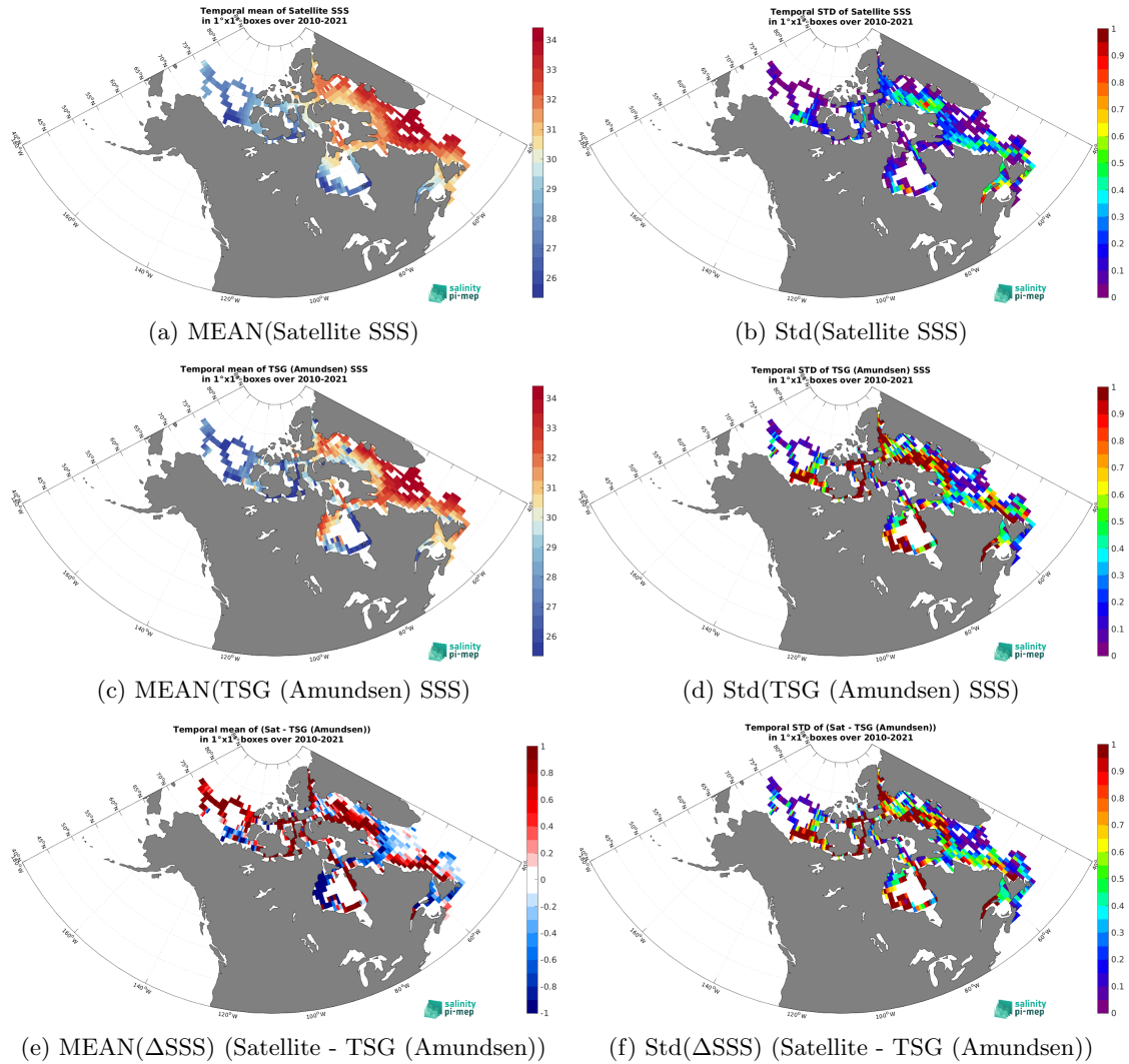
Figure 6: Temporal mean (left) and Std (right) of SSS from SMOS SSS L4 v1 - Monthly (CMEMS-CNR) (top), TSG (Amundsen) (middle), and of \Delta SSS (Satellite - TSG (Amundsen)). Only match-up pairs are used to generate these maps.
