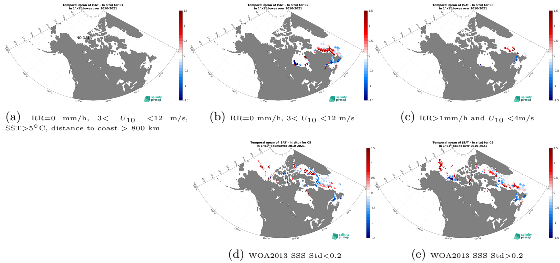
Figure 12: Temporal mean gridded over spatial boxes of size 1^{\circ}\times 1^{\circ} of \Delta\text{SSS} (SMOS SSS L4 v1 - Monthly (CMEMS-CNR) - TSG (Amundsen)) for 5 different subdatasets corresponding to:RR=0 mm/h, 3 < U_{10} < 12 m/s, SST > 5^{\circ}\text{C} , distance to coast > 800 km (a), RR=0 mm/h, 3 < U_{10} < 12 m/s (b), RR > 1 mm/h and U_{10} < 4 m/s (c), WOA2013 SSS Std < 0.2 (d), WOA2013 SSS Std > 0.2 (e).
