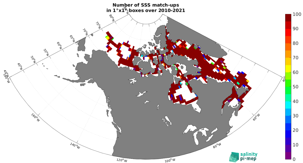
Figure 4: Number of SSS match-ups between TSG (Amundsen) SSS and the SMOS SSS L4 v1 - Monthly (CMEMS-CNR) SSS product for the Global Ocean Pi-MEP region over 1°×1° boxes and for the full satellite product period.
