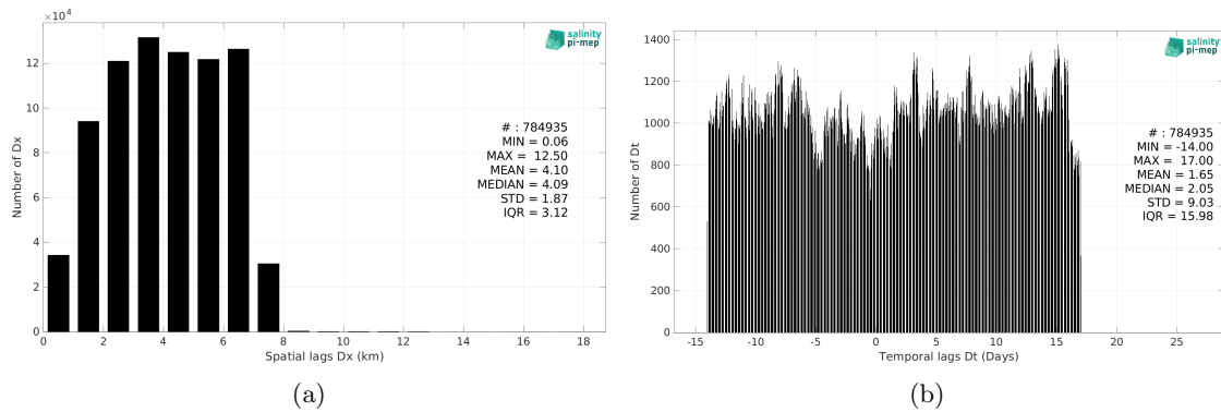
Figure 5: Histograms of the spatial (a) and temporal (b) lags between the location/time of the TSG (Amundsen) measurement and the date of the corresponding SMOS SSS L4 v1 - Monthly (CMEMS-CNR) SSS pixel.
