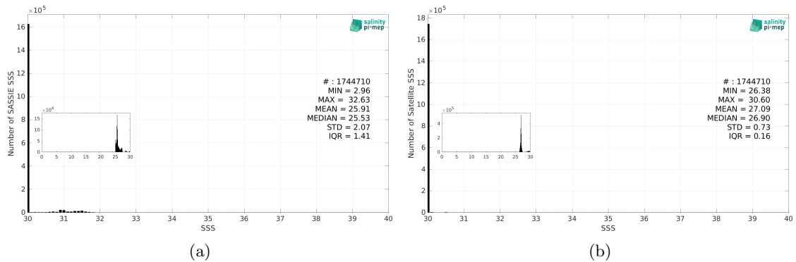
Figure 3: Histograms of SSS from SASSIE (a) and SMOS SSS L4 v1 - Monthly (CMEMS-CNR) (b) considering all match-up pairs per bins of 0.1 over the Global Ocean Pi-MEP region and for the full satellite product period.
