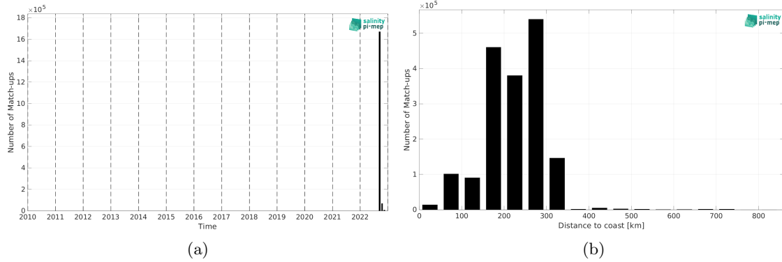
Figure 2: Number of match-ups between SASSIE and SMOS SSS L4 v1 - Monthly (CMEMS-CNR) SSS as a function of time (a) and as function of the distance to coast (b) over the Global Ocean Pi-MEP region and for the full satellite product period.
