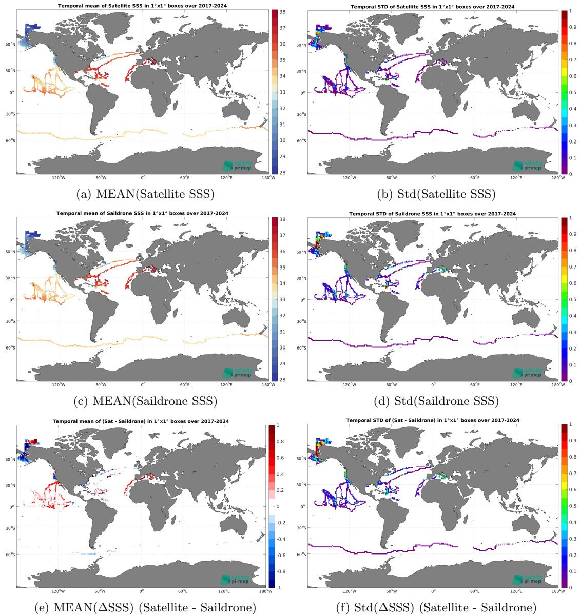
Figure 7: Temporal mean (left) and Std (right) of SSS from SMOS SSS L4 v1 - Monthly (CMEMS-CNR) (top), Saildrone (middle), and of \Delta SSS (Satellite - Saildrone). Only match-up pairs are used to generate these maps.
