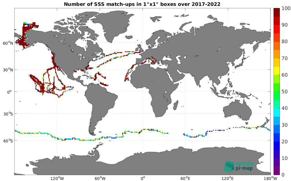
Figure 5: Number of SSS match-ups between Saildrone SSS and the SMOS SSS L4 v1 - Monthly (CMEMS-CNR) SSS product for the Global Ocean Pi-MEP region over 1^\circ \times 1^\circ boxes and for the full satellite product period.
