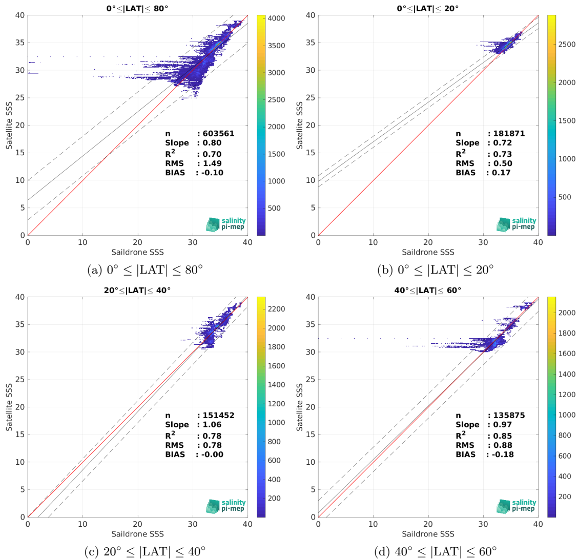
Figure 10: Contour maps of the concentration of SMOS SSS L4 v1 - Monthly (CMEMS-CNR) SSS (y-axis) versus Saildrone SSS (x-axis) at match-up pairs for different latitude bands. For each plot, the red line shows x=y . The black thin and dashed lines indicate a linear fit through the data cloud and the \pm 95\% confidence levels, respectively. The number match-up pairs n , the slope and R^2 coefficient of the linear fit, the root mean square (RMS) and the mean bias between satellite and in situ data are indicated for each latitude band in each plots.
