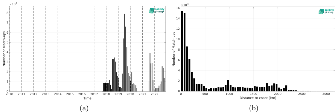
Figure 1: Number of match-ups between Saildrone and SMOS SSS L4 v1 - Monthly (CMEMS-CNR) SSS as a function of time (a) and as function of the distance to coast (b) over the Global Ocean Pi-MEP region and for the full satellite product period.
