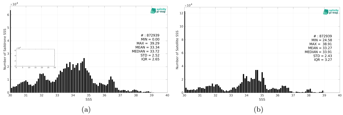
Figure 2: Histograms of SSS from Saildrone (a) and SMOS SSS L4 v1 - Monthly (CMEMS-CNR) (b) considering all match-up pairs per bins of 0.1 over the Global Ocean Pi-MEP region and for the full satellite product period.
