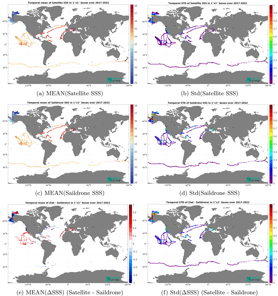
Figure 6: Temporal mean (left) and Std (right) of SSS from SMOS SSS L4 v1 - Monthly (CMEMS-CNR) (top), Saildrone (middle), and of \Delta SSS (Satellite - Saildrone). Only match-up pairs are used to generate these maps.
