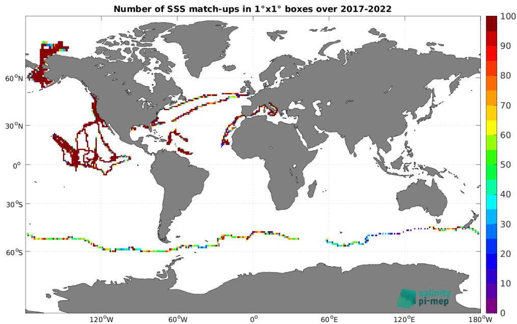
Figure 4: Number of SSS match-ups between Saildrone SSS and the SMOS SSS L4 v1 - Monthly (CMEMS-CNR) SSS product for the Global Ocean Pi-MEP region over 1^\circ \times 1^\circ boxes and for the full satellite product period.
