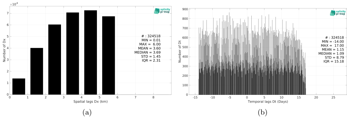
Figure 6: Histograms of the spatial (a) and temporal (b) lags between the location/time of the Marine mammals SSS measurement and the date of the corresponding SMOS SSS L4 v1 - Monthly (CMEMS-CNR) SSS pixel.
