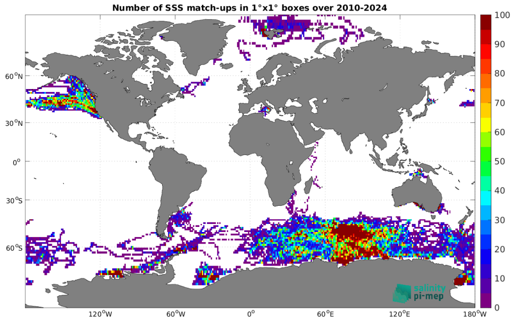
Figure 5: Number of SSS match-ups between Marine mammals SSS and the SMOS SSS L4 v1 - Monthly (CMEMS-CNR) SSS product for the Global Ocean Pi-MEP region over 1^{\circ} \times 1^{\circ} boxes and for the full satellite product period.
