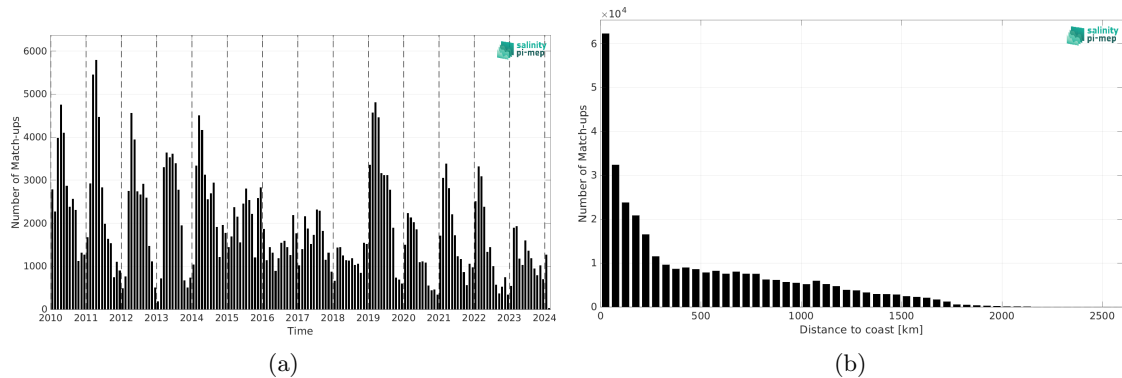
Figure 2: Number of match-ups between Marine mammals and SMOS SSS L4 v1 - Monthly (CMEMS-CNR) SSS as a function of time (a) and as function of the distance to coast (b) over the Global Ocean Pi-MEP region and for the full satellite product period.
