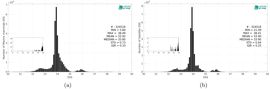
Figure 3: Histograms of SSS from Marine mammals (a) and SMOS SSS L4 v1 - Monthly (CMEMS-CNR) (b) considering all match-up pairs per bins of 0.1 over the Global Ocean Pi-MEP region and for the full satellite product period.
