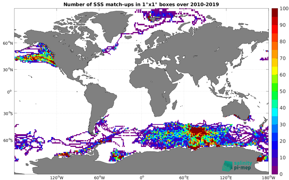
Figure 4: Number of SSS match-ups between Marine mammals SSS and the SMOS SSS L4 v1 - Monthly (CMEMS-CNR) SSS product for the Global Ocean Pi-MEP region over 1°x1° boxes and for the full satellite product period.
