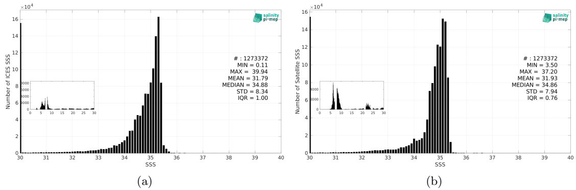
Figure 3: Histograms of SSS from ICES (a) and SMOS SSS L4 v1 - Monthly (CMEMS-CNR) (b) considering all match-up pairs per bins of 0.1 over the Global Ocean Pi-MEP region and for the full satellite product period.
