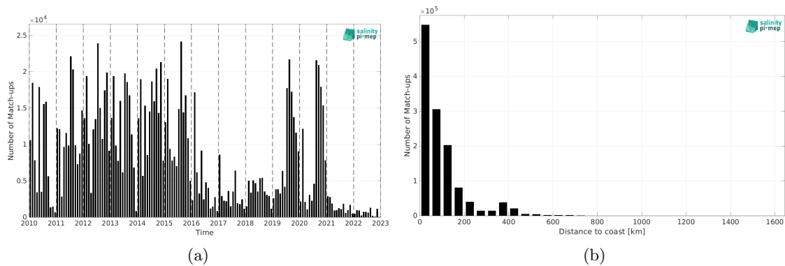
Figure 2: Number of match-ups between ICES and SMOS SSS L4 v1 - Monthly (CMEMS-CNR) SSS as a function of time (a) and as function of the distance to coast (b) over the Global Ocean Pi-MEP region and for the full satellite product period.
