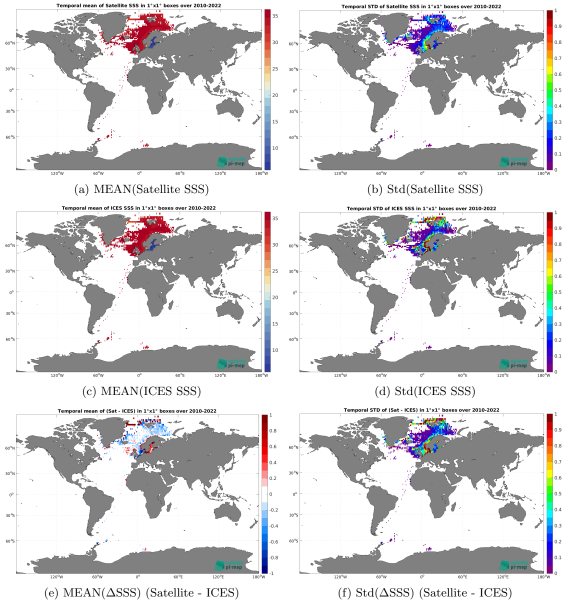
Figure 7: Temporal mean (left) and Std (right) of SSS from SMOS SSS L4 v1 - Monthly (CMEMS-CNR) (top), ICES (middle), and of \Delta SSS (Satellite - ICES). Only match-up pairs are used to generate these maps.
