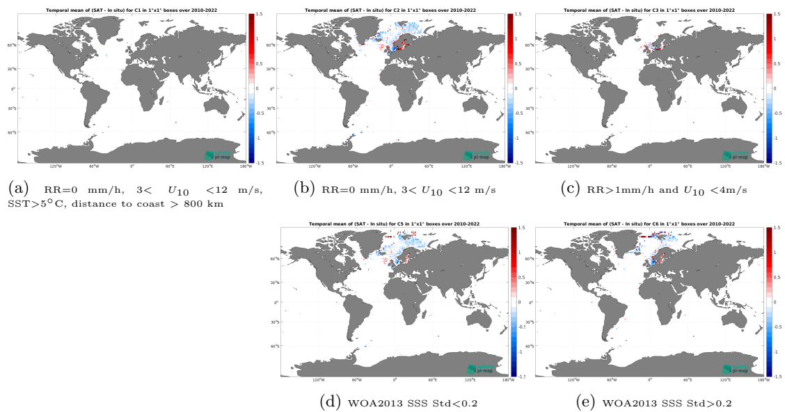
Figure 14: Temporal mean gridded over spatial boxes of size 1^\circ \times 1^\circ of \Delta SSS (SMOS SSS L4 v1 - Monthly (CMEMS-CNR) - ICES) for 5 different subdatasets corresponding to:RR=0 mm/h, 3 < U_{10} < 12 m/s, SST > 5^\circ\text{C} , distance to coast > 800 km (a), RR=0 mm/h, 3 < U_{10} < 12 m/s (b), RR > 1 mm/h and U_{10} < 4 m/s (c), WOA2013 SSS Std < 0.2 (d), WOA2013 SSS Std > 0.2 (e).
