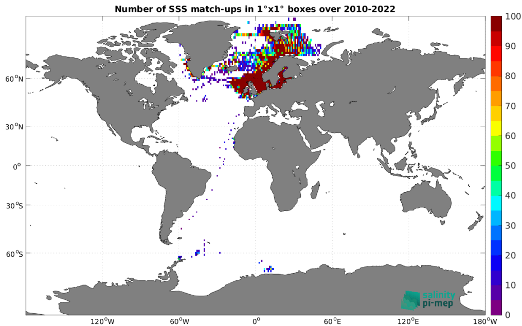
Figure 5: Number of SSS match-ups between ICES SSS and the SMOS SSS L4 v1 - Monthly (CMEMS-CNR) SSS product for the Global Ocean Pi-MEP region over 1^\circ \times 1^\circ boxes and for the full satellite product period.
