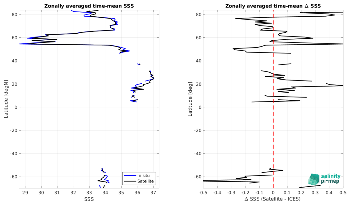
Figure 8: Left panel: Zonal mean SSS from SMOS SSS L4 v1 - Monthly (CMEMS-CNR) satellite product (black) and from ICES (blue). Right panel: Zonal mean of \Delta SSS (Satellite - ICES) for all the collected Pi-MEP match-up pairs estimated over the full satellite product period.
