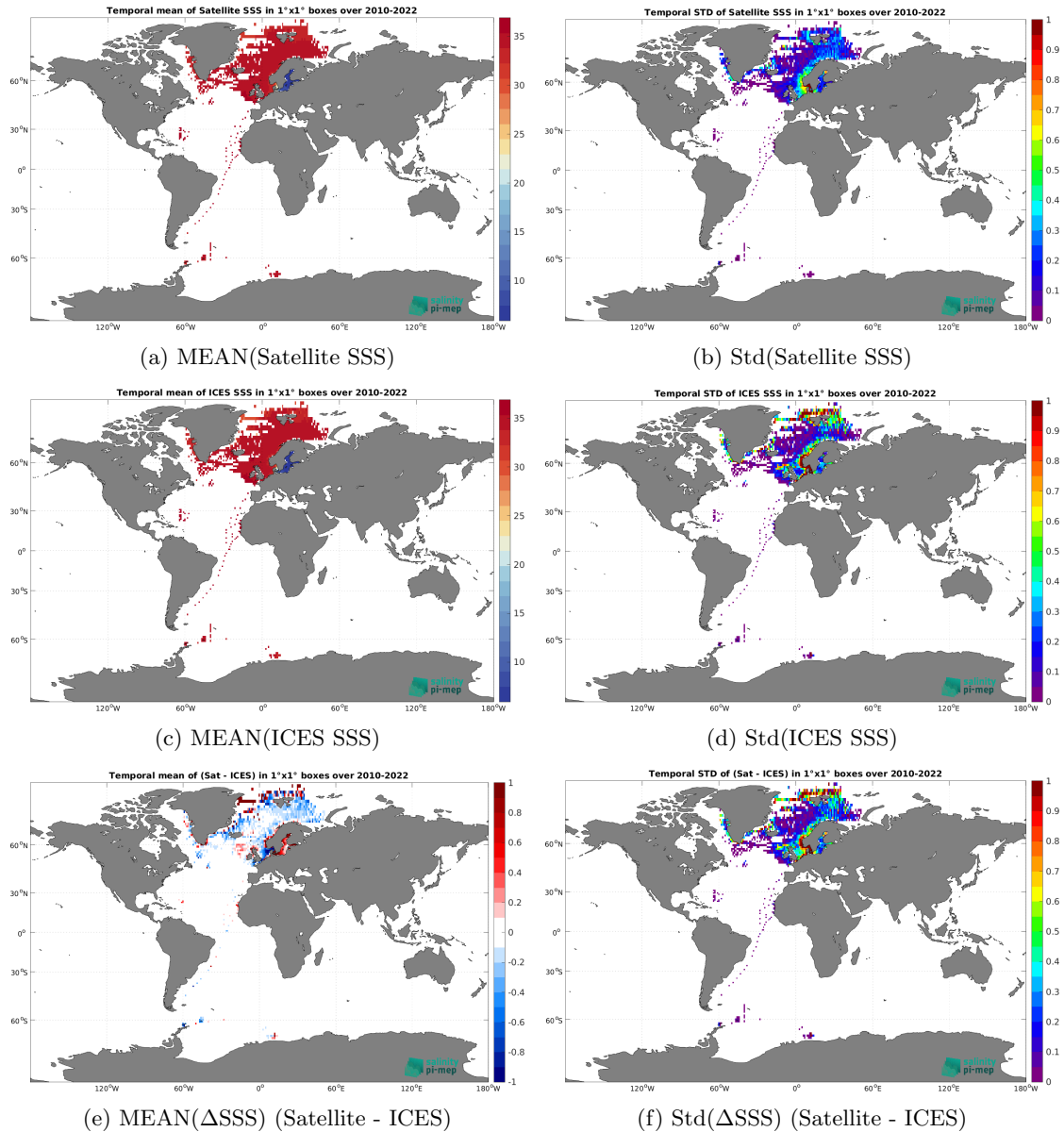
Figure 6: Temporal mean (left) and Std (right) of SSS from SMOS SSS L4 v1 - Monthly (CMEMS-CNR) (top), ICES (middle), and of \Delta SSS (Satellite - ICES). Only match-up pairs are used to generate these maps.
