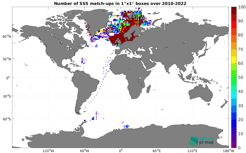
Figure 4: Number of SSS match-ups between ICES SSS and the SMOS SSS L4 v1 - Monthly (CMEMS-CNR) SSS product for the Global Ocean Pi-MEP region over 1^\circ \times 1^\circ boxes and for the full satellite product period.
