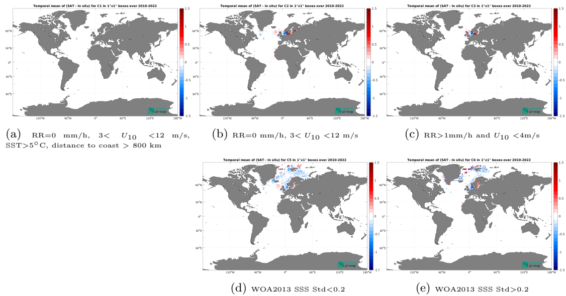
Figure 12: Temporal mean gridded over spatial boxes of size 1^\circ \times 1^\circ of \Delta SSS (SMOS SSS L4 v1 - Monthly (CMEMS-CNR) - ICES) for 5 different subdatasets corresponding to:RR=0 mm/h, 3 < U_{10} < 12 m/s, SST >5^\circ C, distance to coast > 800 km (a), RR=0 mm/h, 3 < U_{10} < 12 m/s (b), RR >1 mm/h and U_{10} < 4 m/s (c), WOA2013 SSS Std <0.2 (d), WOA2013 SSS Std >0.2 (e).
