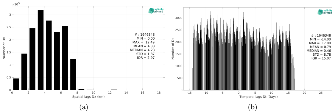
Figure 5: Histograms of the spatial (a) and temporal (b) lags between the location/time of the ICES measurement and the date of the corresponding SMOS SSS L4 v1 - Monthly (CMEMS-CNR) SSS pixel.
