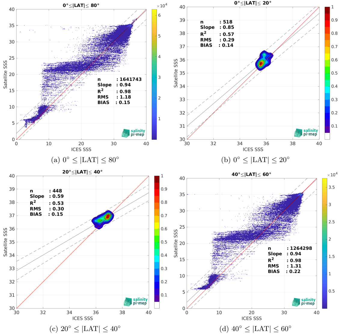
Figure 9: Contour maps of the concentration of SMOS SSS L4 v1 - Monthly (CMEMS-CNR) SSS (y-axis) versus ICES SSS (x-axis) at match-up pairs for different latitude bands. For each plot, the red line shows x=y . The black thin and dashed lines indicate a linear fit through the data cloud and the \pm 95\% confidence levels, respectively. The number match-up pairs n , the slope and R^2 coefficient of the linear fit, the root mean square (RMS) and the mean bias between satellite and in situ data are indicated for each latitude band in each plots.
