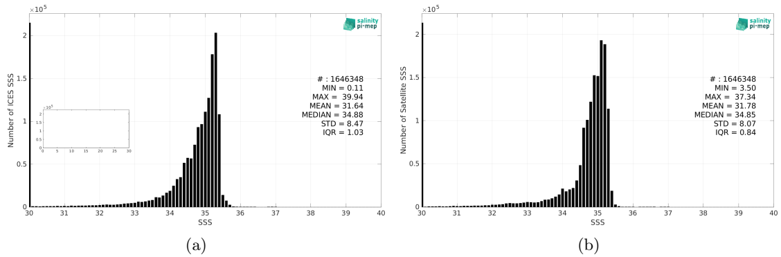
Figure 2: Histograms of SSS from ICES (a) and SMOS SSS L4 v1 - Monthly (CMEMS-CNR) (b) considering all match-up pairs per bins of 0.1 over the Global Ocean Pi-MEP region and for the full satellite product period.
