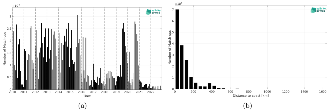
Figure 1: Number of match-ups between ICES and SMOS SSS L4 v1 - Monthly (CMEMS-CNR) SSS as a function of time (a) and as function of the distance to coast (b) over the Global Ocean Pi-MEP region and for the full satellite product period.
