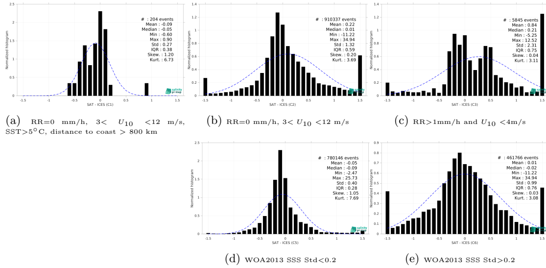
Figure 13: Normalized histogram of \Delta SSS (SMOS SSS L4 v1 - Monthly (CMEMS-CNR) - ICES) for 5 different subdatasets corresponding to: RR=0 mm/h, 3 < U_{10} < 12 m/s, SST > 5°C, distance to coast > 800 km (a), RR=0 mm/h, 3 < U_{10} < 12 m/s (b), RR > 1mm/h and U_{10} < 4 m/s (c), WOA2013 SSS Std < 0.2 (d), WOA2013 SSS Std > 0.2 (e).
